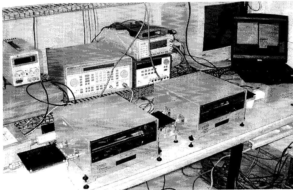
Figure 8.2 DLPS Practical Setup
