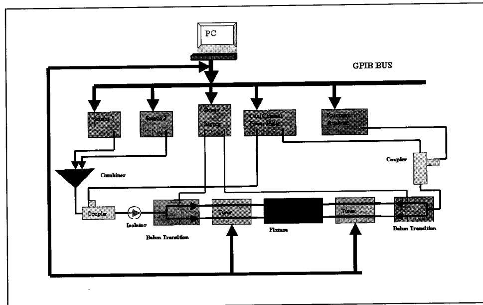
Figure 8.1 DLP Configurations
