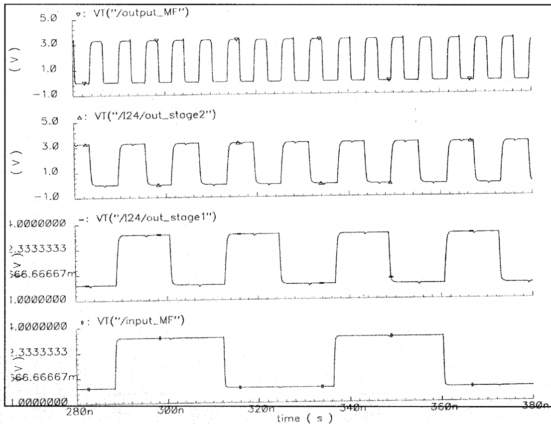
Figure 6.2: The Simulation Results of ICDPMLIU Chip
