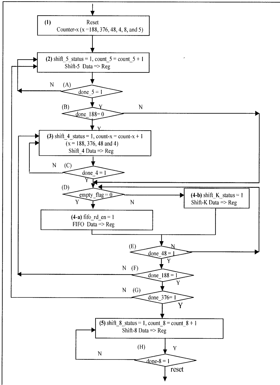
Figure 3.4: Flowchart for the Read Data Controls of the FSM
