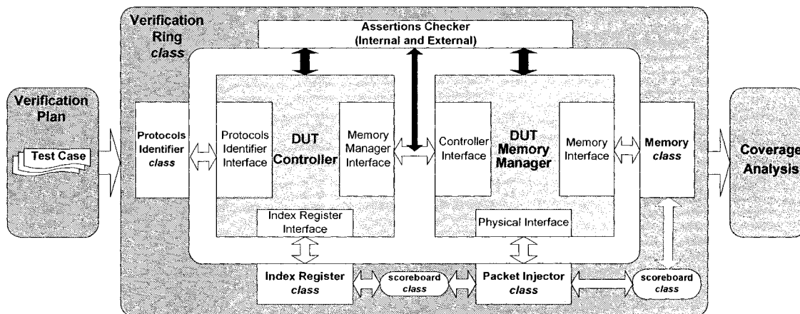
Figure 6. Reusability Realization
