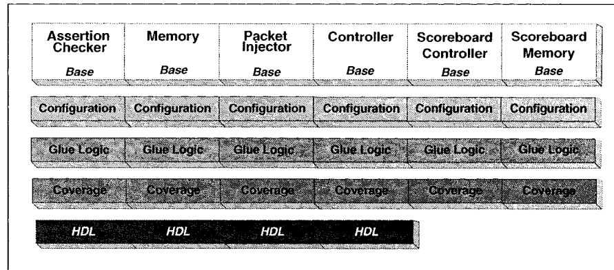
Figure 5 - Aspect Partitioning
