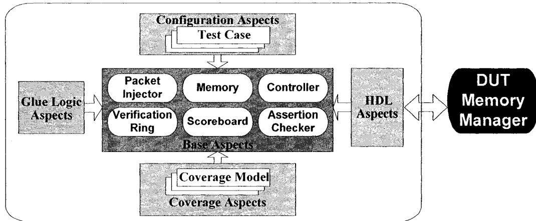
Figure 4. Aspects framework
