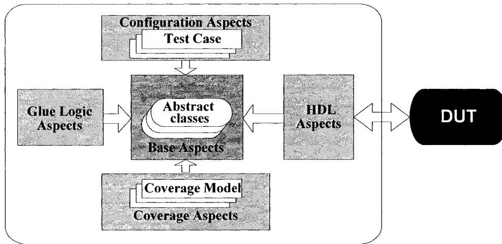
Figure 1. Aspect categories
