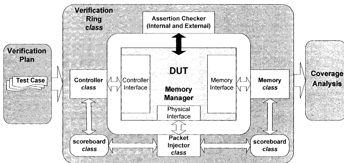
Figure 3. Verification Environment Functional View
