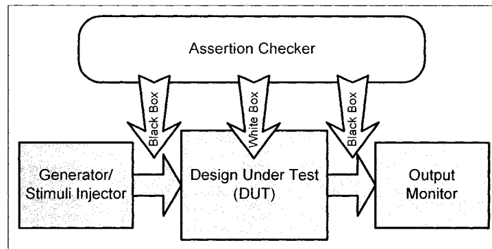
Figure 4.1 - Assertion Checker Functional View
