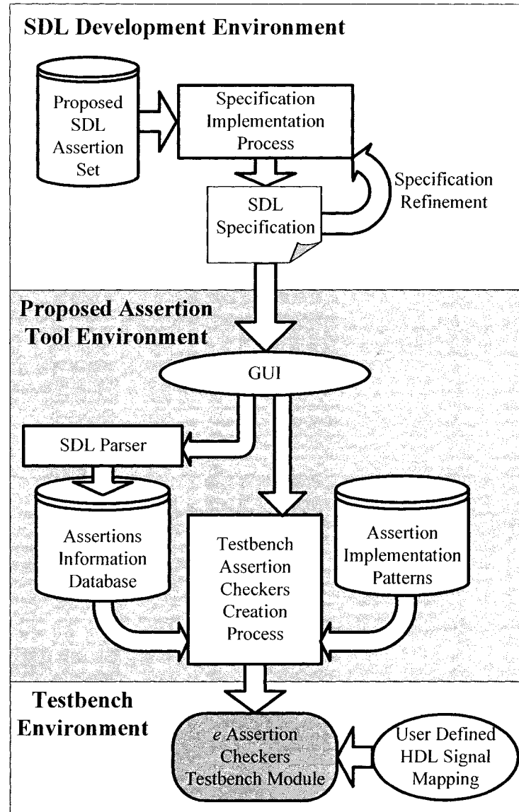
Figure 4.4 - Assertion Tool Overview
