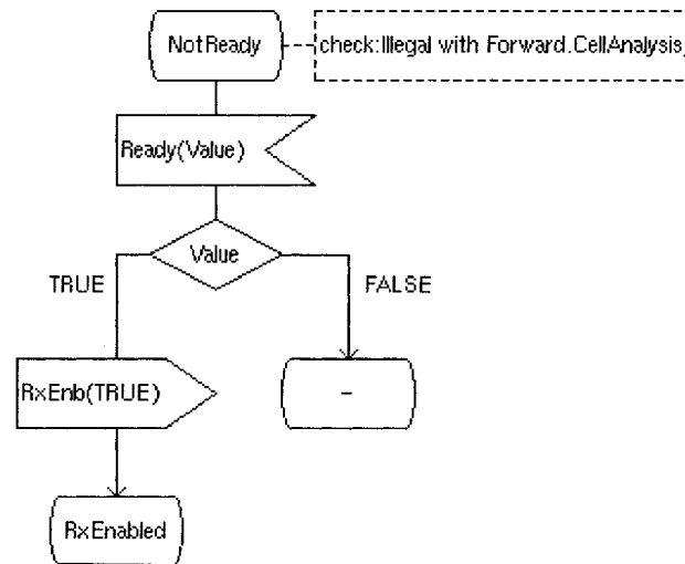
Figure 4.6 - State Assertion Example
