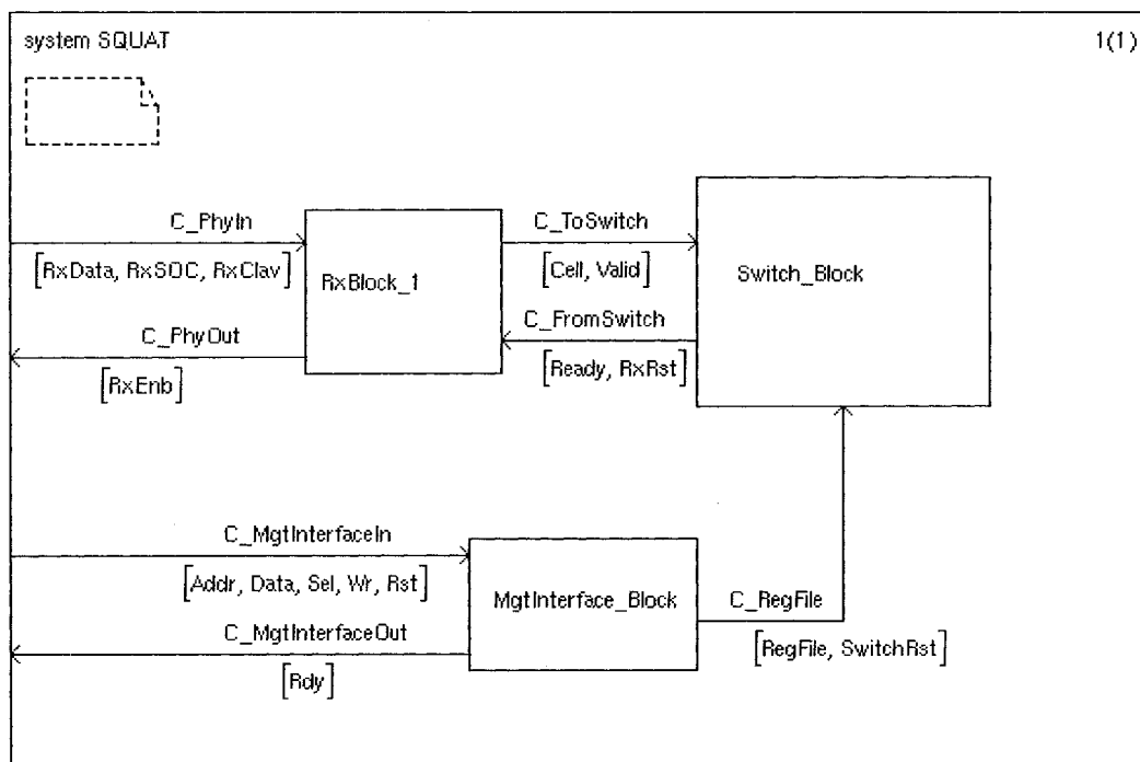
Figure 4.5 - ATM Switch SDL System Example
