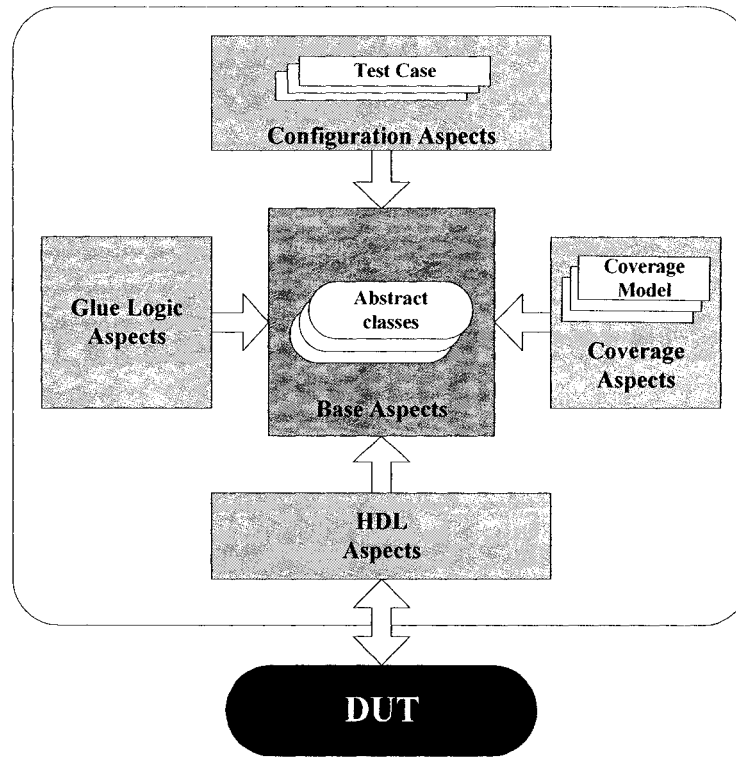
Figure 1 - Aspects of a verification environment
