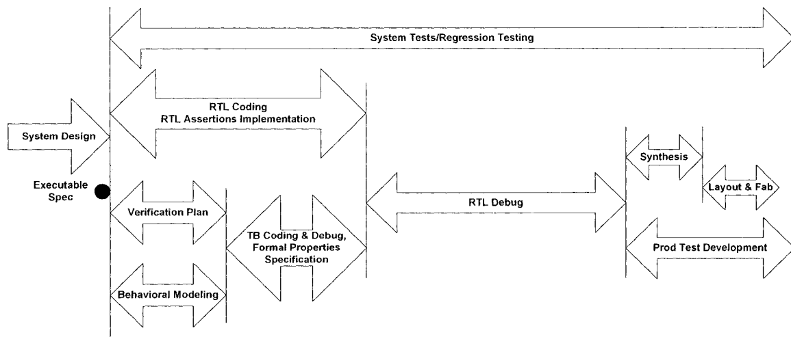
Figure 2.1 - Proposed Development Flow
