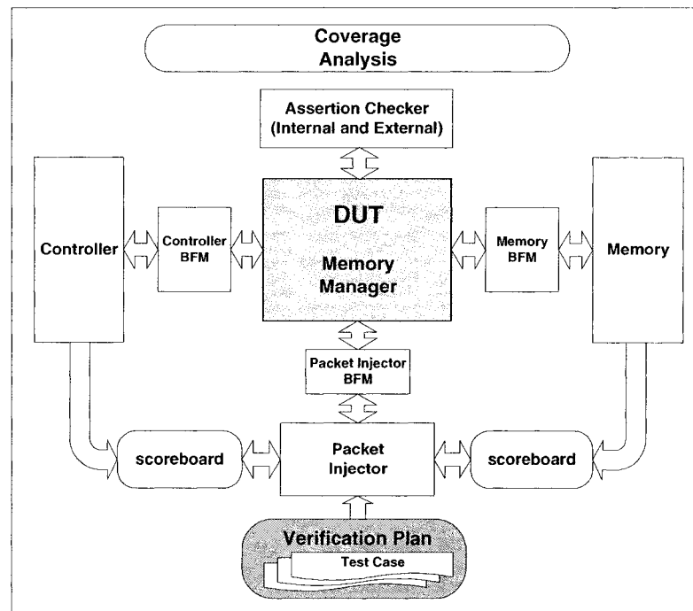
Figure 3 - Verification Environment (Functional View)
