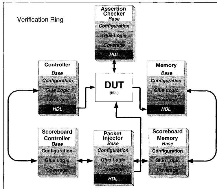
Figure 4 - Verification Environment (Aspect View)
