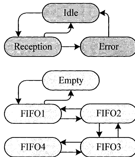
Figure 7 - State Machine
