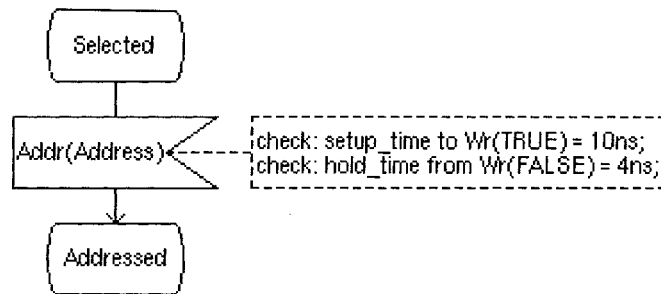
Figure 4.7 - Timing Assertions Example
