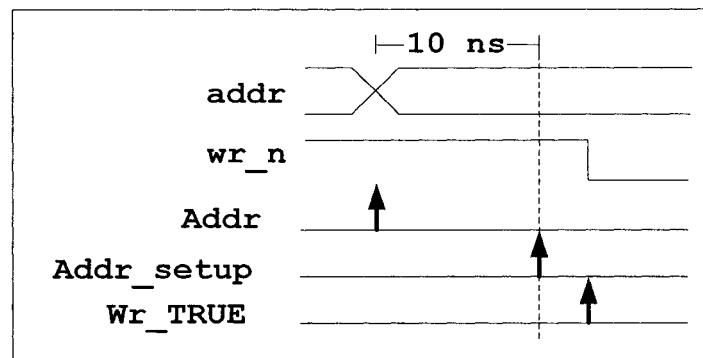
Figure 4.11 - Address Setup-Time Assertion Timing Diagram
