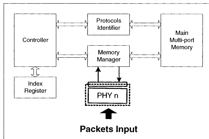
Figure 2 - Part of the protocol converter
