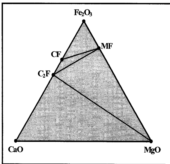
Figure 32: The CaO-MgO- \text{Fe}_2\text{O}_3 phase diagram.
