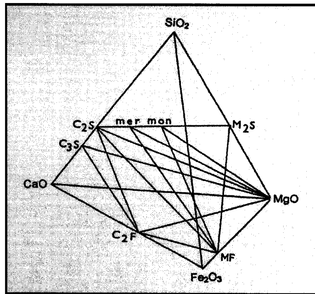
Figure 33: The \text{SiO}_2 – CaO – MgO – \text{Fe}_2\text{O}_3 system.
