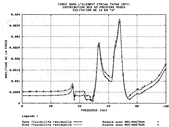
Figure III.36 : Élément CTRIA6 75760 (MFX)
