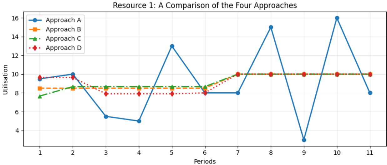
FIGURE 6.3 Comparison of four approaches for Resource 1 of instance 40-3-2-3 in terms of workload utilization across periods
