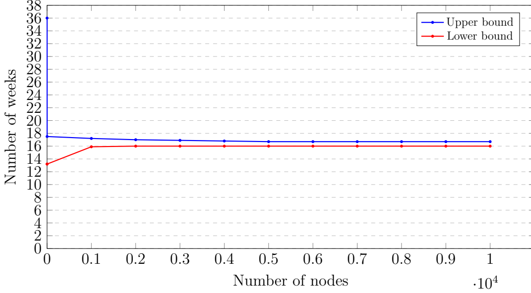
FIGURE 4.6 Curves illustrating the largest absolute optimality gap found
