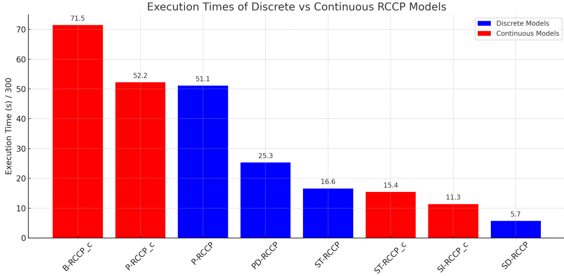
FIGURE 5.3 Execution time comparison between discrete RCCP models (in blue) and continuous RCCP models (in red)
