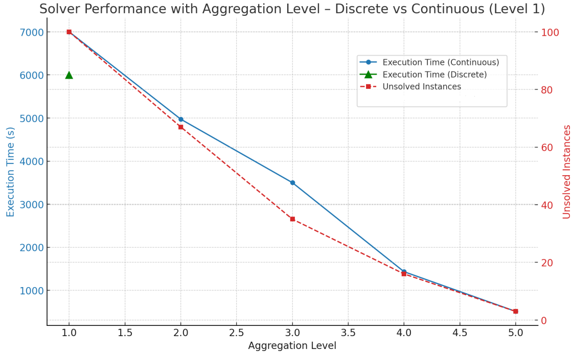
FIGURE 5.5 Solver performance with aggregated level : continuous vs discrete formulations
