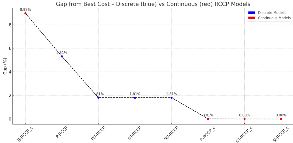
FIGURE 5.4 Gap from the best cost : Continuous vs. Discrete RCCP formulations
