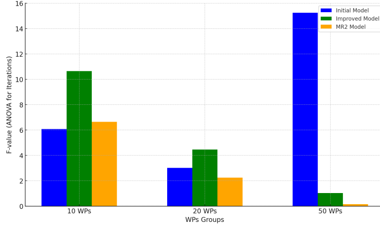
FIGURE 4.8 ANOVA F-values for number of iterations across models : Resource-driven variant
