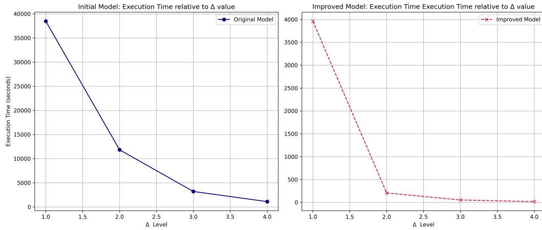
FIGURE 4.3 Impact of \Delta value over execution time : Initial model vs Improved model
