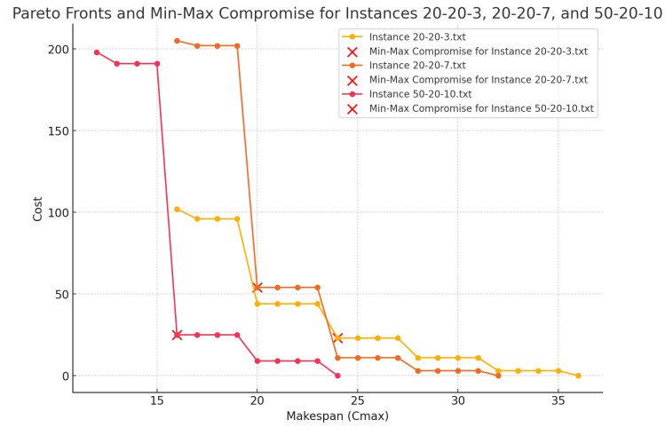
FIGURE 4.9 Pareto front for instances with a fairly good number of non-dominated points
