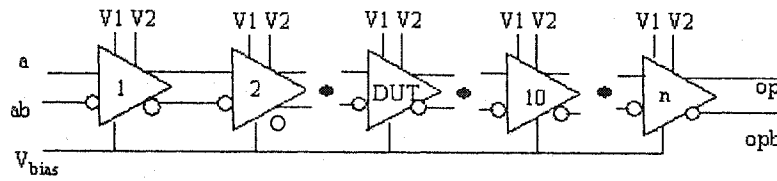
Figure 3.2 BUFFER test bench employed for ITT
