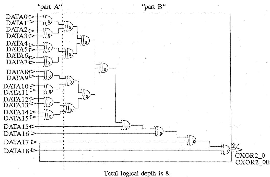
Figure 5.4 XOR half tree
