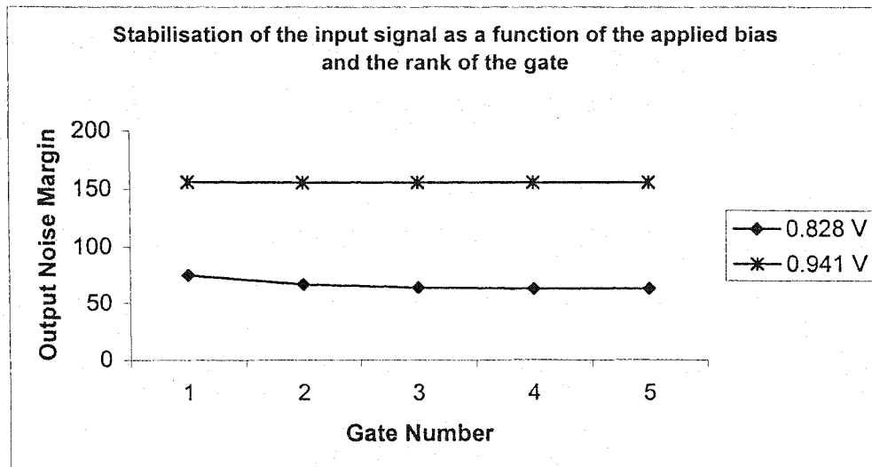
Figure 2.5 Stabilisation of the input signal as a function of the applied bias for grade 0 BUFFERS
