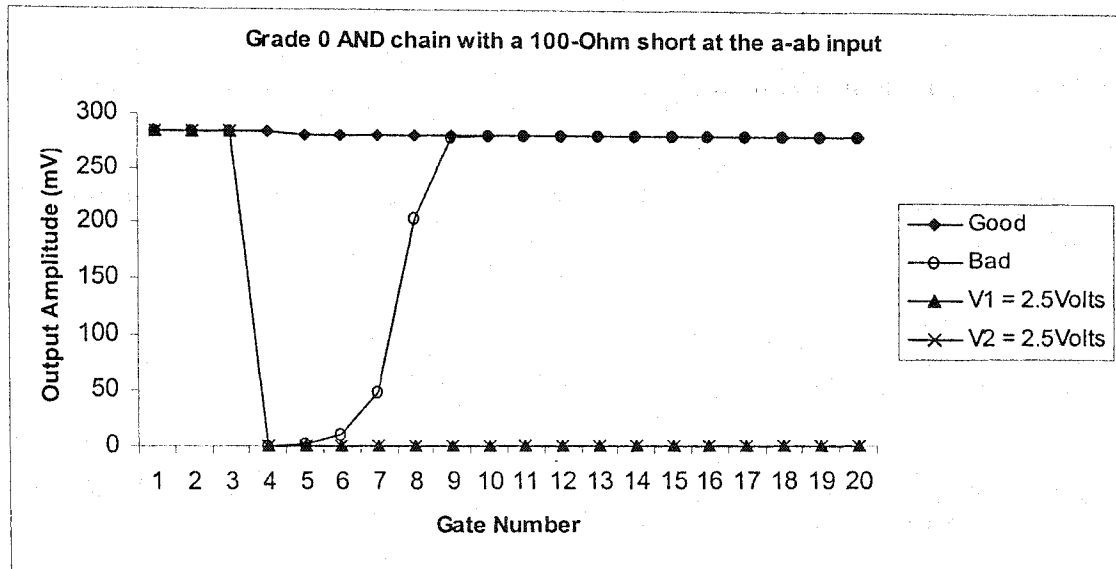
Figure 3.3 Output of a defective chain with & without ITT
