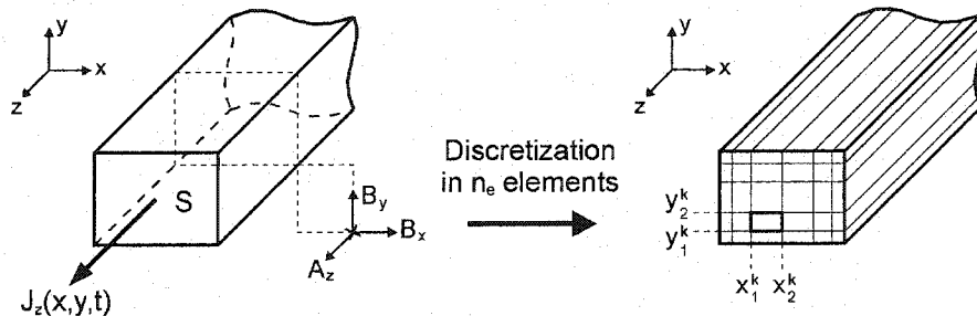
FIG. 5.1 – Left : typical 2D conductor geometry considered in this paper. The conductor cross-section S lies in the x - y plane, and the current density exists along the z axis only. The conductor's shape is not restricted to rectangles, but any shape that can be made by superposing rectangular elements. Also shown are the existing components of flux density and magnetic vector potential. Right : decomposition of the conductor in n_e rectangular elements. Elements of different sizes are allowed by the method formulation. The superscript k is used to identify the element number.
