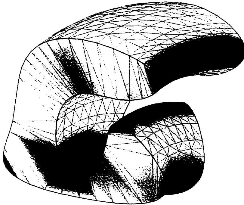
Figure 3.6: Graph of the curvatures obtained on the triangles by linear interpolation of the curvatures corresponding to the vertices. The most curved areas are shown in black
