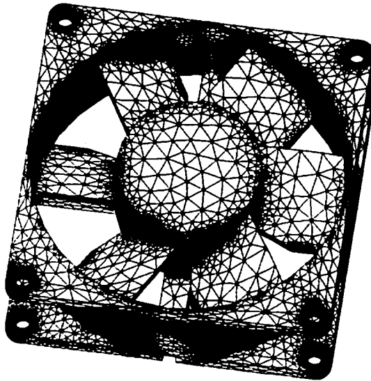
Figure 3.38: Adaptive refinement: maximum imposed geometric error: 0.01 mm, maximum imposed triangle size: 10 mm for low curvature regions. Smoothing. 75696 triangles, 37826 vertices.
