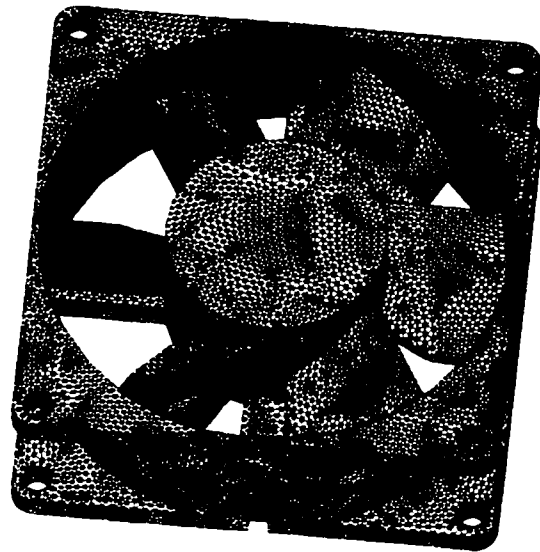
Figure 3.35: Refinement: constant target size: 2mm. Smoothing. 59196 triangles, 29576 vertices
