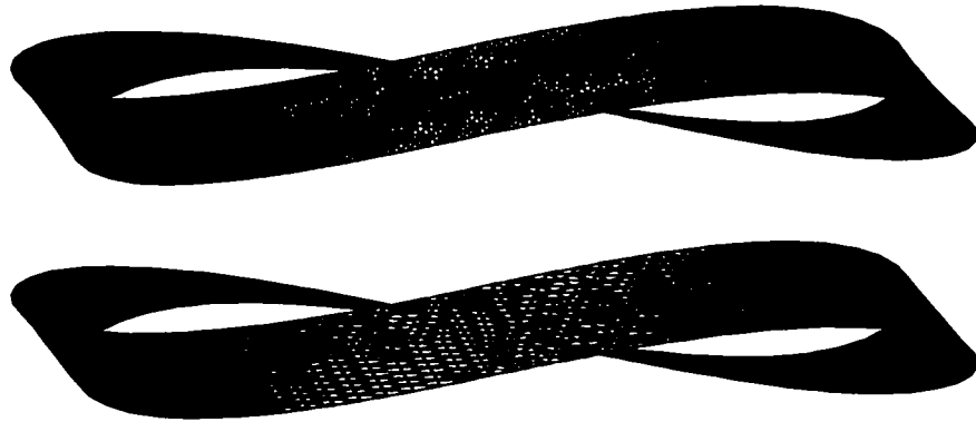
Figure 6.2: A Moebius band with an isotropic mesh (top) and an anisotropic mesh (bottom)
