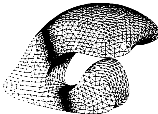
Figure 3.33: Refinement: constant target size: 8 mm , except on a plane: 2 mm. Smoothing. 8622 triangles, 4313 vertices.
