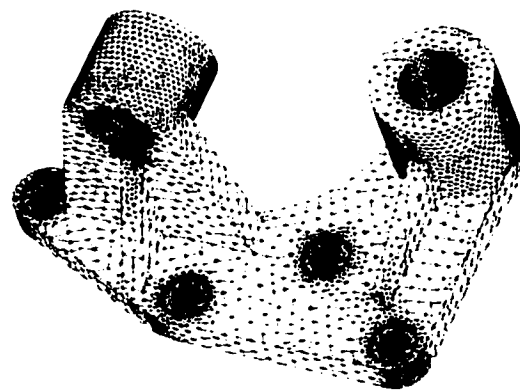
Figure 3.52: Adaptive refinement: maximum imposed geometric error: 0.05 mm, maximum imposed triangle size: 13 mm for low curvature regions. Smoothing. 26432 triangles, 13206 vertices
