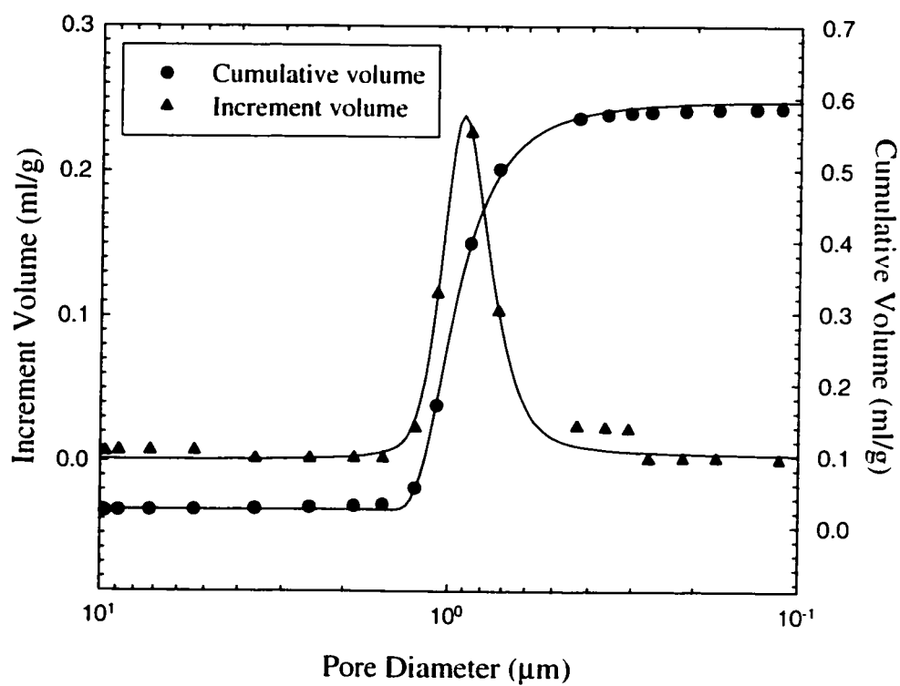
Figure 4.5. Pore size distribution of the extracted compatibilized blend (50HDPE/50PS/20SEBS) measured by mercury porosimetry.
