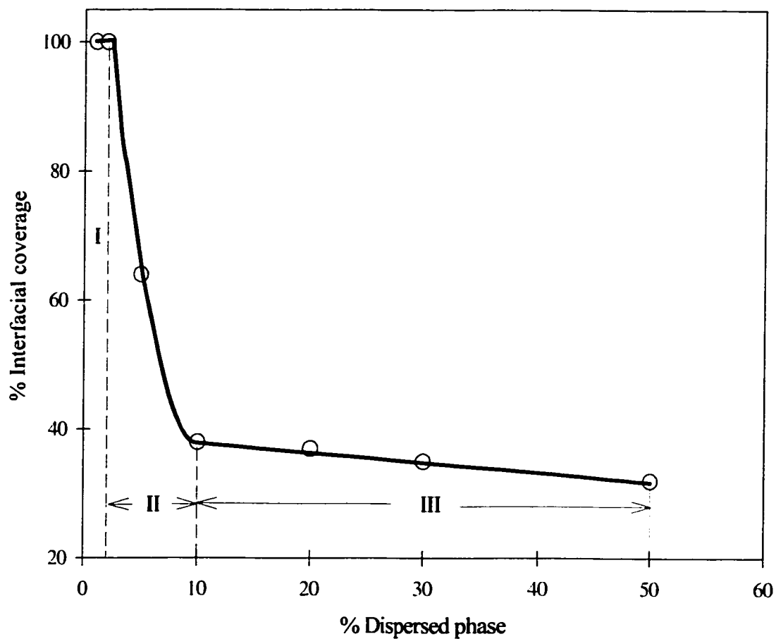
Figure 6.7. Interfacial coverage versus the dispersed phase concentration for PS dispersed in HDPE with SEBS1 as the interfacial modifier. Three distinct regions are observed in this system. Region I) all of the copolymer goes to the interface; region II) onset of micelle formation in the system; and region III) a quasi equilibrium between micelle formation and a partially saturated interface.
