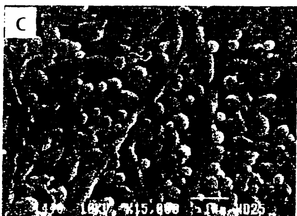
Figure 5.18 SEM photomicrographs of the dispersed HDPE phase and the corresponding TFR data after the matrix dissolution technique for a Type III system: (a) 5 HDPE/95 PS/20 SEBS1; (b) 10 HDPE/90 PS/20 SEBS1; and (c) 20 HDPE/80 PS/20 SEBS1.
