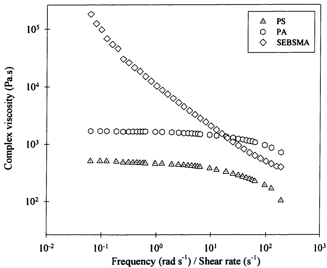
Figure 1. Complex viscosity-frequency/shear rate relationship for PA, PS and SEBS-g-MA at 250°C
