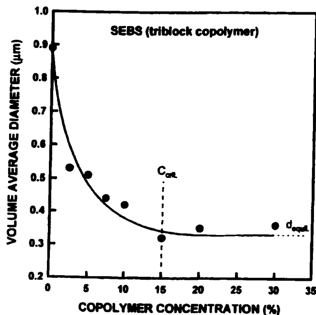
Figure 2.6 Emulsification curve for a 10%EPR/90%PS blend compatibilized by an SEBS triblock modifier of molecular weight 70K (Matos et al., 1995)
