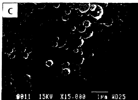
Figure 17 SEM photomicrographs of the dispersed HDPE phase after the matrix dissolution technique: (a) 5 HDPE/95 SEBS I (Type I); (b) 5 HDPE/95 PS (Type II); and (c) 5 HDPE/95 PS/20 SEBS I (Type III).
