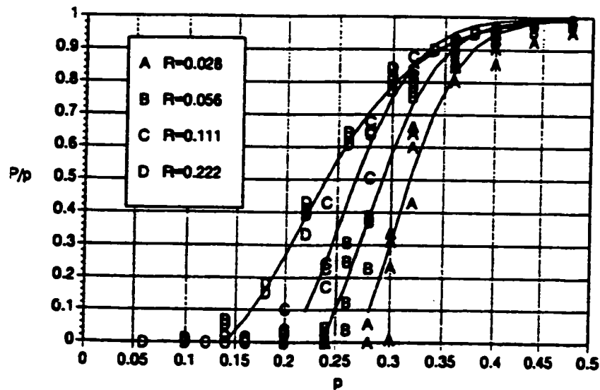
Figure 2.5 Effect of finite size on percolation : R is the ratio of inclusion to domain size in the percolation direction (Arends, 1992)
