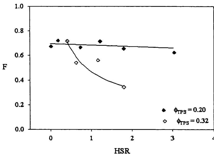
Figure 6.2. Form factor ( F ) vs. HSR of LDPE/TPS blends prepared in a one-step process at 150^{\circ}\text{C} .
