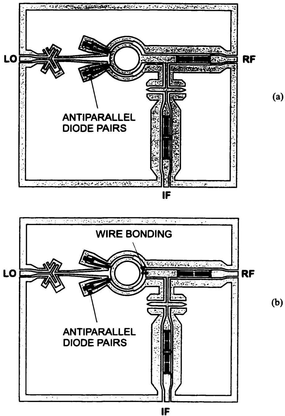
Figure 6.8 Two different balanced SH mixers with finite width ground plane: (a) without wire connection and (b) with a wire connection.
