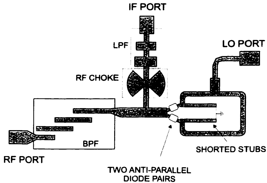
Figure 2.7 A circuit schematic for the balanced SH mixer.
