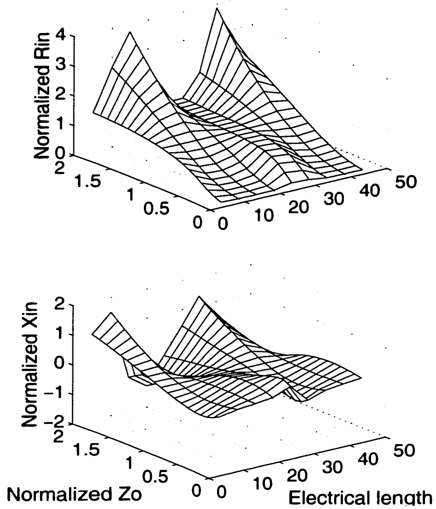
Figure 3.3 Input normalized impedance vs. \beta l and \tilde{Z}_0 .
