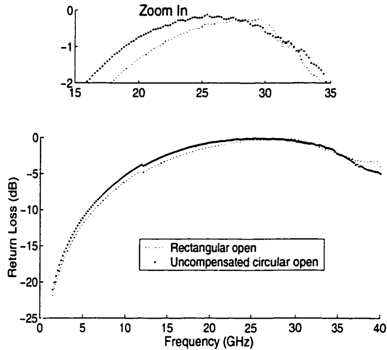
Figure 4.4 Measured results of both the rectangular-open RF choke and the circular-open RF choke without taping the central conductor shape. Geometrical dimensions are S_1 = 1.3 mil, W=3 mil, L_1 = 45.7 mil, W_1 = 12 mil, W_2 = 17 mil, L_2 = 50.7 mil, R_3 = 6 mil and thickness of alumina is equal to 10 mil.
