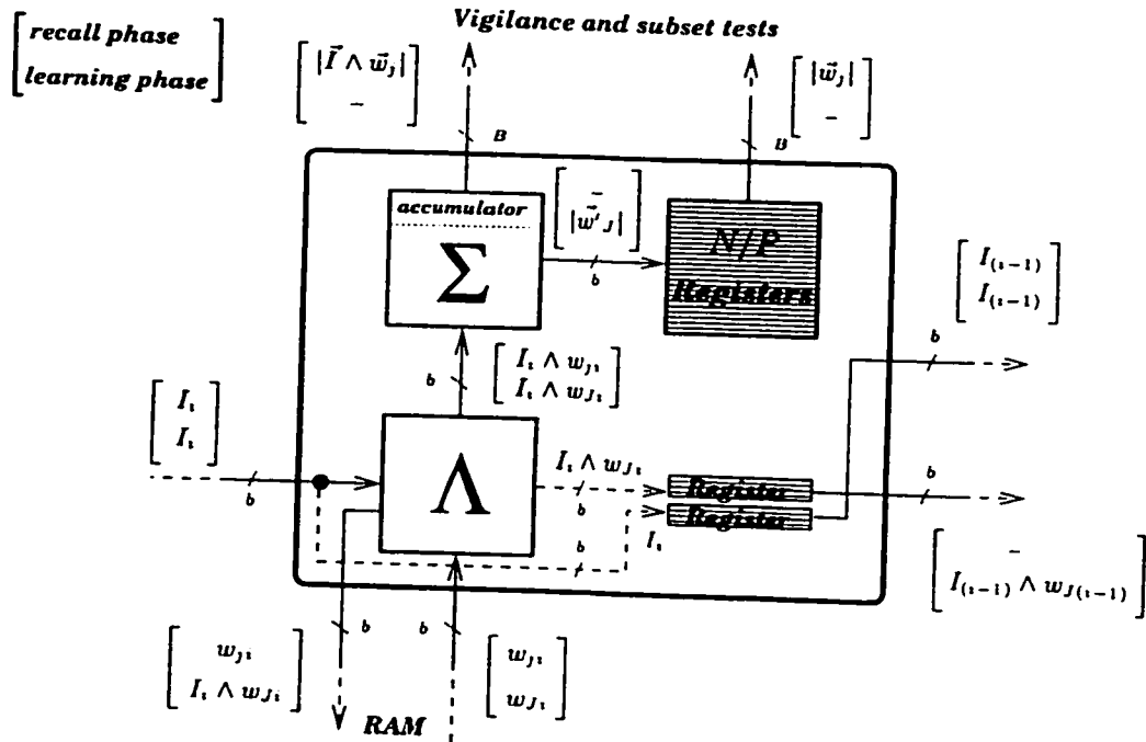
Figure 3.6: The basic structure of a NP module consists of a “min” comparator ( \Lambda ), an adder-accumulator ( \Sigma ), and registers to compute the values |\bar{I} \wedge \bar{w}_j| , w'_j and |\bar{w}'_j| . Note the dual labels for recall (top) and learning (bottom) phases respectively.
