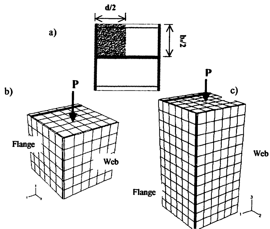
Fig. 4 Finite element models of the column: (a) Quarter cross section; (b) Specimen with s = d/2 ; and (c) Specimen with s = d .
