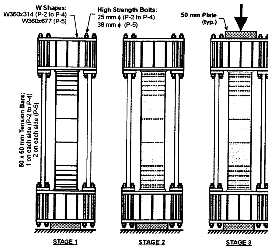
Figure 3.2. Loading Stages 1 to 3 for Specimens P-2 to P-5
