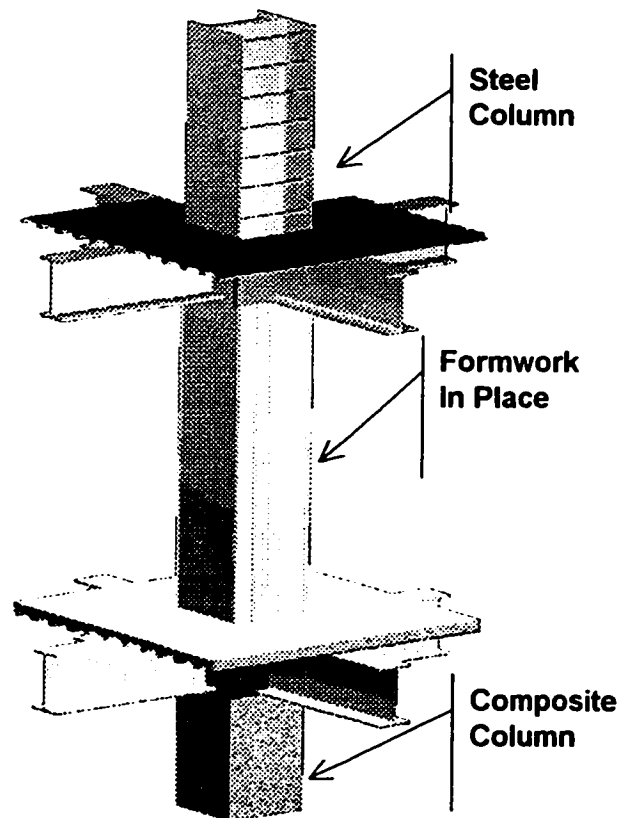
Figure 1.2 Construction Stages for Partially Encased Composite Column
