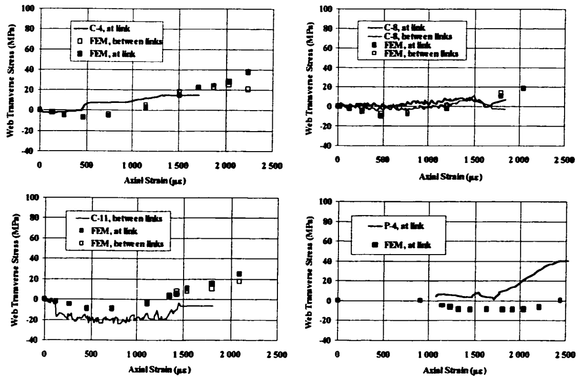
Fig. 11 Transverse stresses in the steel web of specimens and FE models
