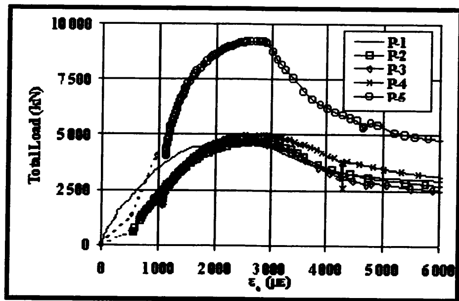
FIG. 12. Axial Load-Deformation Response of Specimens P-1 to P-5
