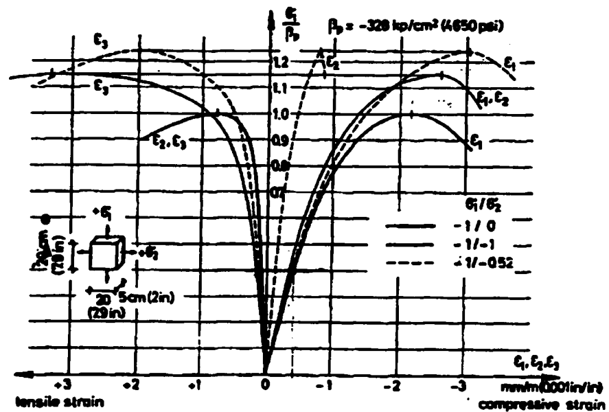
Figure 3.7. Longitudinal and Transversal Stress-Strain Relationship for Biaxial Test (Kupfer and Hilsdorf, 1969)
