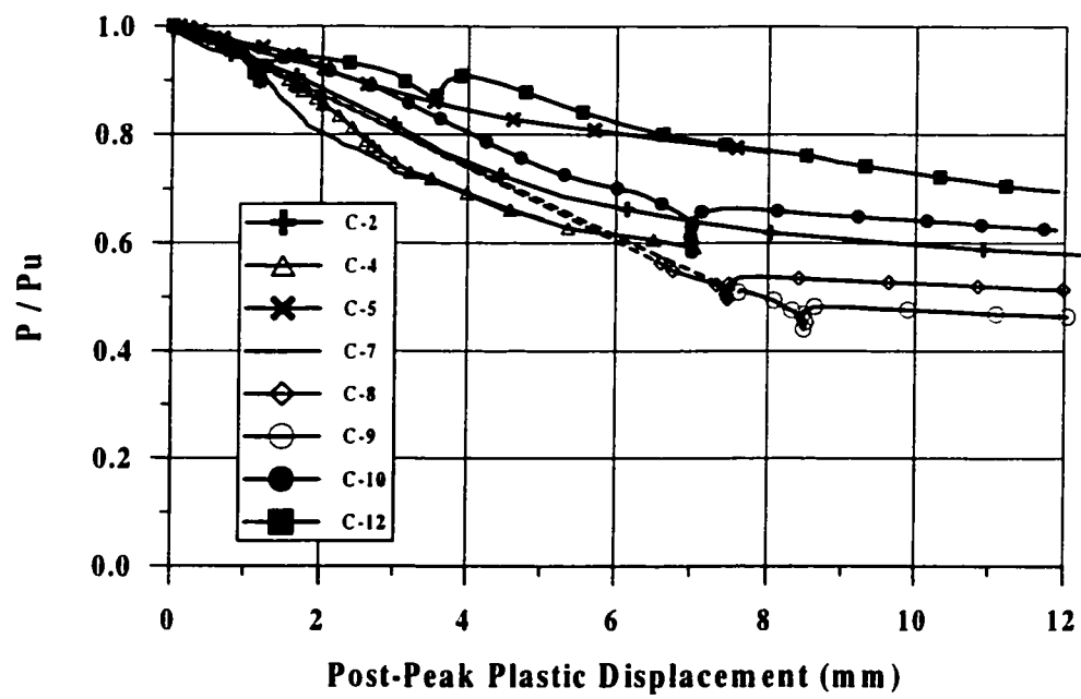
FIG. 11. Normalised Load vs. Post-Peak Plastic Displacement
