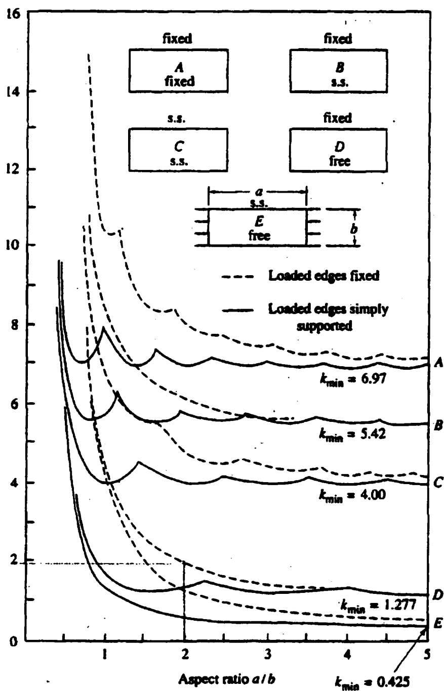
Figure 3.4. Variation of Plate Buckling Coefficient k with a/b Ratio (Salmon and Johnson, 1996)
