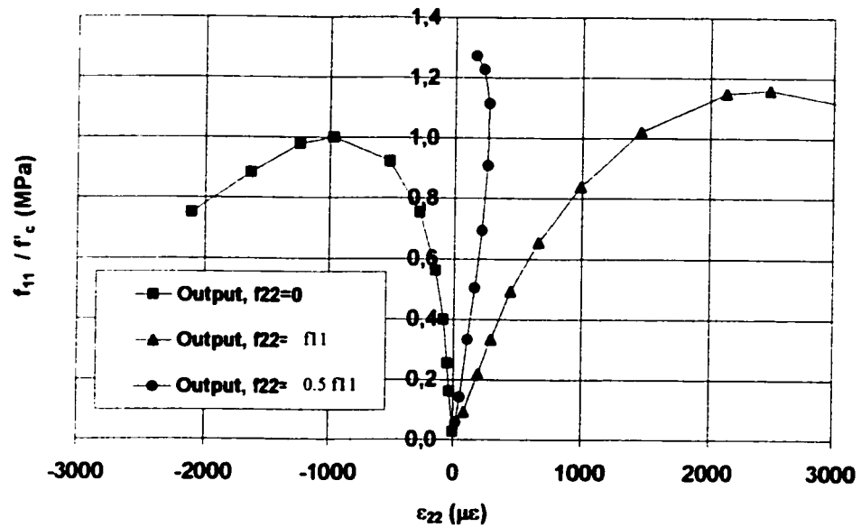
Figure 3.6. Normalised Longitudinal Stresses with Lateral Strain
