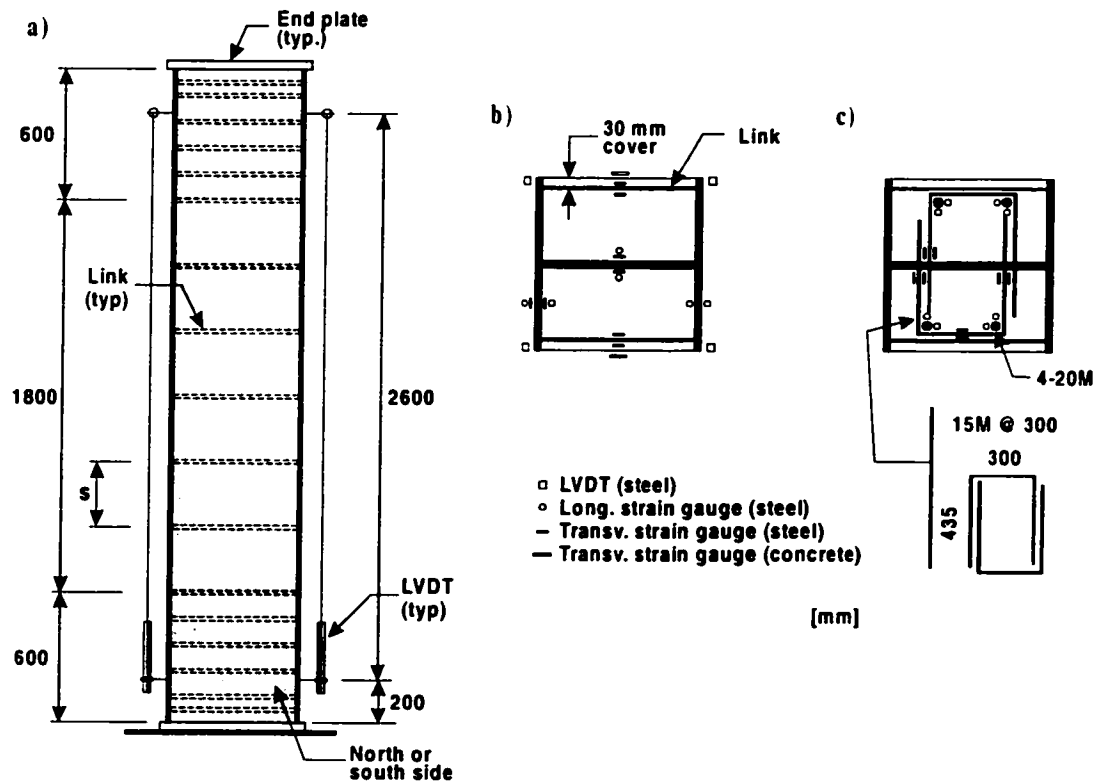
FIG. 2. Geometry and Instrumentation of Test Specimens: (a) Elevation; (b) Typical Cross-Section at Link Elevation; (c) Cross-Section at Link Elevation with Additional Reinforcement and Instrumentation for Specimen C-12
