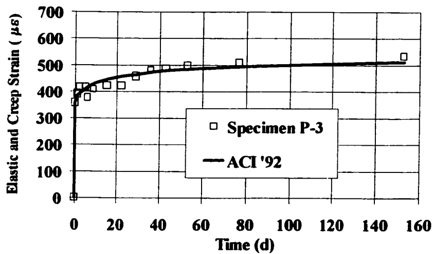
Figure. 3.11. Experimental and Predicted Elastic plus Creep Strain in Specimen P-3
