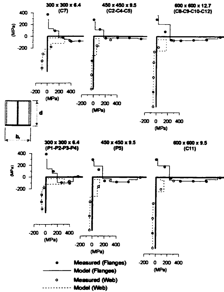
Fig. 6 Residual stresses in the steel shapes
