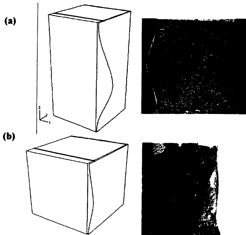
Fig. 7 Predicted and experimental failure modes for specimens with: (a) s = d ; (b) s = d/2
