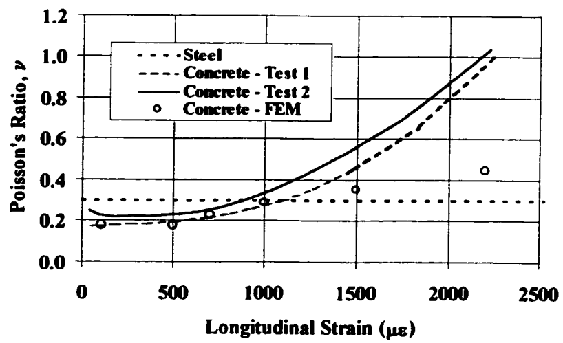
Fig. 5 Variation of the Poisson's ratio of concrete
