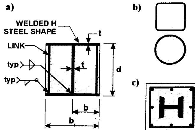
Figure 1.1 Composite Columns: (a) Proposed New Design; (b) CFT; (c) SRC.
