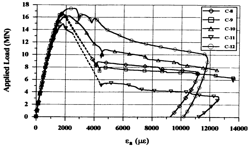
Figure 3.13. Load vs. Average Axial Strain Curves of Series 2 Specimens
