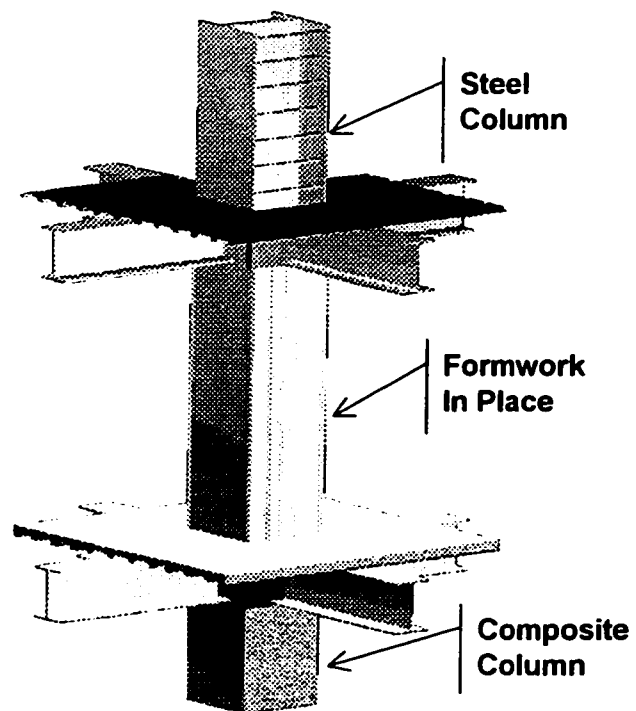
FIG. 2. Construction Stages for Partially Encased Composite Column
