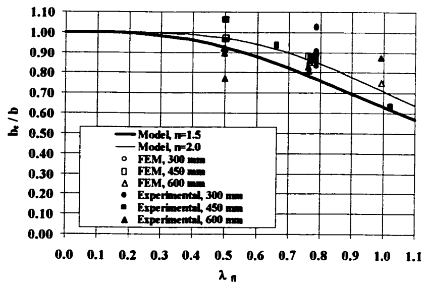
Fig. 13 Prediction model for flange effective width
