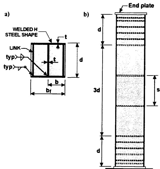
FIG. 1. Geometry of Stub Columns: (a) Cross-Section; (b) Elevation View
