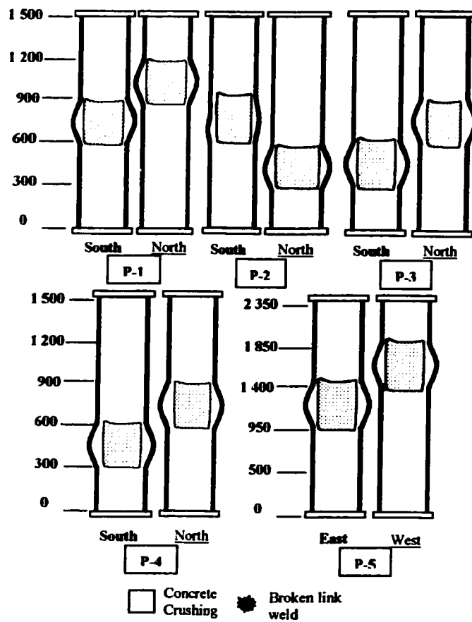
FIG. 10. Visual Observations on Specimens P-1 to P-5, after Failure
