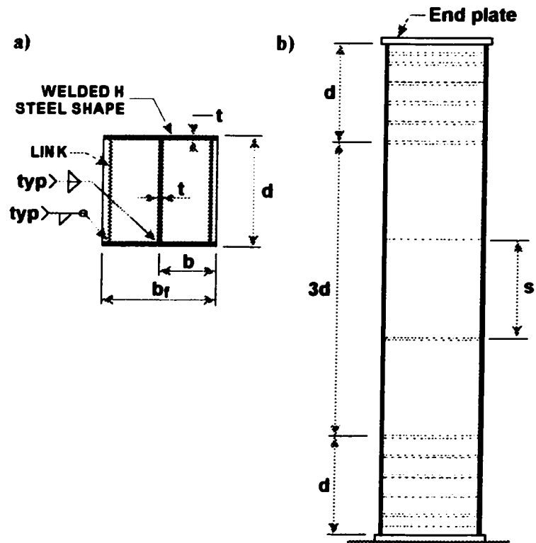
Fig. 2 Geometry of partially encased columns: (a) Cross-section; (b) Elevation of typical stub-column test specimens
