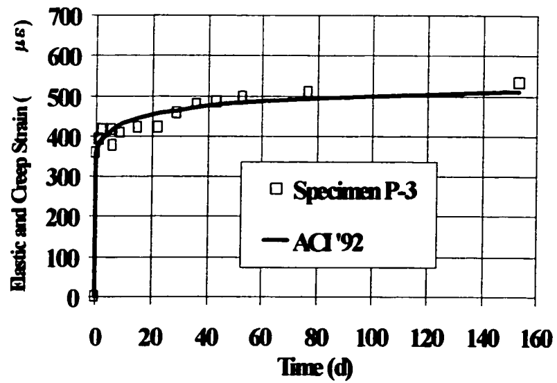
FIG. 9. Experimental and Predicted Elastic plus Creep Strain in Specimen P-3
