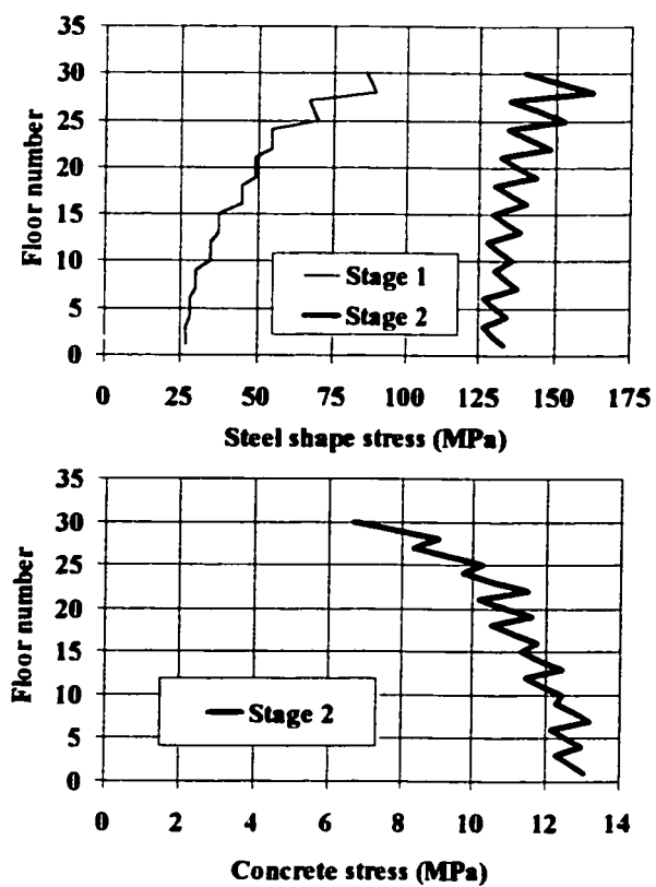
FIG. 3. Anticipated Stresses in Steel and Concrete of Columns in a 36-Storey Office Building
