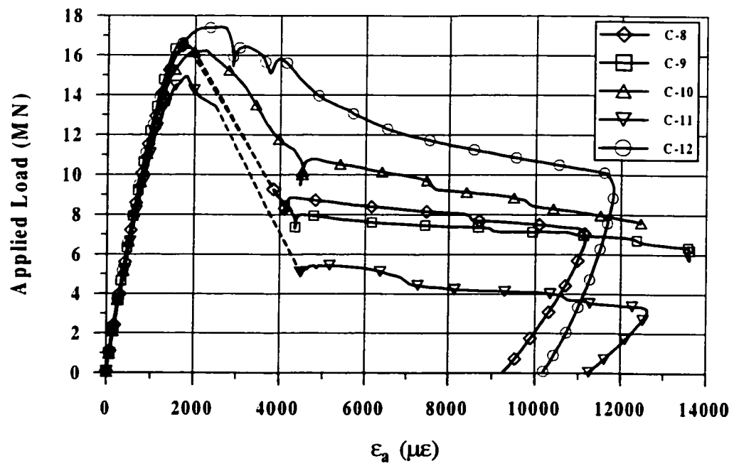
FIG. 7. Load vs. Average Axial Strain Curves of Test Specimens
