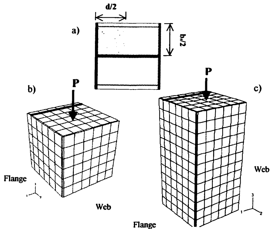
Figure 3.8 Finite element models of the column: (a) Quarter cross section; (b) Specimen with s = d/2 ; and (c) Specimen with s = d .
