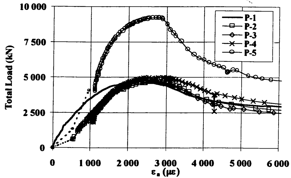
Figure 3.14. Load vs. Average Axial Strain Curves of Series 3 Specimens
