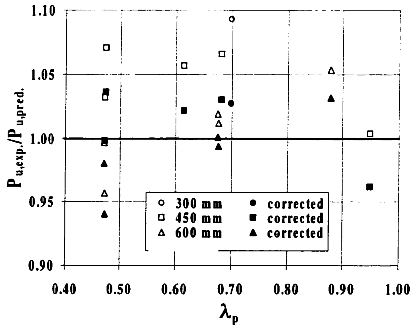
FIG. 12. Experimental-to-Predicted Load Ratio for Specimens C-2 to C-12
