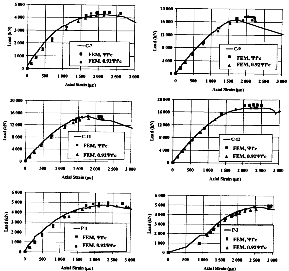
Figure 3.15 Load-strain behaviour of specimens and FE models
