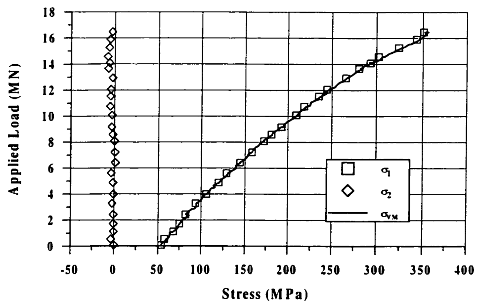
FIG. 8. Web Stresses in Specimen C-8
