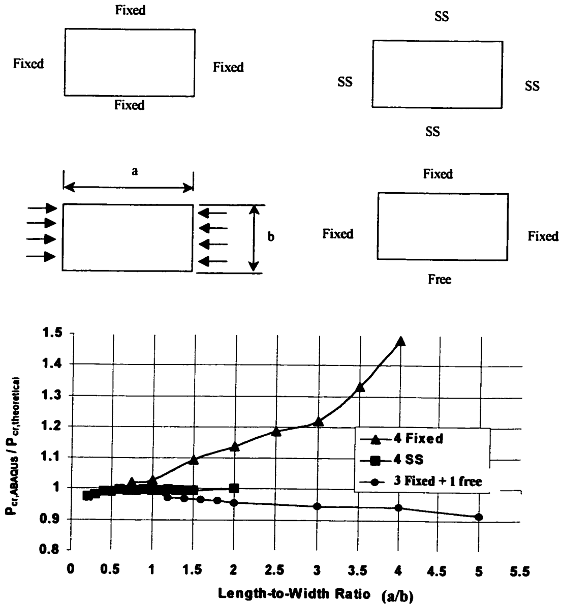
Figure 3.3. Buckling Model with Different Aspect Ratio and Boundary Conditions
