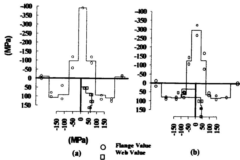
FIG. 5. Measured Residual Stresses: (a) P-1 to P-4; (b) P-5
