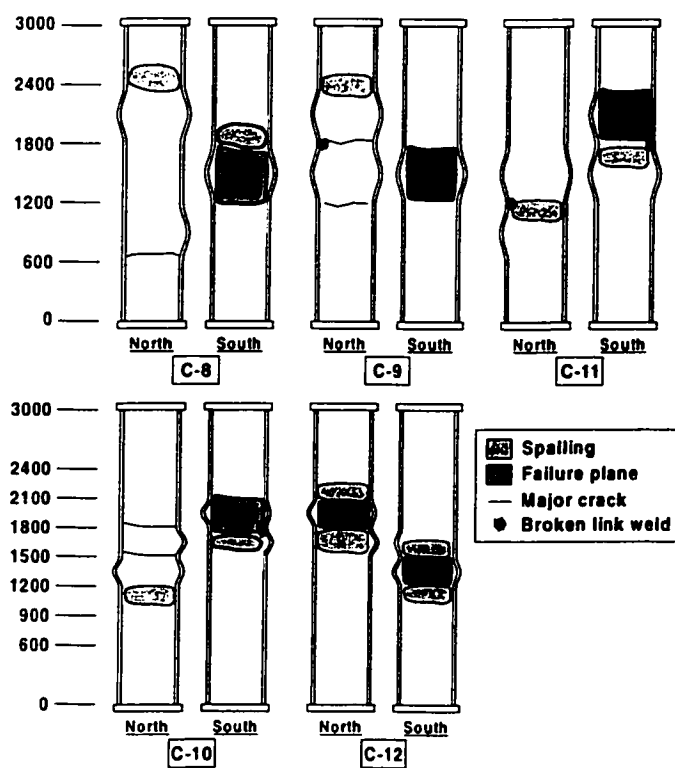
FIG. 5. Observations on Specimens C-8 to C-12 after Failure
