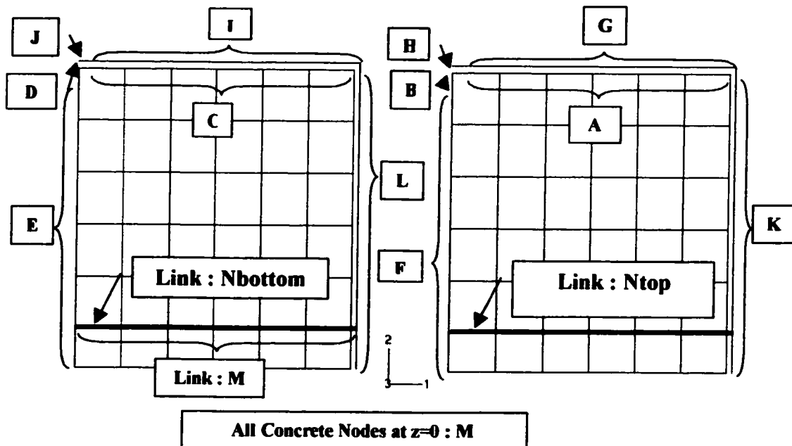
FIG. 3.9. Boundary Conditions at : (a) z = 0 ; (b) z > 0
