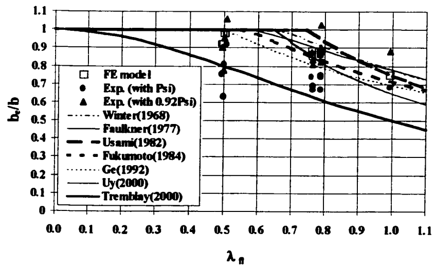
Fig. 12 Flange buckling capacity with plate slenderness
