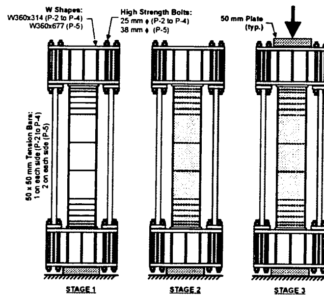
FIG. 4. Loading Stages 1 to 3
