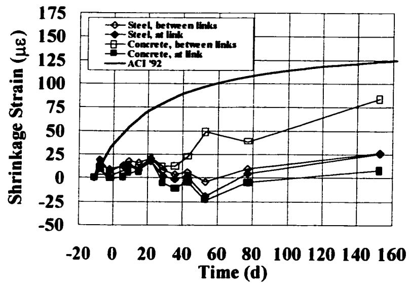
Figure 3.10. Average Shrinkage Axial Strain in Specimens P-1, P-2, and P-7
