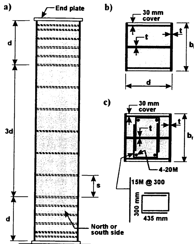
Figure 3.1. Geometry of Stub Columns: (a) Elevation View; (b) Cross-Section without Additional Reinforcement; (c) Cross-Section with Additional Reinforcement
