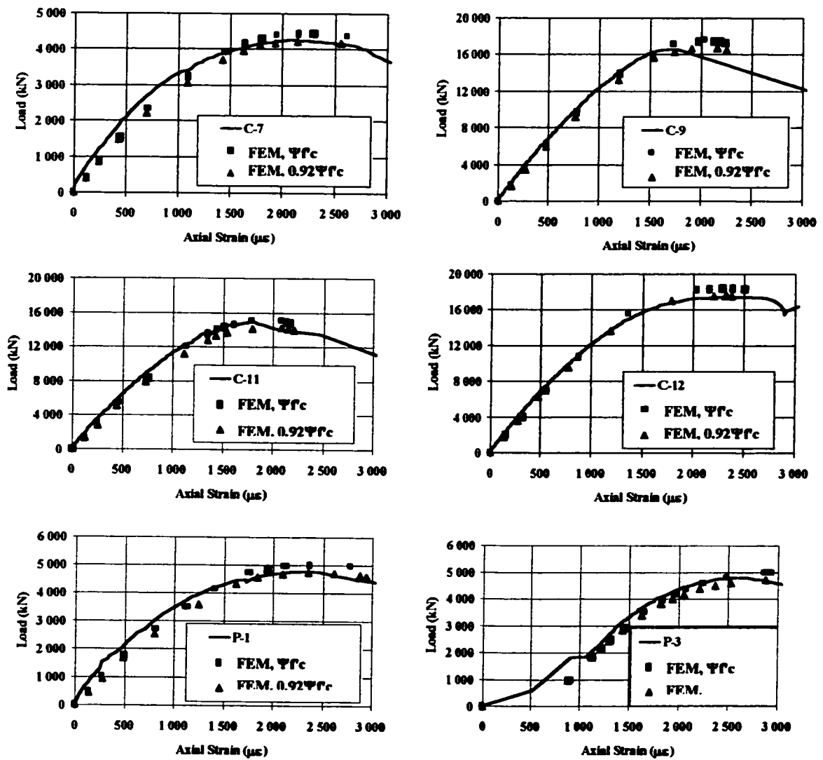
Fig. 8 Load-strain behaviour of specimens and FE models
