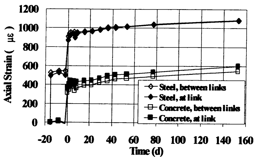
FIG. 8. Total Strain History for Specimen P-3
