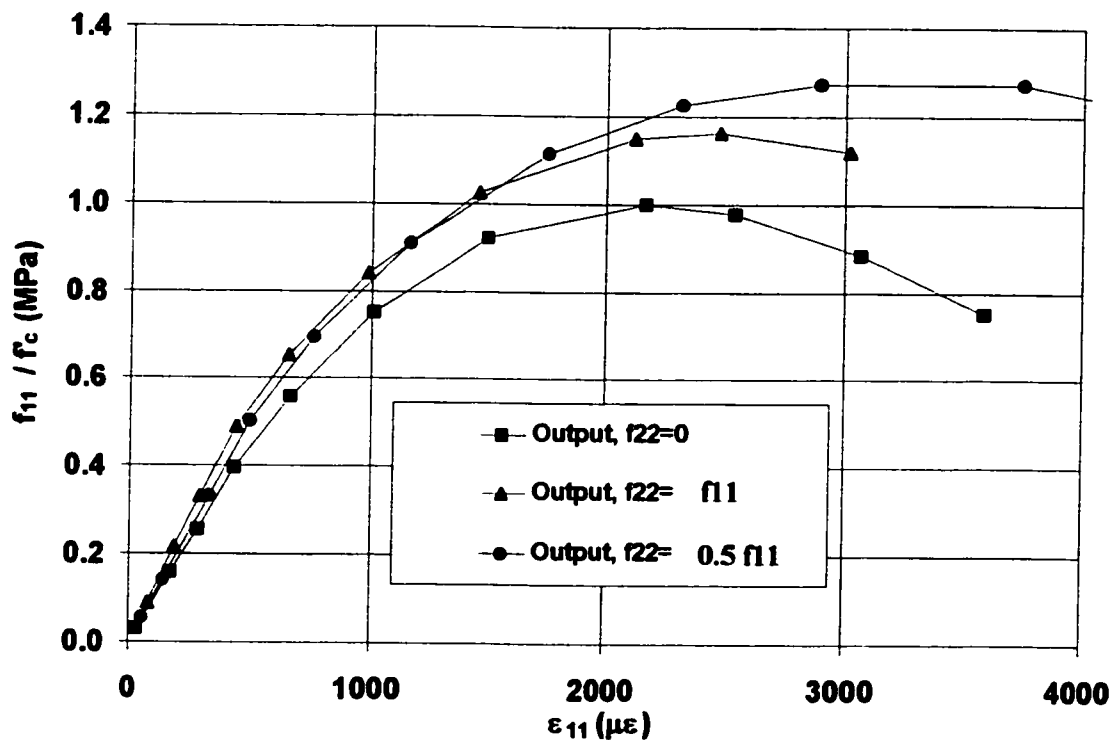
Figure 3.5. Normalized Longitudinal Stresses with Longitudinal Strain
