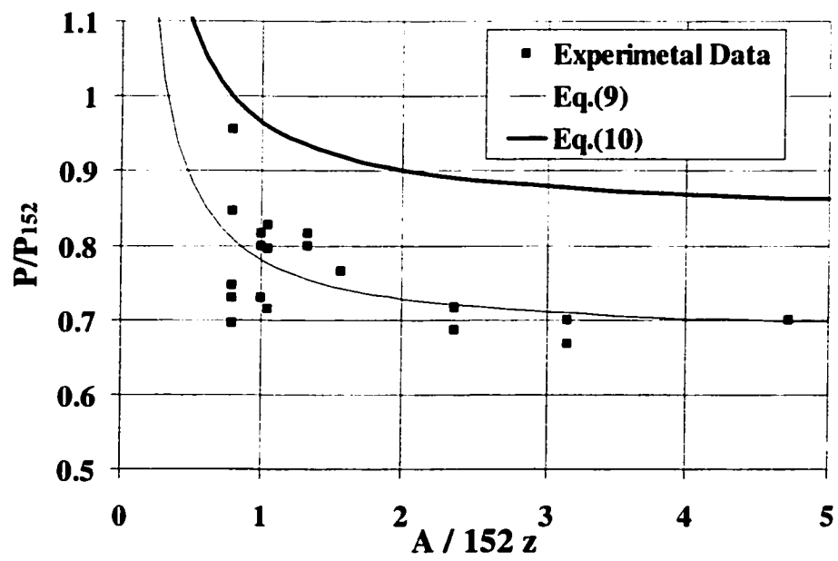
FIG. 13. Size Effect on Concrete Strength
