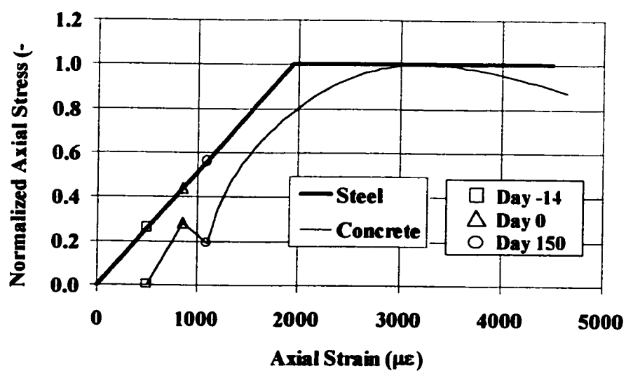
FIG. 13. Stress-Strain Response in Steel and Concrete of Specimen P-4
