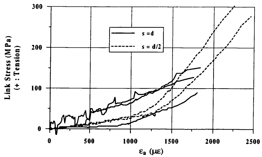
FIG. 9. Link Axial Stresses in Large Specimens Outside Concrete Failure Zone
