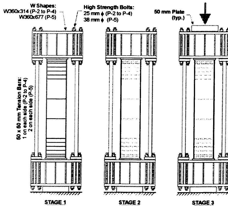
Fig. 3 Loading stages 1 to 3
