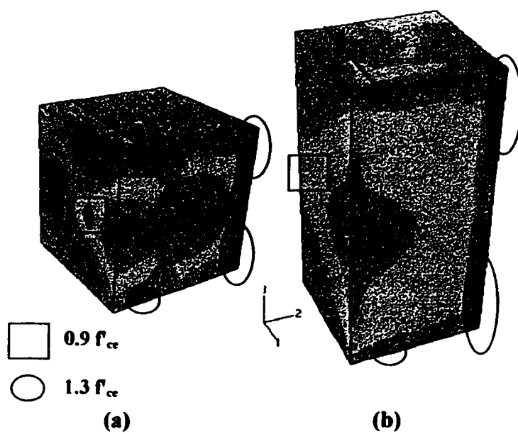
Fig. 9 Axial stresses in the concrete at peak load for specimens: (a) C-2; (b) C-4
