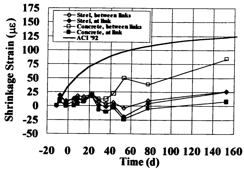
FIG. 7. Average Shrinkage Axial Strain in Specimens P-1, P-2, and P-7
