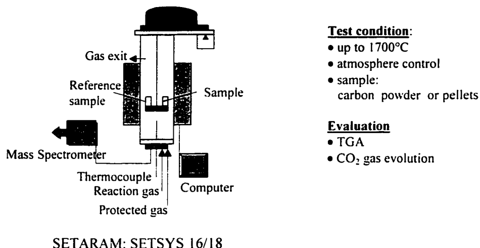
Figure 4.12 Thermobalance with mass spectrometer: Set-up A
