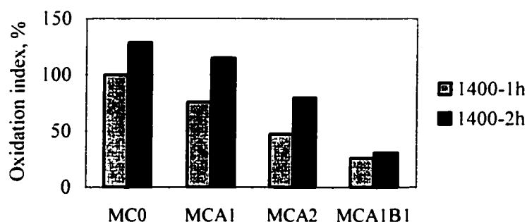
Figure 4.18 Influence of antioxidants on oxidation resistance of the matrixes
