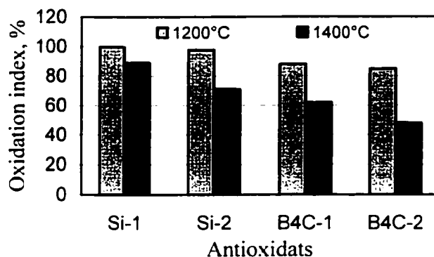
Figure 4.28 Influence of antioxidants on oxidation resistance of MgO-MA-EG castables after firing at 1200°C and 1400°C for 3 hours in Set-up B
