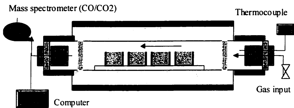
Figure 2.14 Horizontal furnace [96]
