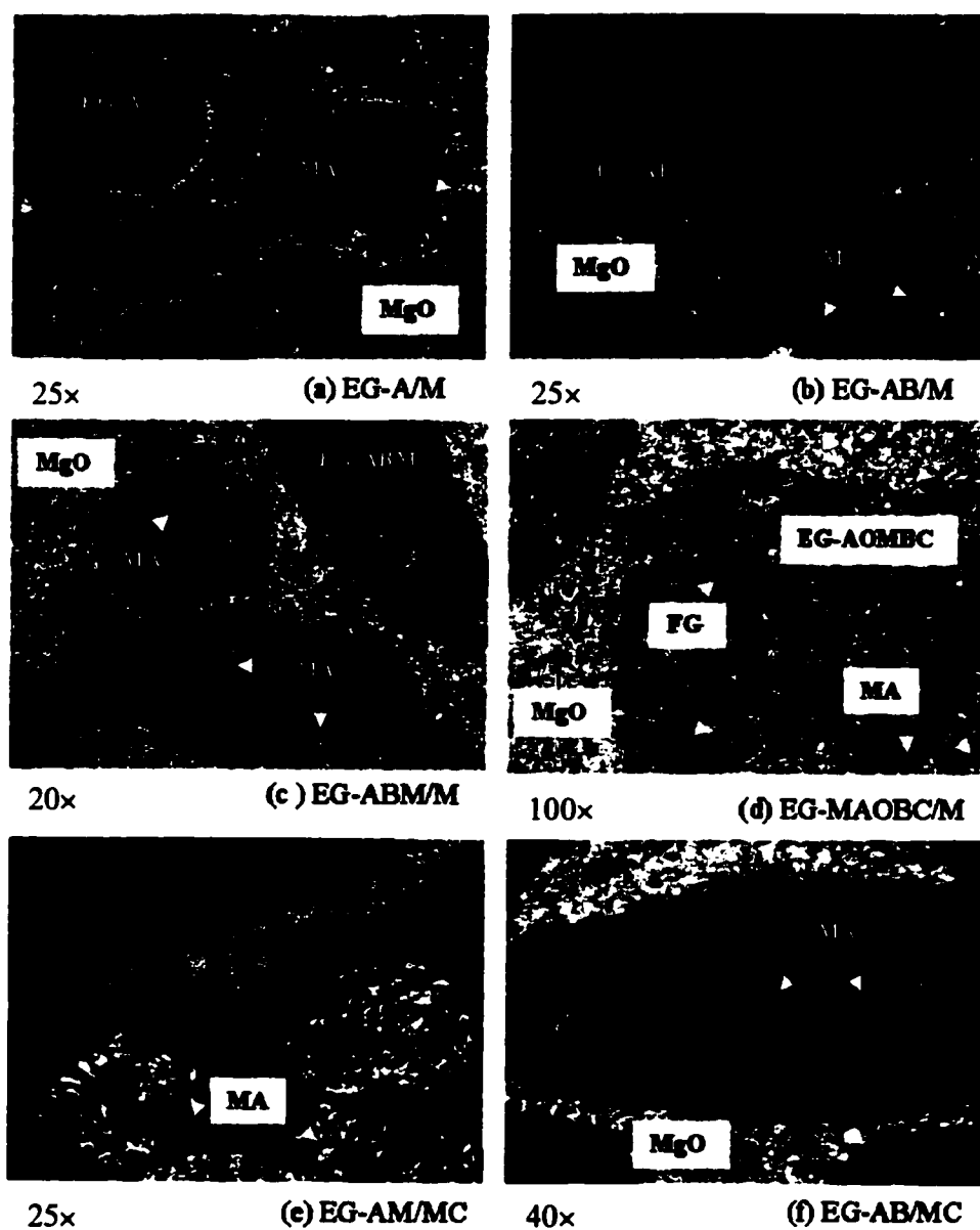
Figure 3.10 New compounds formation in (EG-A.O.)_{MA} in a matrix of magnesia without fine carbon ( /M ) and with fine carbon ( /MC ) (CLM observation: spinel-green, MgO -blue or purple, graphite-black)
