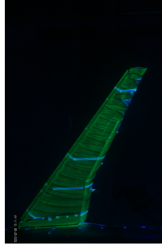
(b) \alpha = 17.7^\circ , oil-flow visualization;
