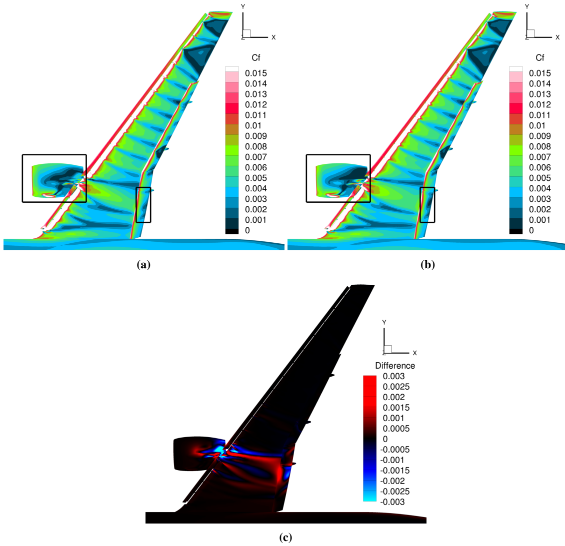
Fig. 23 Skin friction at 16° for case 3.2: a) standard restart, b) SFD-restart, c) difference between both.
