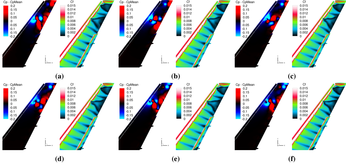
Fig. 15 Test case 3.2 at \alpha = 16^\circ : pseudo-instability over a pseudo-period, successively at iterations a) 39540, b) 39661, c) 39782, d) 39902, e) 40023, and f) 40144.
