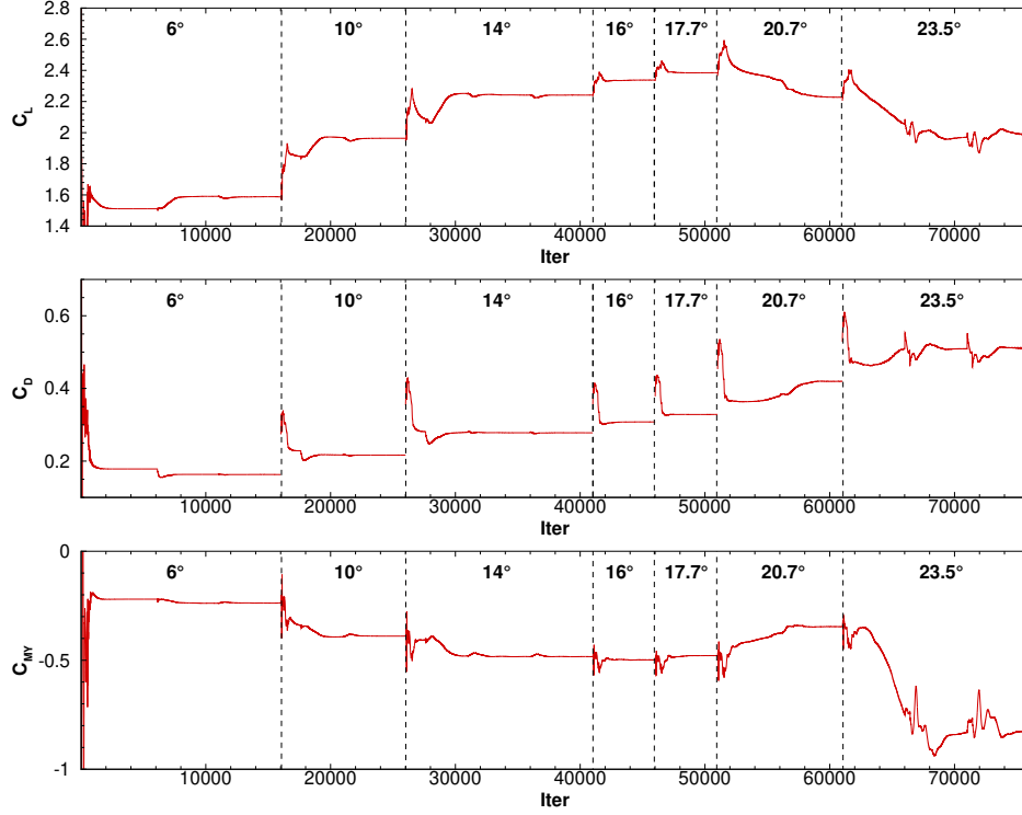
Fig. 3 Test case 2.3: iterative convergence of the aerodynamic coefficients.
