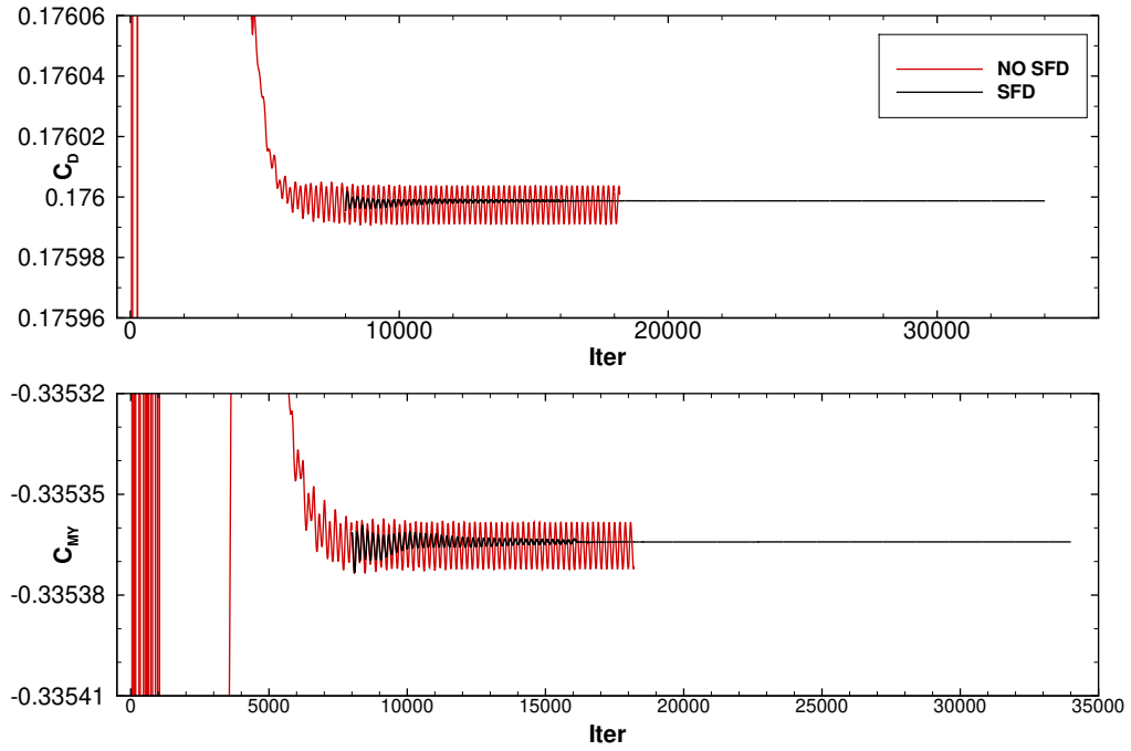
Fig. B1 Test case 3.2 at 6^\circ : drag and pitching moment iterative convergence with and without SFD
