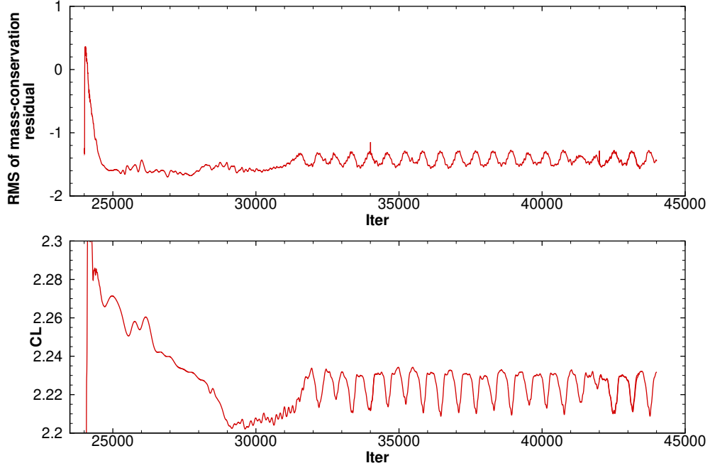
Fig. 13 Test case 3.2 at 16^\circ : zoom on a pseudo-period in the limit cycle.
