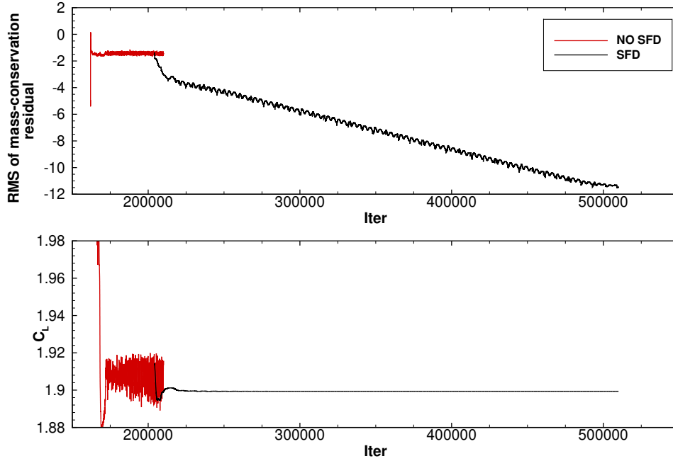
Fig. 22 Test case 3.2 at \alpha = 20^\circ : iterative convergence using SFD.
