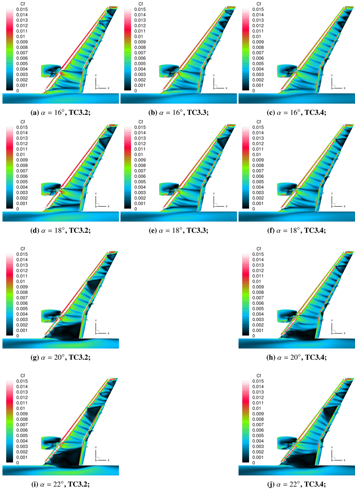
Fig. A1 Skin friction coefficient evolution with \alpha : Cases 3.2 (left), 3.3 (middle), 3.4 (right).
