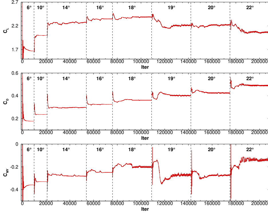
Fig. 8 Test case 3.4: iterative convergence of the aerodynamic coefficients.
