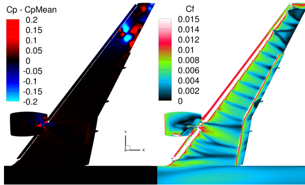
Fig. 14 Test case 3.2 at 16^\circ : instantaneous pressure coefficient and skin friction.
