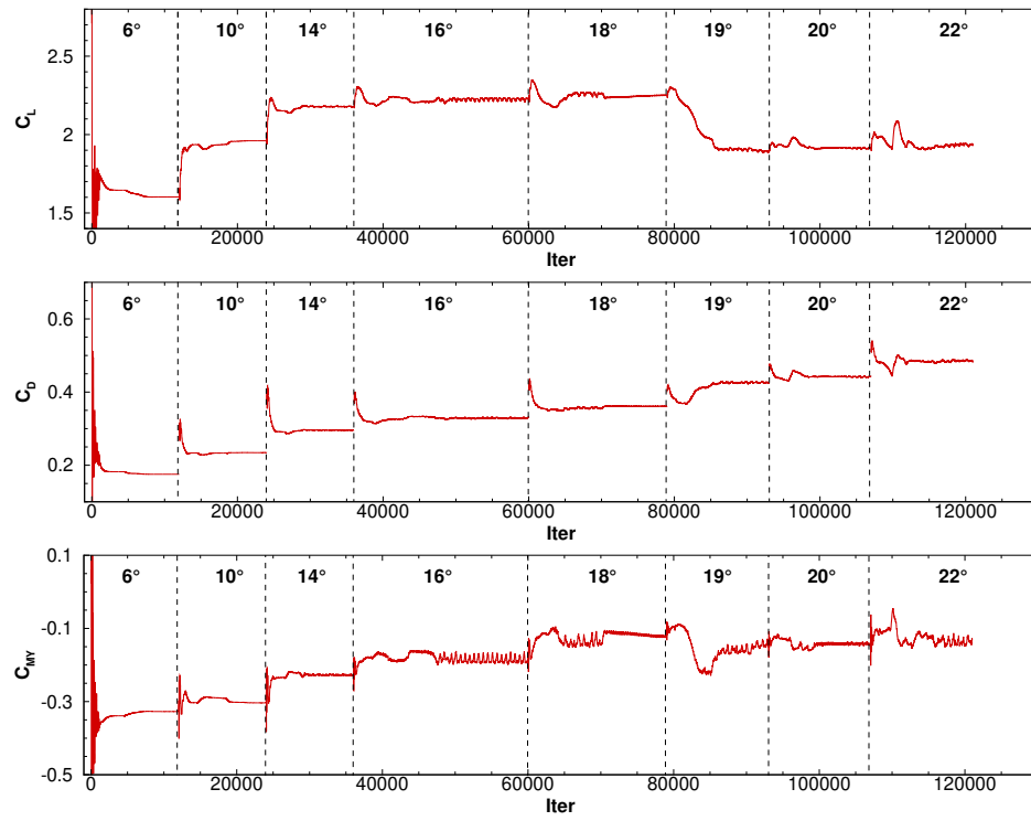
Fig. 6 Test case 3.2: iterative convergence of the aerodynamic coefficients.
