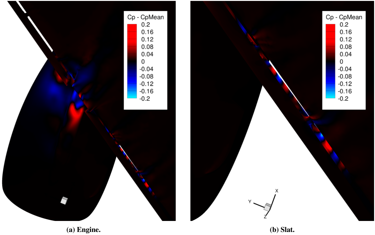
Fig. 16 Test case 3.2 at 16^\circ : instantaneous pressure coefficient distributions.
