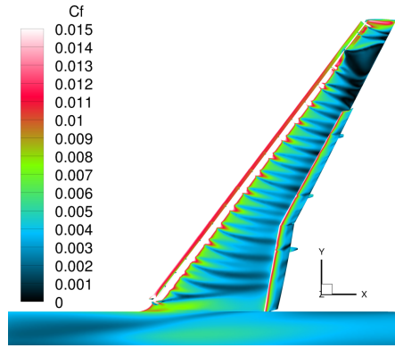
(a) \alpha = 17.7^\circ , TC2.3;
