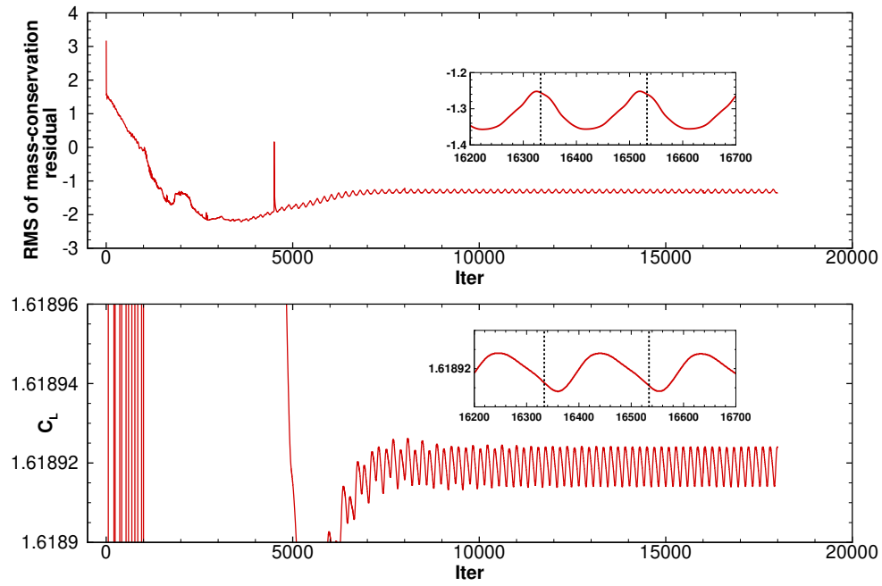
Fig. 10 Test case 3.2 at 6^\circ : zoom on a pseudo-period in the limit cycle.
