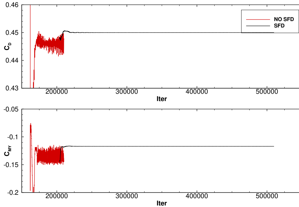
Fig. B3 Test case 3.2 at 20°: drag and pitching moment iterative convergence with and without SFD
