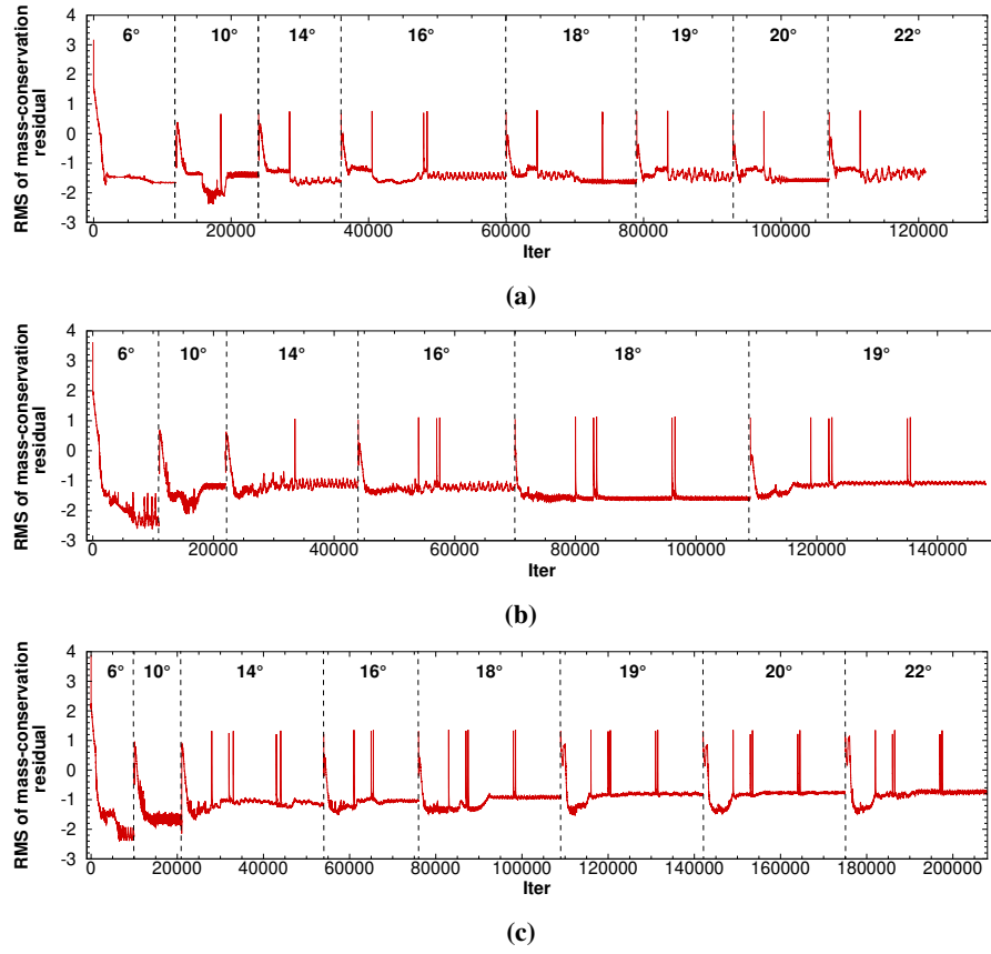
Fig. 5 Iterative convergence: RMS of mass-conservation residual for test case a) 3.2, b) 3.3, and c) 3.4.
