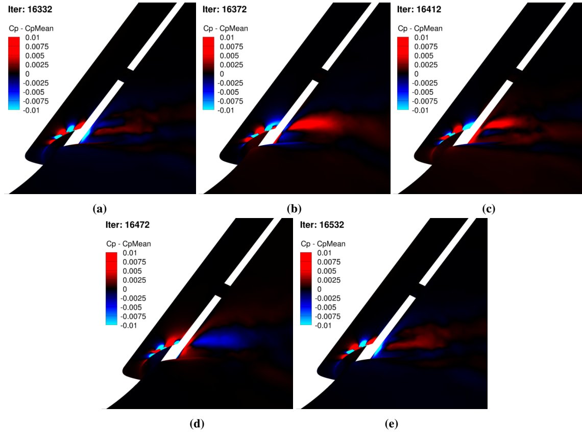
Fig. 12 Test case 3.2 at \alpha = 6^\circ : pseudo-instability over a pseudo-period, successively at iterations a) 16332, b) 16372, c) 16412, d) 16472, and e) 16532.
