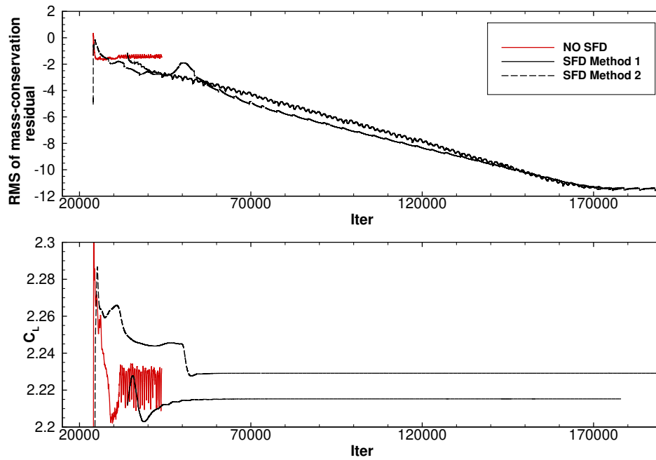
Fig. 21 Test case 3.2 at \alpha = 16^\circ : iterative convergence using SFD.
