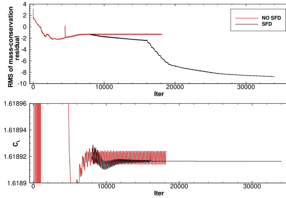
Fig. 20 Test case 3.2 at \alpha = 6^\circ : iterative convergence using SFD.
