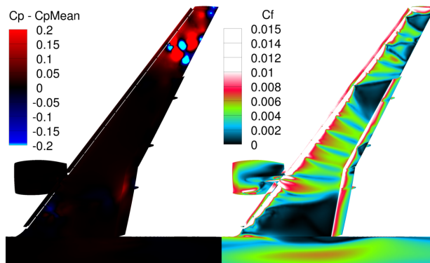
Fig. 18 Test case 3.2 at 20^\circ : instantaneous pressure coefficient and skin friction.
