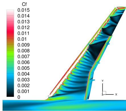
(c) \alpha = 20.7^\circ , TC2.3;
