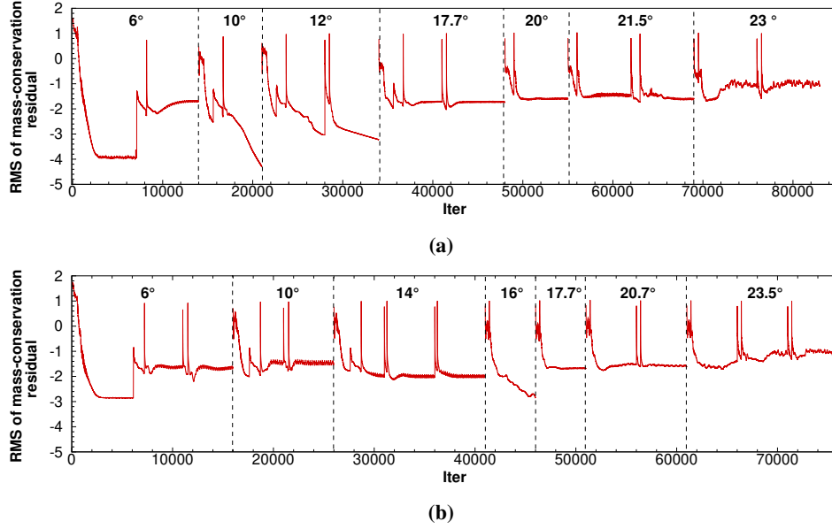
Fig. 1 Iterative convergence: RMS of mass-conservation residual for test case a) 2.2 and b) 2.3.
