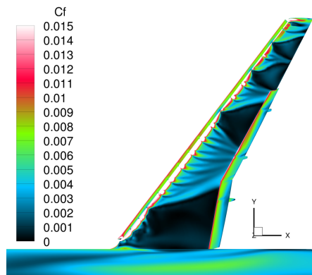
(e) \alpha = 23.5^\circ , TC2.3;
