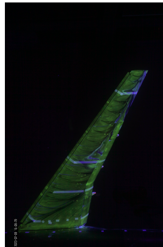
(f) \alpha = 23.5^\circ , oil-flow visualization;
