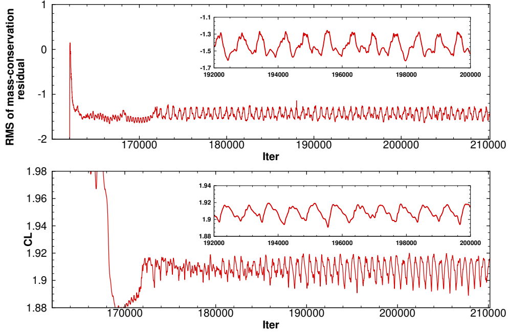
Fig. 17 Test case 3.2 at 20^\circ : zoom on a pseudo-period in the limit cycle.
