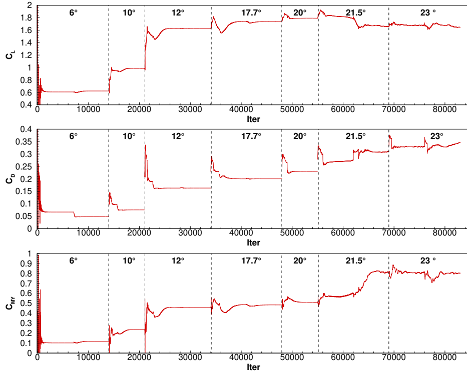
Fig. 2 Test case 2.2: iterative convergence of the aerodynamic coefficients.
