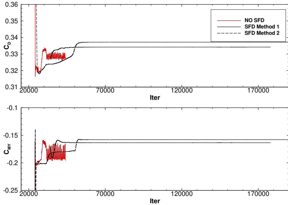
Fig. B2 Test case 3.2 at 16^\circ : drag and pitching moment iterative convergence with and without SFD, using two initialization methods.
