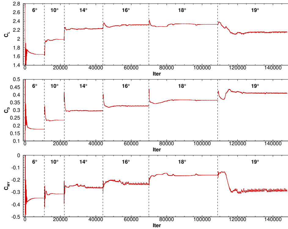
Fig. 7 Test case 3.3: iterative convergence of the aerodynamic coefficients.
