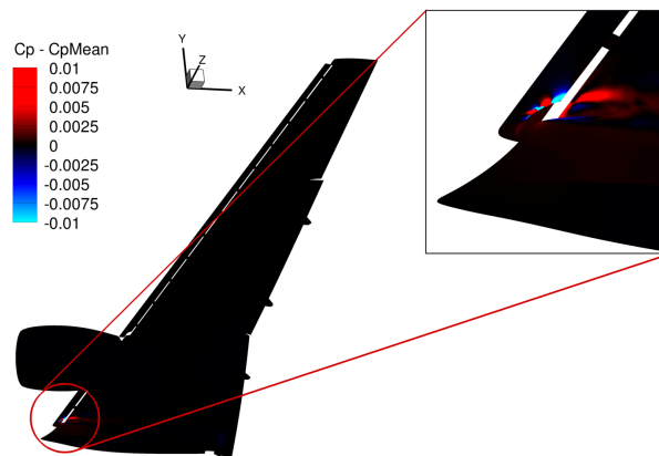
Fig. 11 Test case 3.2 at 6^\circ : instantaneous pressure coefficient.
