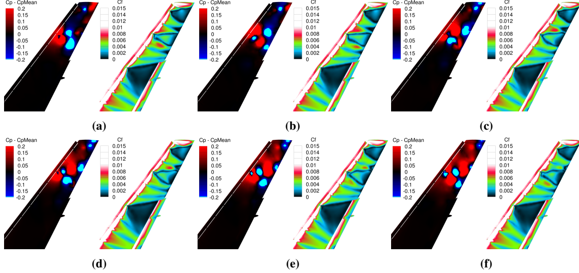
Fig. 19 Test case 3.2 at \alpha = 20^\circ : pseudo-instability over a pseudo-period, successively at iterations a) 197645, b) 197784, c) 197922, d) 198060, e) 198200, and f) 198339.
