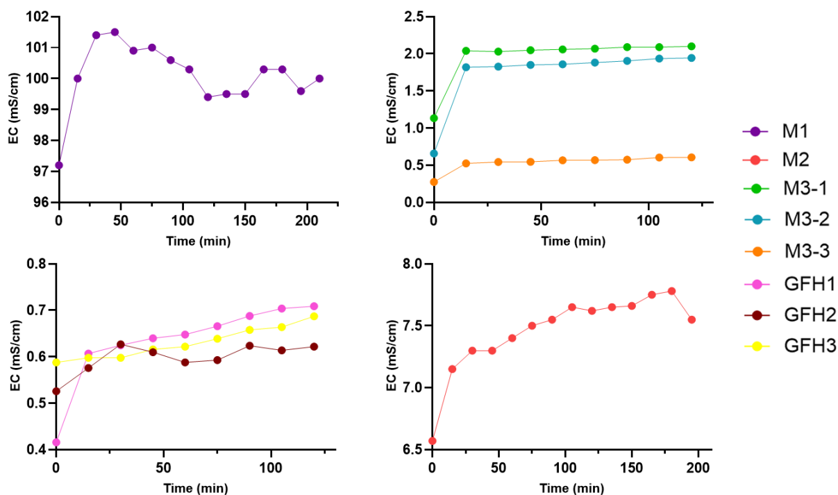
Figure 6.3 Evolution of water electrical conductivity (EC) during microbubble ozonation
