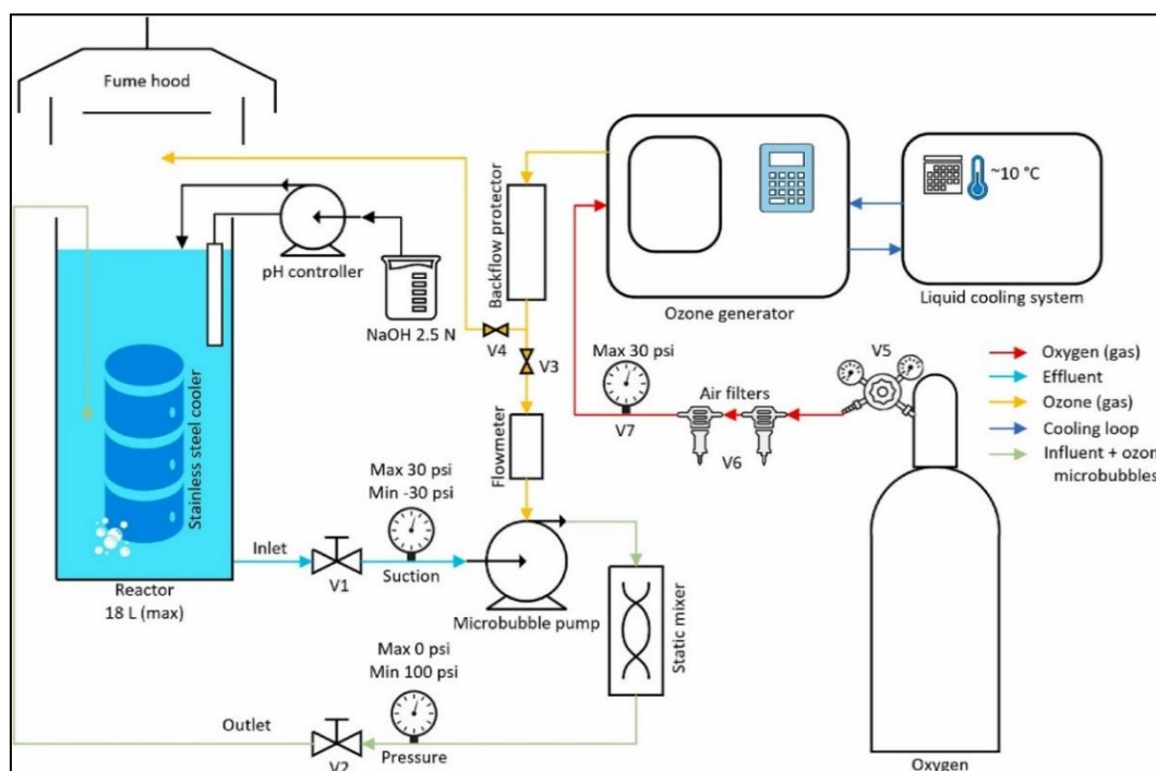
Figure 6.2 Schematic pilot-scale ozonation system under recirculated flow
