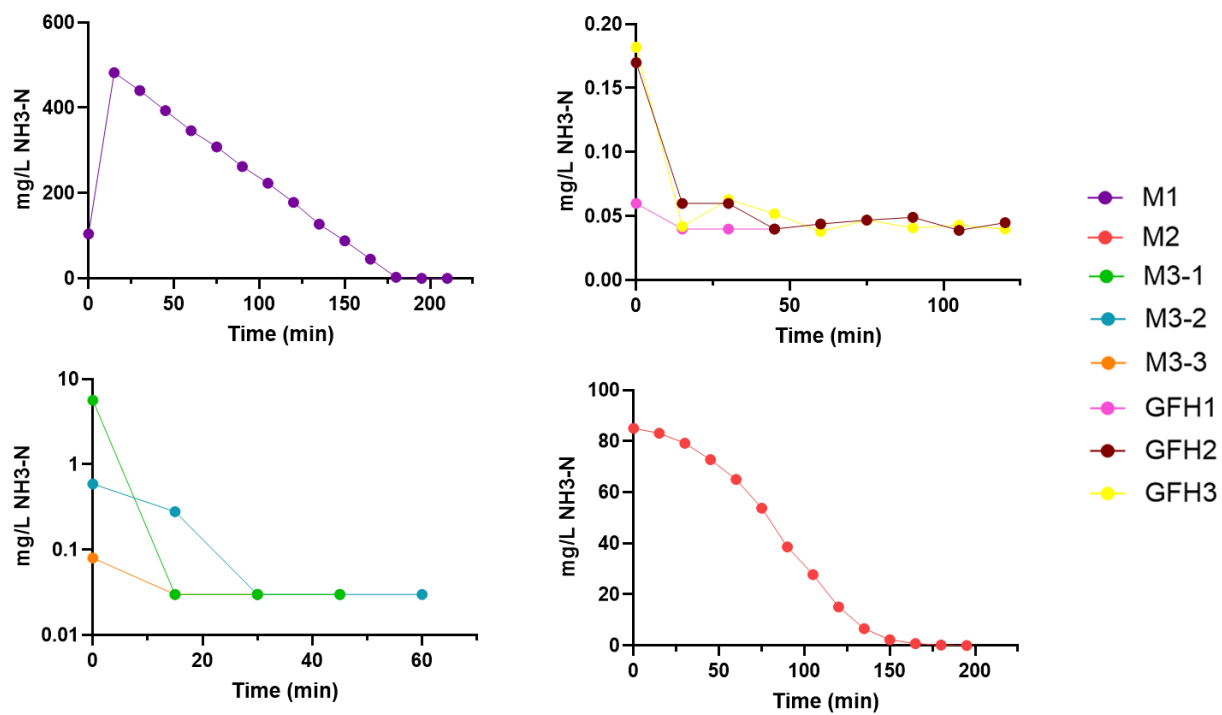
Figure 6.4 Evolution of ammoniacal nitrogen ( \text{NH}_3\text{-N} ) during microbubble ozonation
