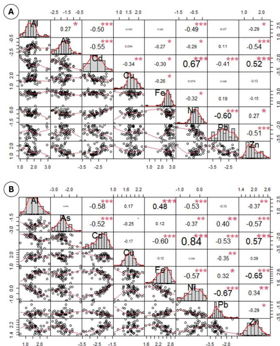
Figure 4.3 Correlation coefficient matrix for metallic elements in the non-toxic group (a) vs. toxic group (b). Histograms and red density curves on the diagonal show the distribution of each element. The upper panels display Pearson correlation coefficients with significance levels (* p < 0.05 ; ** p < 0.01 ; *** p < 0.001 ). The lower panels show scatterplots with red trend lines indicating pairwise relationships.
