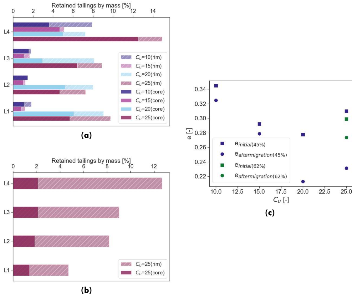
Figure 4: Results for a filter ratio = 14:(a) retained tailings per layer for an initial solids content of 45%; (b) retained tailings per layer for an initial solids content of 62% (c), initial and post-migration void ratio
