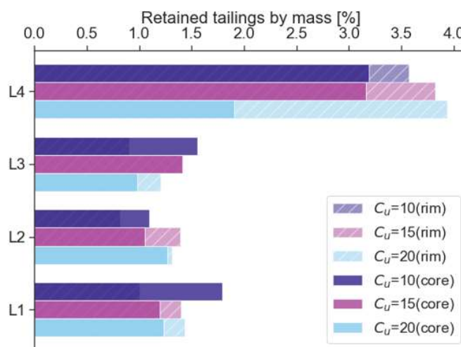
Figure 3 (a): Results for a filter ratio ( d_{15-wr}/d_{85-tailings} ) = 8.5 with an initial tailings solids content of 45%: retained tailings per layer
