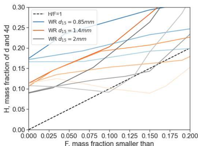
Figure 1: (b) Internal stability of each PSD (after Kenney & Lau, 1985, 1986)
