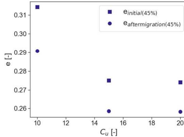
Figure 3 (b): Results for a filter ratio ( d_{15-wr}/d_{85-tailings} ) = 8.5 with an initial tailings solids content of 45%: initial and post-migration void ratio
