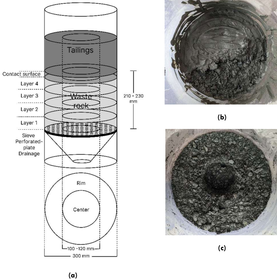
Figure 2: (a) Physical model of the column migration test; (b) removal of the contact surface; (c) sampling of a specimen center
