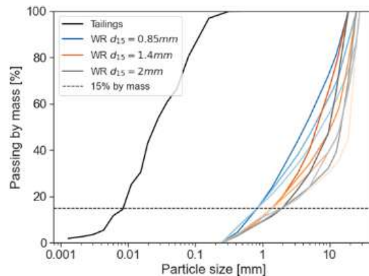
Figure 1: (a) PSD of tailings and waste rock (after Kenney & Lau, 1985, 1986)
