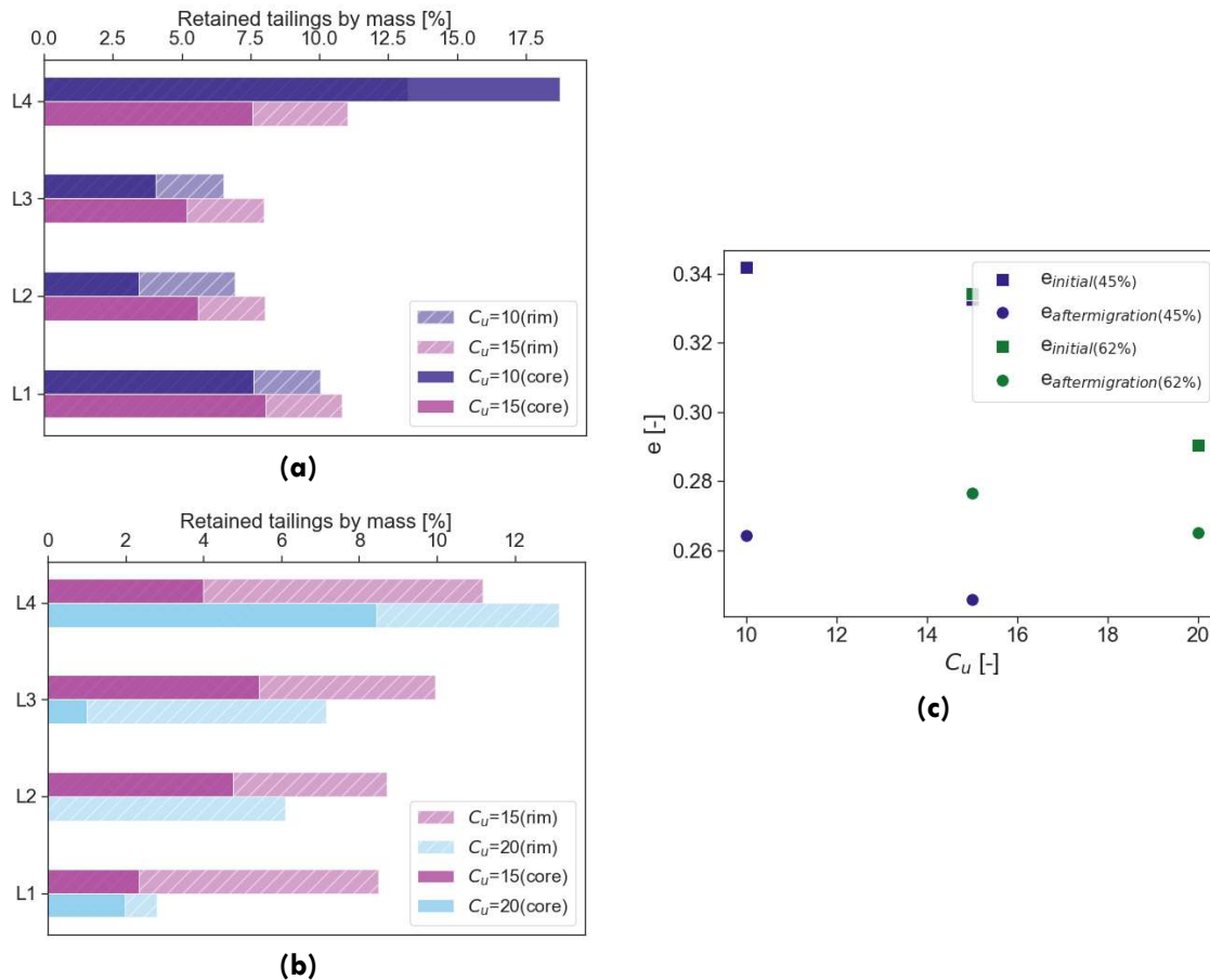
Figure 5: Results for a filter ratio = 20: (a) retained tailings per layer for an initial solids content of 45%; (b) retained tailings per layer for an initial solids content of 62%; (c) initial and post-migration void ratio
