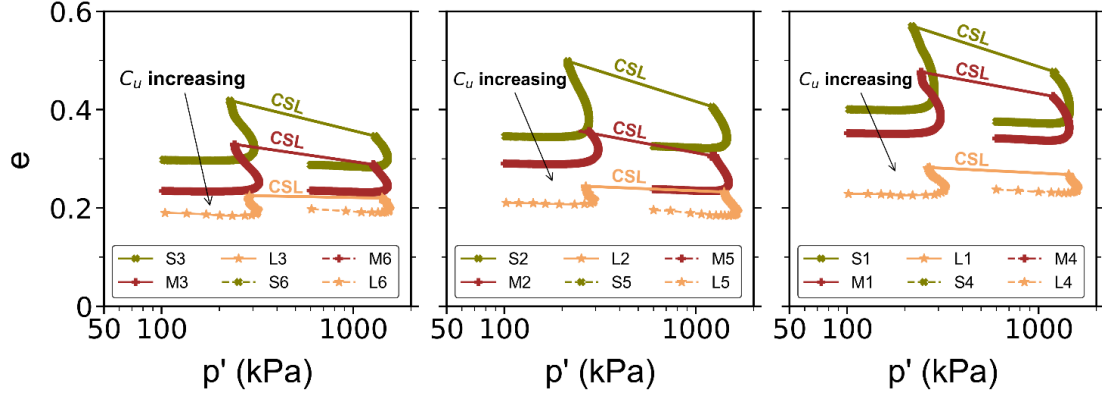
Figure 4. Critical state lines (CSL) of S, M and L specimens: C_u decreasing for a given specimen size from left to right .
