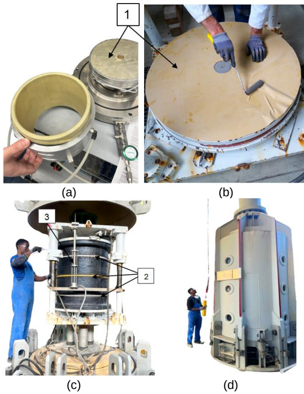
Figure 2. Specimen preparation: (a) S and M specimens showcasing the greased rubber sheet installation for lubrication (1); (b) L specimen (D=800 mm) base platen; (c) circumference bandage and extensometer installation (2 and 3); (d) L specimen ready for testing.
