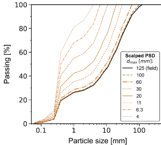
Figure 1. PSDs of the small-scale specimens prepared through scalping.
