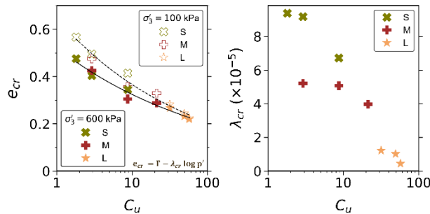
Figure 5. Critical state parameters analysis on S, M and L specimens: e_{cr} estimates ( left ) and CSL slope \lambda_{cr} ( right ).
