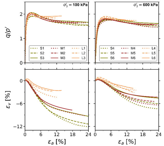
Figure 3. Stress-strain results on S, M and L specimens at \sigma'_3 = 100 kPa (left) and 600 kPa (right): volumetric deformations are plotted at the bottom subplots, respectively.
