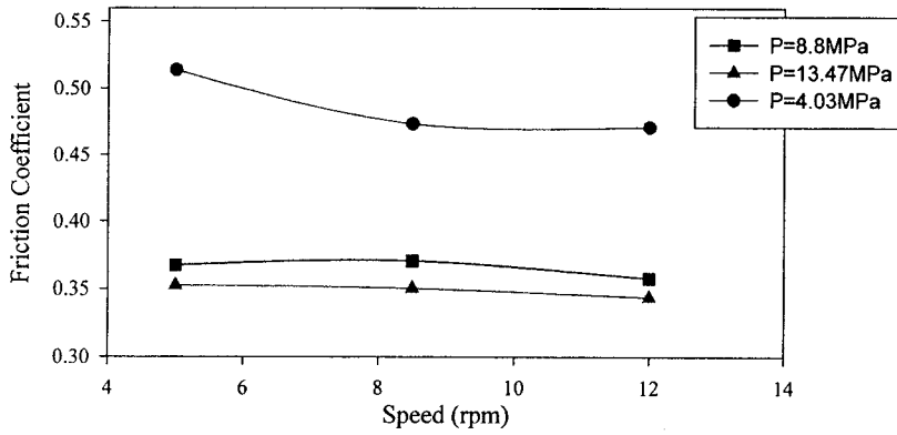
(B) Interface Temperature=60°C, \mu_d as a function of plate velocity at P=4.03 MPa, 8.8 MPa, and 13.47 MPa.
