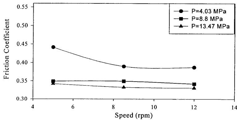
(C) Interface Temperature = 81°C, \mu_d as a function of plate velocity at P=4.03 MPa, 8.8 MPa, and 13.47 MPa.
