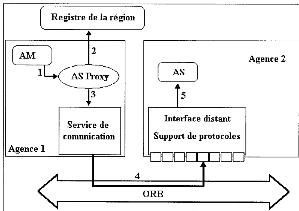
Figure 4.10 Communication entre AM et AS sous Grasshopper
