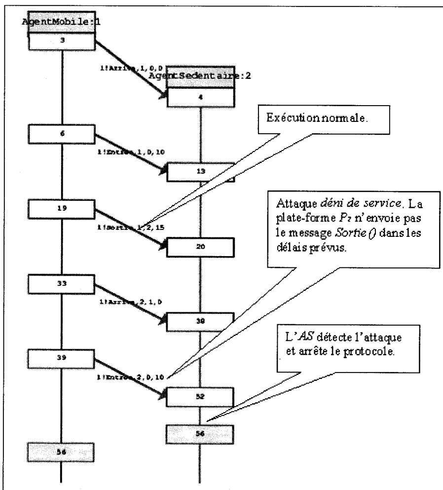
Figure 4.2 Simulation 2 : Déni de service
