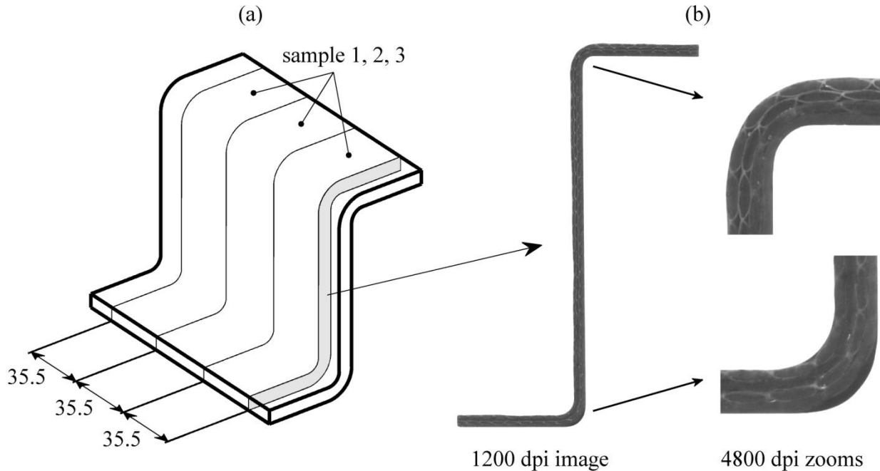
Figure 3-6 : Sample preparation for image analysis: (a) cutting pattern (dimensions in mm); (b) typical scanned images.
