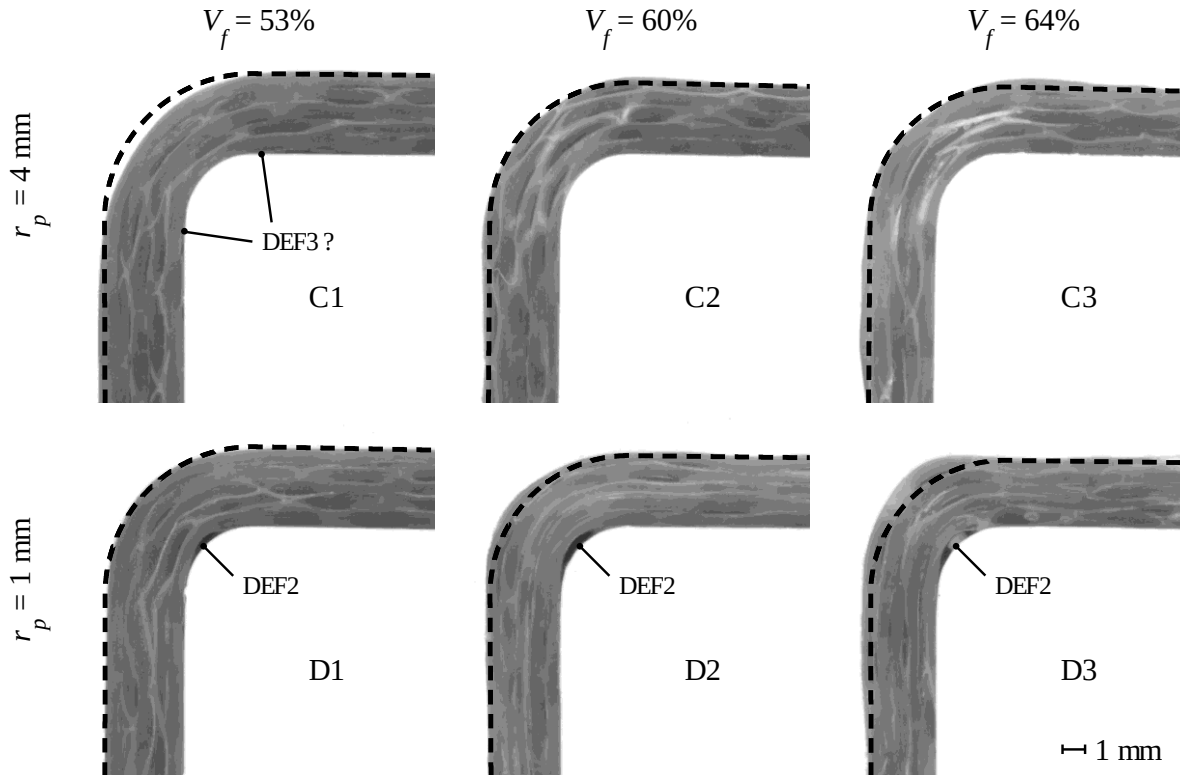
Figure 4-23 : Typical images of the convex corner of parts manufactured for two different inner preforming radii r_p = 1 mm and r_p = 4 mm.
