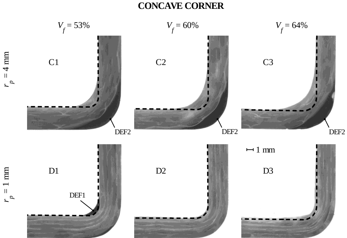
Figure 4-25 : Layup quality observed in the concave corner for two different inner preforming radii r_p = 1 mm and r_p = 4 mm.
