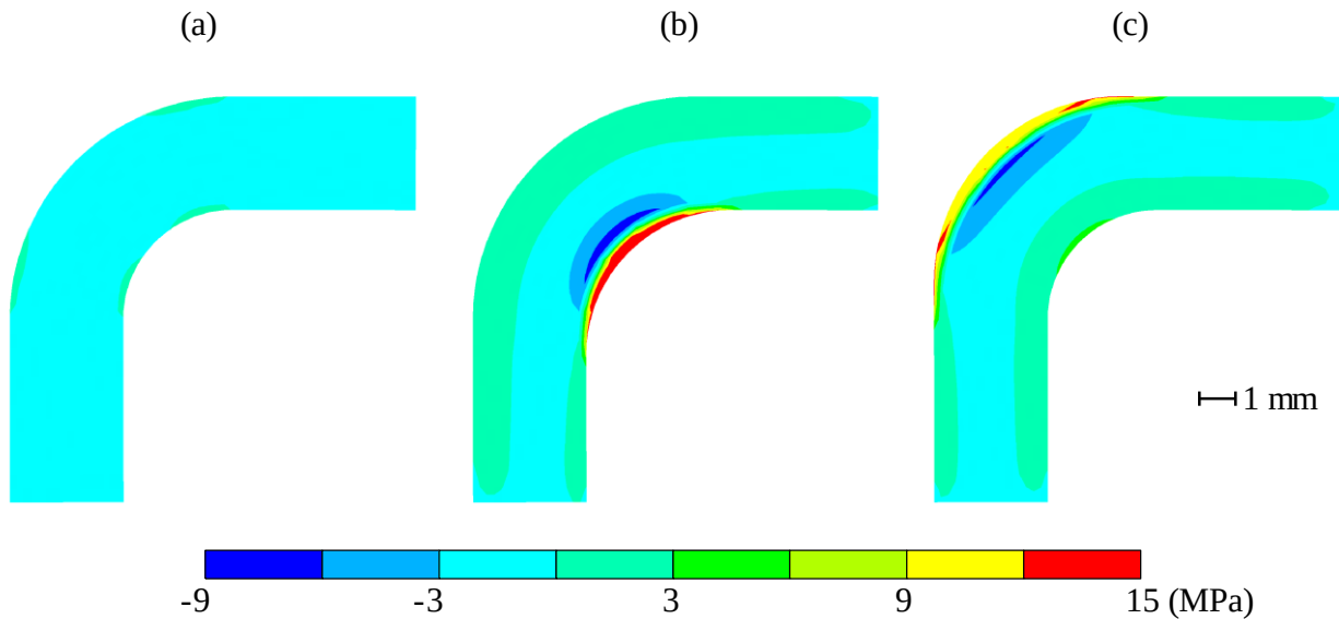
Figure 5-12 : Predicted longitudinal stress distribution during uniform cool down ( \Delta T = -68^\circ\text{C} ) for different corner qualities: (a) perfect lay-up; (b) inner resin rich zone; (c) outer resin rich zone.
