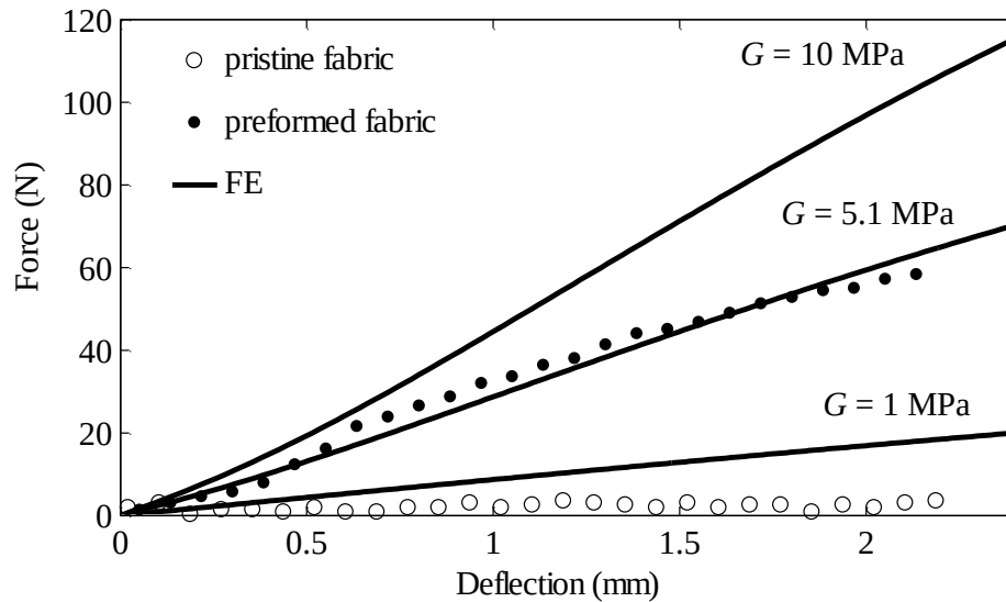
Figure 4-18 : Influence of preforming on the flexural behavior of the reinforcement in three point bending test (fabric oriented at 0^\circ ).
