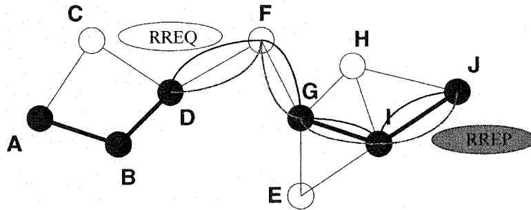
Figure 3.5 Re-routage local
