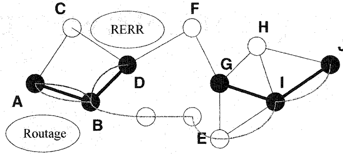
Figure 3.6 Re-routage global
