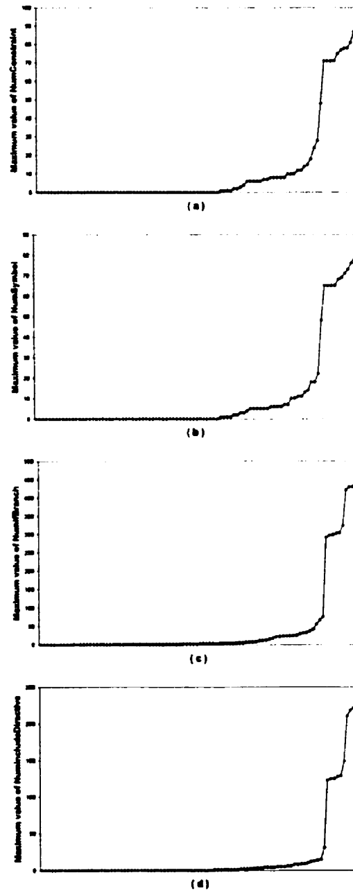
Figure 5.14: Distributions of maximum values of four metrics for individual files, sorted by increasing metrics values
