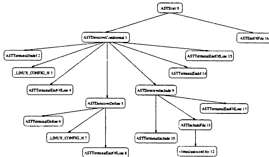
Figure 4.2: A sample AST
