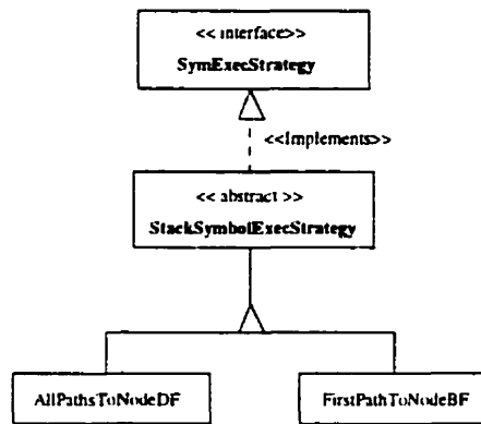
Figure 4.15: Class design of symbolic execution strategy
