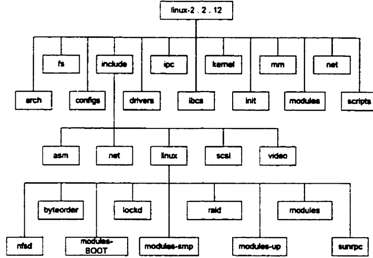
Figure 5.1: Directory structure of linux-2.2.12
