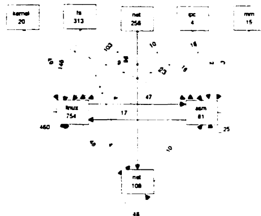
Figure 5.3: Dependence relationship of linux-2.2.12 subdirectories
