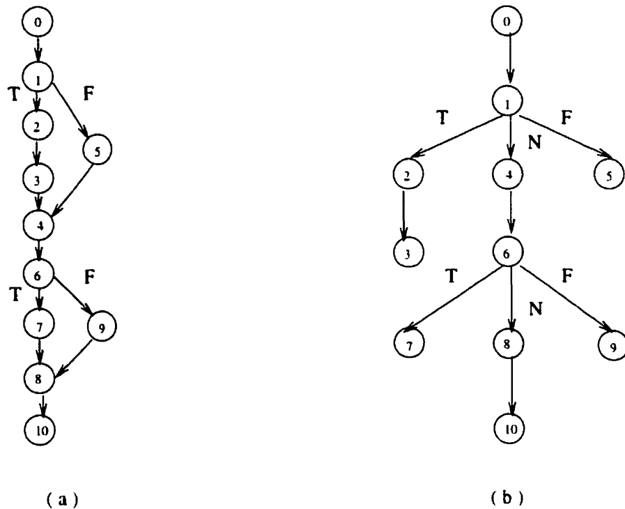
Figure 4.13: CFG example and corresponding dominator tree
