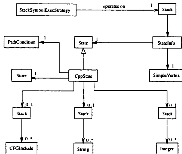
Figure 4.14: Class design of state information
