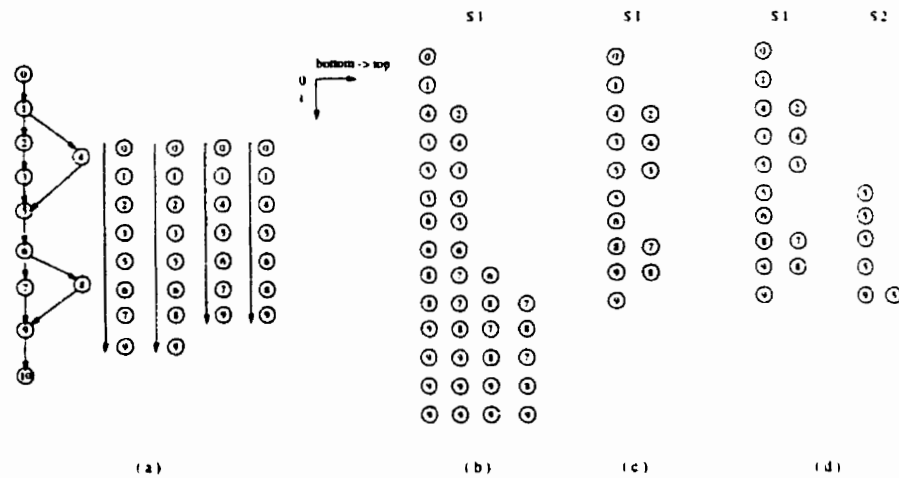
Figure 4.24: Examples of BFS
