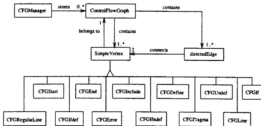
Figure 4.9: Class relationships in control flow graph design
