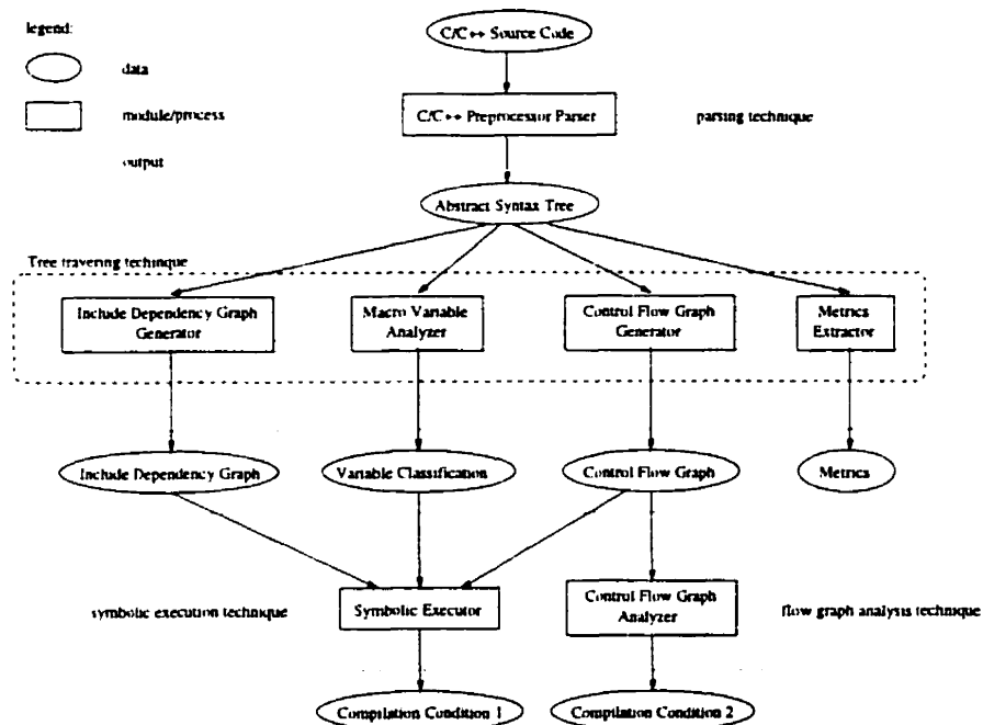
Figure 4.1: System architecture of the tool
