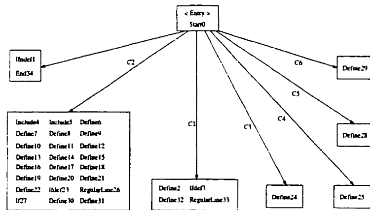
Figure 5.16: Compilation condition graph of kernel.h
