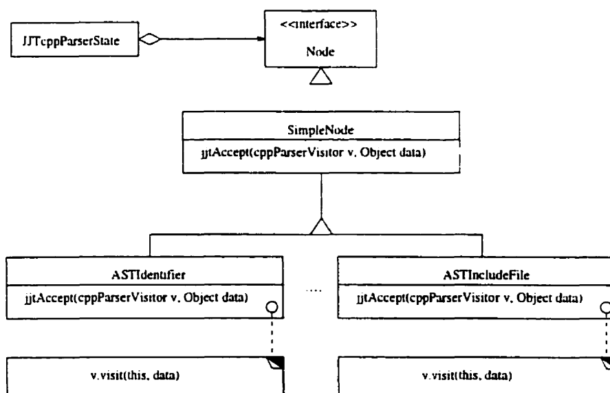
Figure 4.3: AST node hierarchy
