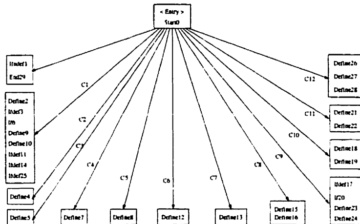
Figure 5.18: Compilation condition graph of linkage.h
