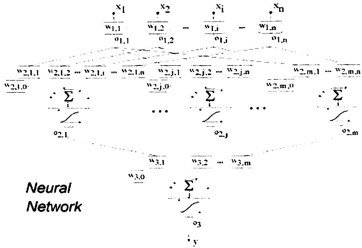
Figure 4.1 Neural Network with three layers
