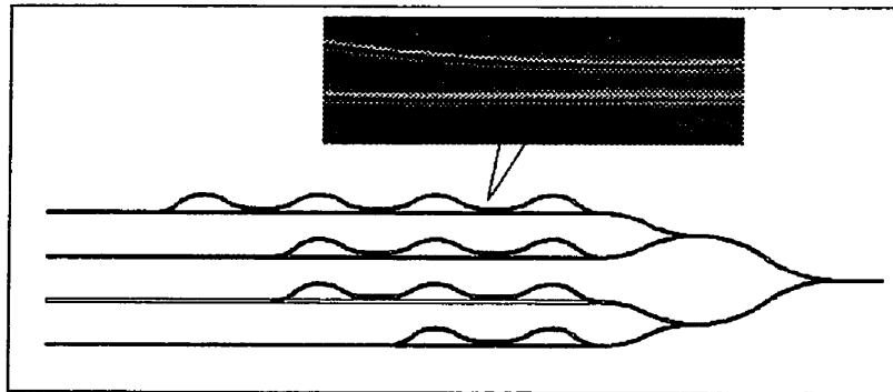
Figure 3.1 Mask pattern of the Mach-Zehnder filter.
