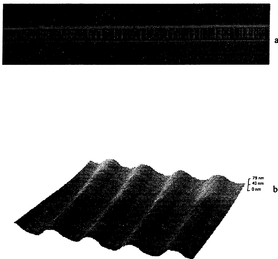
Figure 3.17 (a) Optical microscope photograph of a grating imprinted in sol-gel ridge waveguides. Grating period in 0.5025 \mu\text{m} . (b) Atomic force microscope picture of grating.
