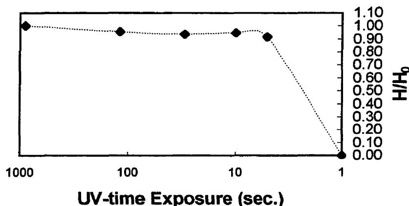
Figure 2.11 Characteristic curve for the hybrid organoaluminosilicate section (nominal composition 85 \text{SiO}_2 -15 \text{Al}_2\text{O}_3 ) showing the ratio H/H_0 as function of exposure time. The exposure time is plotted on a logarithmic scale.
