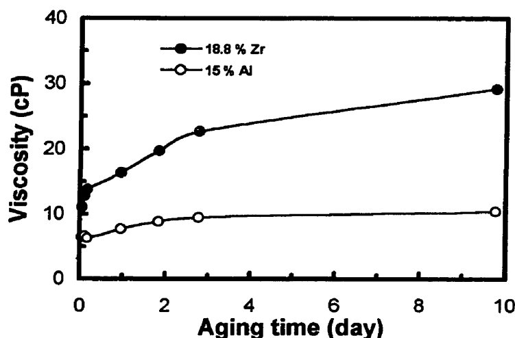
Figure 2.2 Viscosity of (1-x)\text{SiO}_2 - x\text{ZrO}_2 ( x = 18.8 ) and (1-y)\text{SiO}_2 - y\text{Al}_2\text{O}_3 ( y=15 ) sol-gel as a function of aging time.
