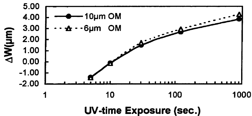
Figure 2.13 Variation of \Delta W (=W_{\max}-W_0) as function of exposure dose. W_{\max} is the maximum width for waveguides cross-section and W_0 is the opening-mask feature width.
