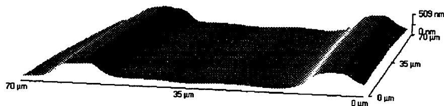
Figure 2.19 Atomic Force Microscopy (AFM) 3-D view of the surface relief waveguide inscribed in an organoaluminophosphate polyglass film. The depressed region distinguishes the densified waveguide structure from the surrounding matrix that has not been exposed to UV light.
