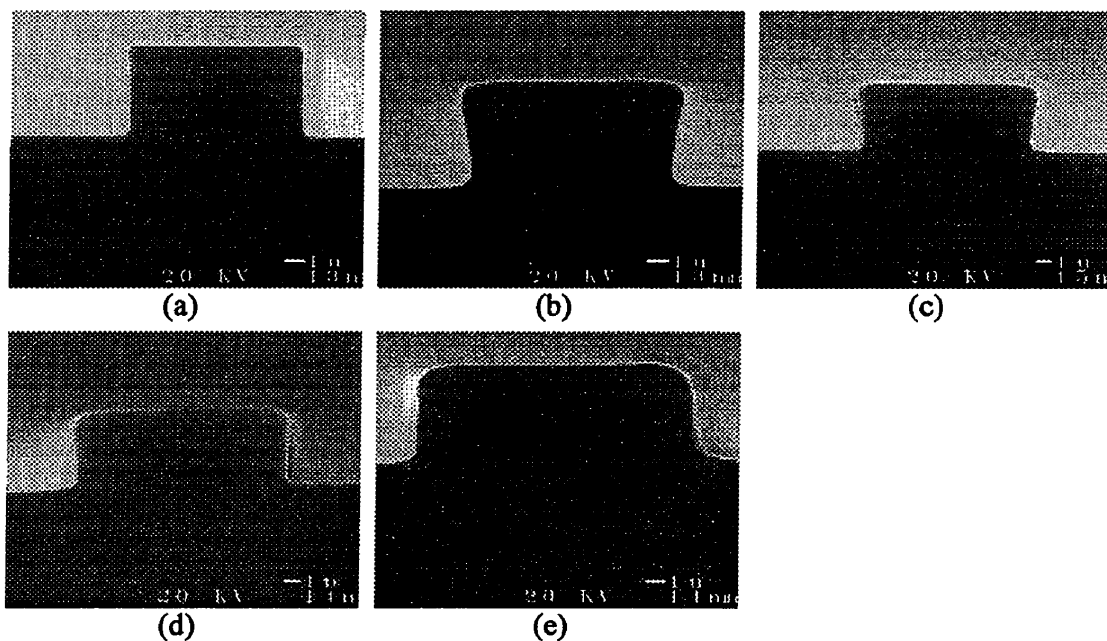
Figure 2.9 SEM image of ridge waveguide cross section (nominal composition 85\text{ SiO}_2\text{-}15\text{ Al}_2\text{O}_3 ) as function of exposure time: (a) 5 sec., (b) 10 sec., (c) 30 sec., (d) 120 sec. and (e) 900 sec. Mask opening = 10\text{ }\mu\text{m} .
