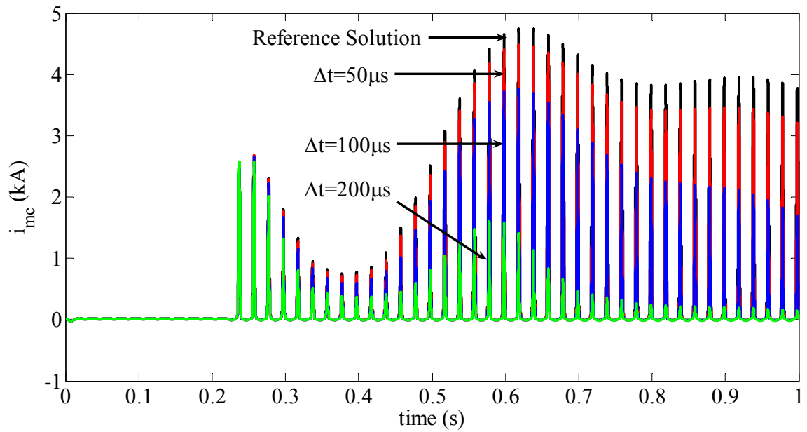
Figure 4.17 Numerical solutions with PD-dq0 model and the reference waveform for phase-c current on transformer magnetizing branch, Test Case C6,
