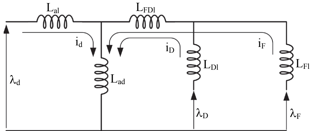
Figure 2.3 d -axis equivalent circuit illustrating flux-current relationship
