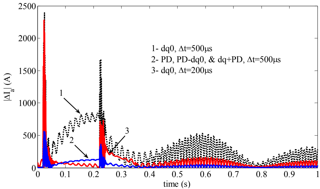
Figure 4.10 Differences between the numerical solutions and the reference waveform for phase-a currents, Test Case C2
