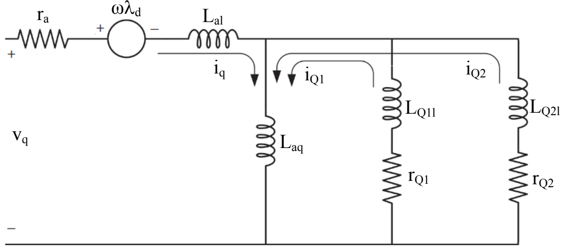
Figure I.2. q -axis equivalent circuit representing the complete characteristic
