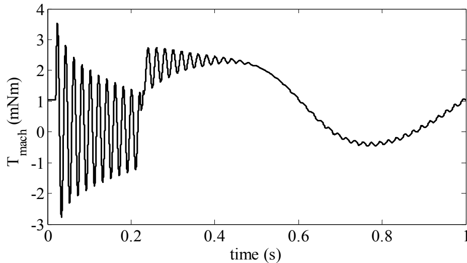
Figure 4.8 Reference waveform for electrical torque, Test Case C1
