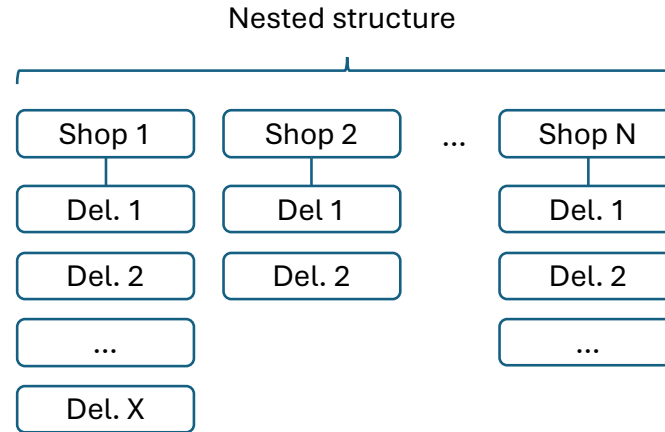
Figure 4.2 Nested structure of the data
