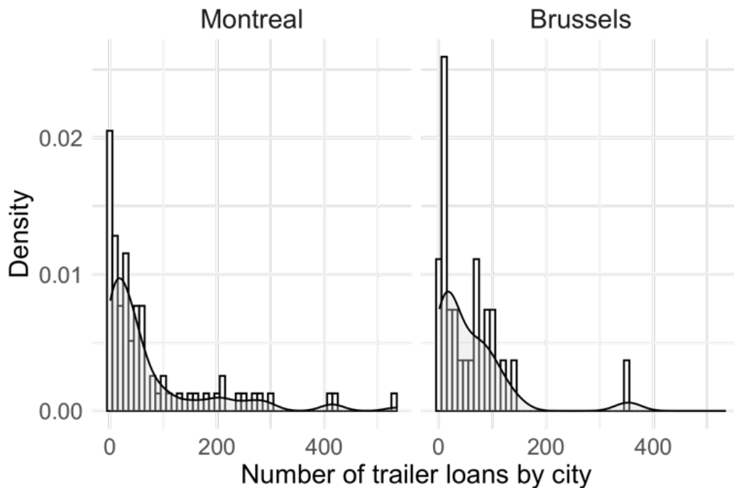
Figure 7.1 Data distribution for Montreal and Brussels
