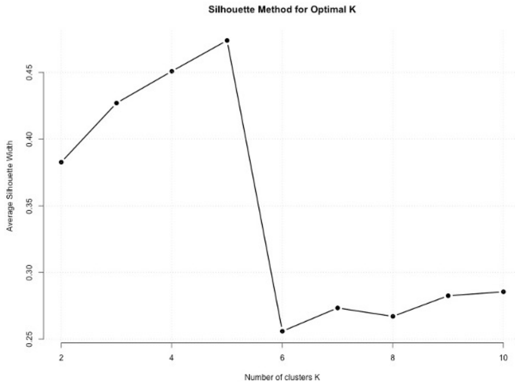
Figure 7.2 Results of the silhouette method
