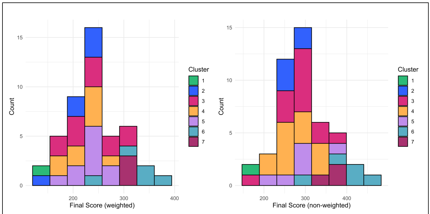
Figure 6.13 Distribution of final scores (i) weighted (left) and (ii) non-weighted (right) by cluster
