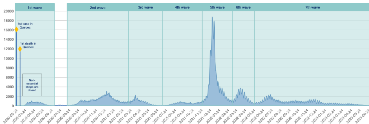
Figure 4.1 Waves of Covid-19 cases for Quebec (Canada)
