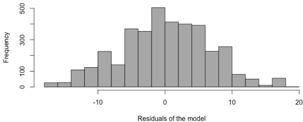
Figure 4.3 Histogram of the residuals of the model
