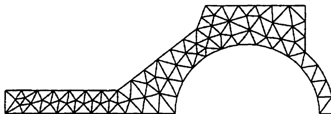
Figure 1.1: FEM meshing of a connecting rod.
