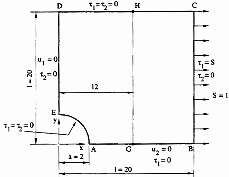
Figure 8: Modeling of Kirsch's problem.
