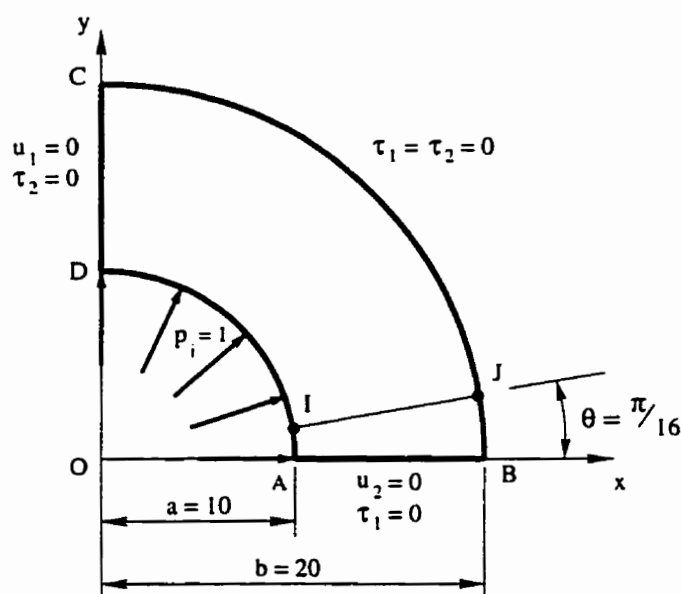
Figure 8: Modeling of Lamé's problem.
