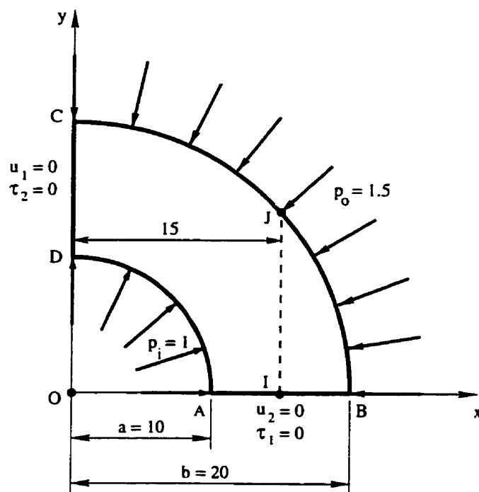
Figure 4: Modeling of Lamé's problem.
