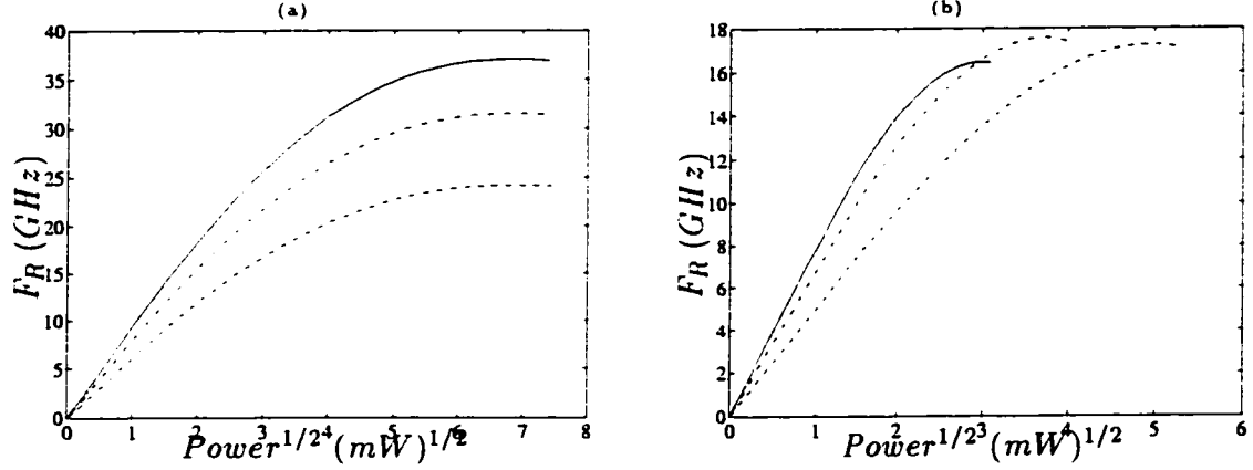
Fig. 14 (a) Length dependency of the gain compression effect on the relaxation oscillation frequency F_R = \Omega_R/2\pi in antiphase gain-coupled DFB laser with a linear gain material, where |K|L = 1 , \alpha_M = 2 , \varepsilon_N = 5 \times 10^{-17} \text{ cm}^{-3} and \gamma = 2/\pi . (b) Length dependency of the gain compression effect on the relaxation oscillation frequency F_R = \Omega_R/2\pi in antiphase gain-coupled DFB laser with logarithmic gain material, where |K|L = 1 , \alpha_M = 3 , \varepsilon_N = 5 \times 10^{-17} \text{ cm}^{-3} and \gamma = 2/\pi . Solid line: L = 250 \mu m ; dot-dashed line: L = 350 \mu m ; dashed line: L = 600 \mu m .
