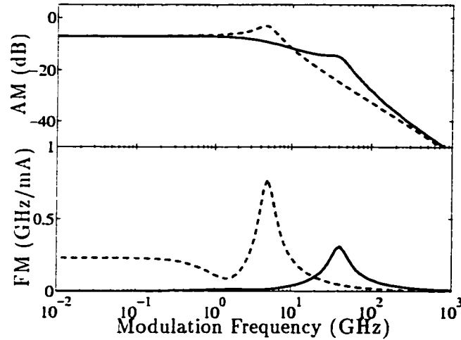
Fig. 4 Comparison of the AM and FM responses between the same DFB device modulated as a single-contact laser (dashed line) or a two-contact push-pull laser (solid line), where |K|L = 6 , L = 600 \mu\text{m} and I_0 = I_{th} + 20 \text{ mA} .
