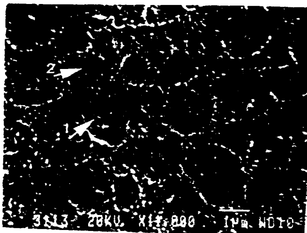
Figure 3.8. Large dimple-like features approximately 2 \mu\text{m} in diameter observed in a PS specimen for \Delta K = 0.84 \text{ MPa}\sqrt{\text{m}} , da/dN = 8 \times 10^{-4} \text{ mm/cycle} and f = 2 \text{ Hz} presenting numerous fine U-shape dimples (arrow 1) with the U-edge pointing towards a region of fine round dimples (arrow 2) near the center of each large dimple-like feature. The macroscopic FCP direction is from bottom to top.
