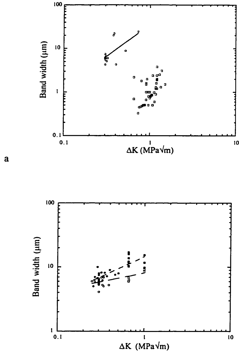
Figure 3.7. Band width (i.e., DGB width and interstriation spacing) plotted against \Delta K on log-log scale at either 0.2, 2 or 20 Hz: a) DGB's (○) and striation-like features (□) observed in PS specimens; b) DGB's (○, ●) and striation-like features (□, ■) observed in 95/5 PS/HDPE and 95/(0.5/4.5) PS/(SEBS/HDPE) specimens (open symbols represent blends without SEBS, closed symbols blends with SEBS). Power law regressions are drawn for DGB's in PS (—) and for the DGB's and striation-like features in compatibilized (---) and noncompatibilized (— —) specimens.
