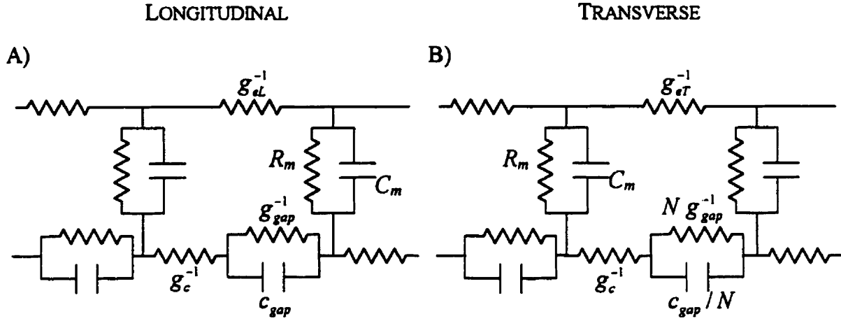
Figure 3.3 Diagram of the intracellular capacitance model. A) Along the fiber direction. B) Transverse to fiber direction. g_c : bidomain cytoplasmic conductivity, g_{gap} : bidomain gap junction conductivity, c_{gap} : bidomain junction capacitance per unit length, N : transverse to longitudinal ratio of junction density.
