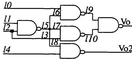
Figure 4.6 A two-output example
