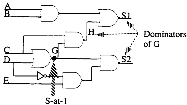
Figure 3.2 A two-output circuit with fault G_{s-a-1} .
