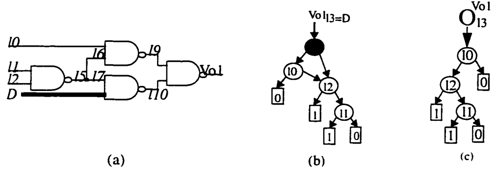
Figure 4.7 (a) circuit Vo1 with l3 = D, (b) the BDD of Vo1, and (c) the observability of l3 at Vo1
