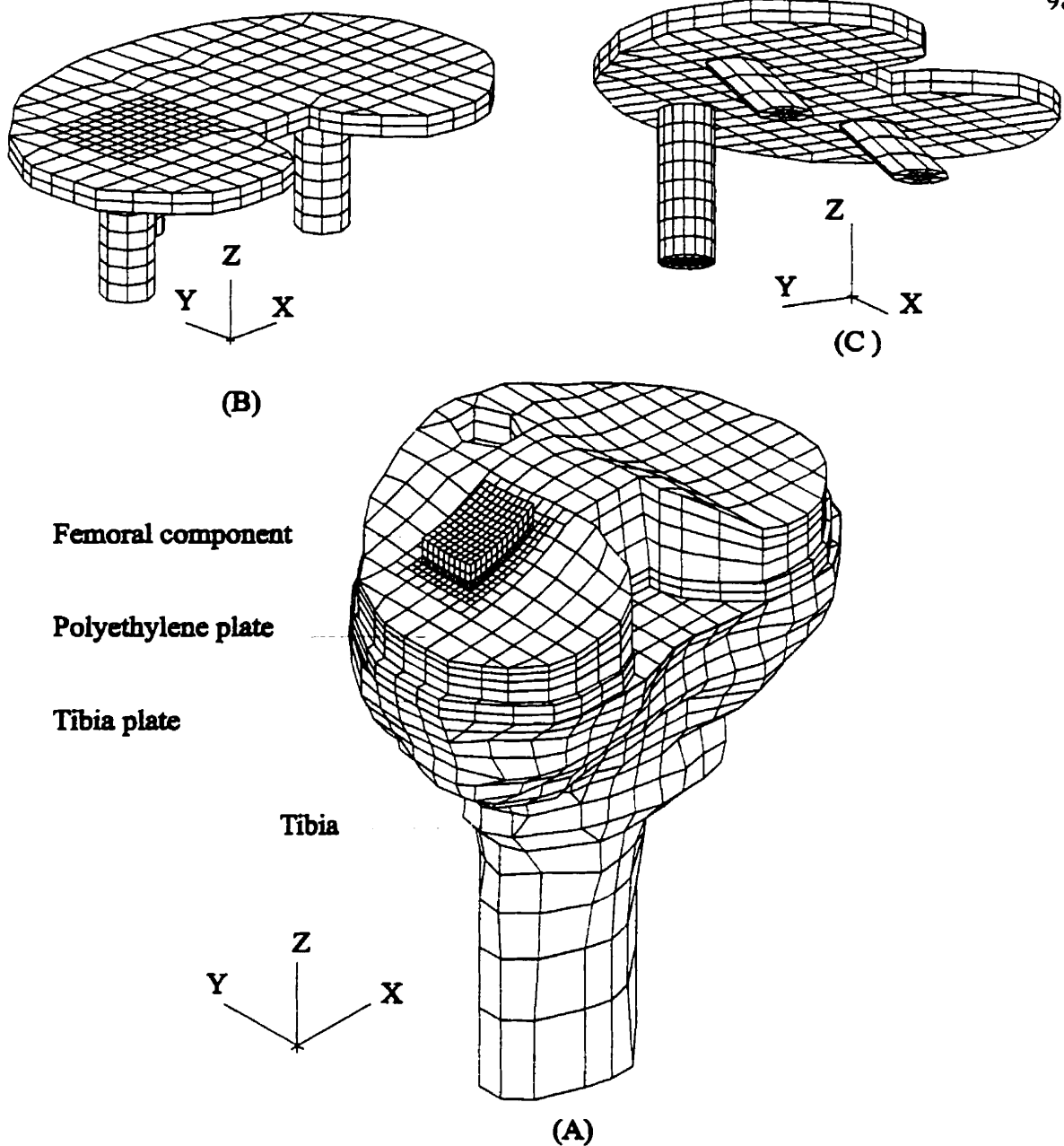
Figure 4.1 Finite element grid used in the study; A) Proximal tibia, metallic baseplate, polyethylene insert and a part of the femoral component used to apply compression, B) tibial baseplate for the design with screws, and C) tibial baseplate for the design with two inclined pegs and one screw at the anterior region. Pegs and screws are modeled as cylinders with interference and friction properties representing their measured pull-out response.
