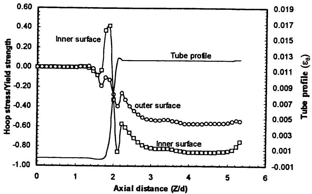
Figure 8.5: Hoop stress and tube deformation profiles after first step of expansion
