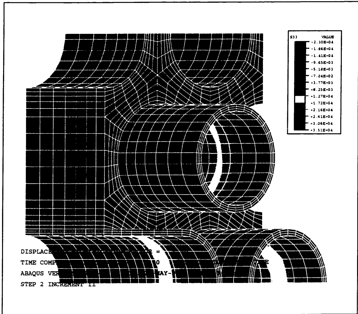
Figure 7.5: 3-D residual axial stress contour on the tubes transition zone
