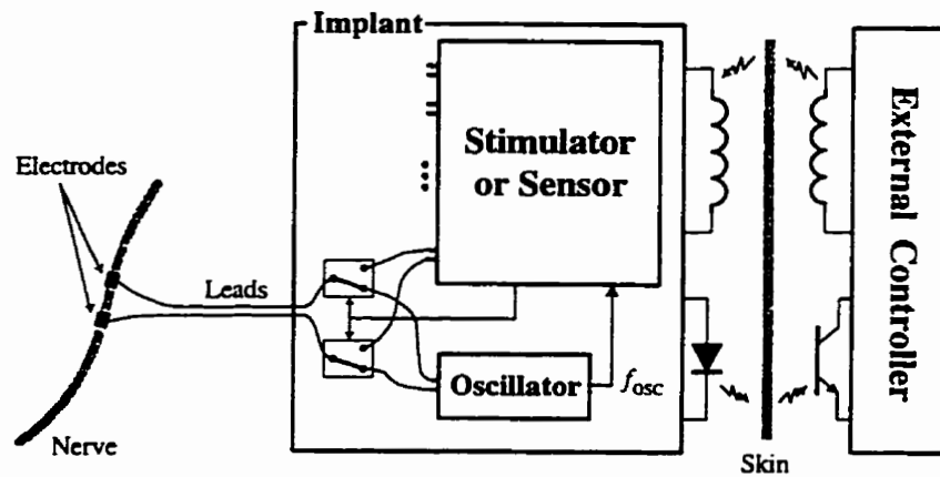
Fig. 3: Simplified block diagram of an implantable stimulator/sensor containing an oscillator to monitor the electrodes and lead failures as well as the living tissue state.
