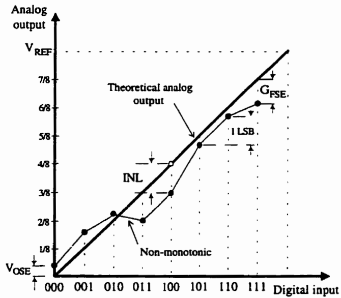
Fig. 1(b): Graphical representation of INL, V_{OSE} , G_{FSE} , and nonmonotonicity for a 3-bit D/A converter.
