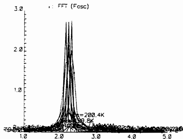
Fig. 16. Fast Fourier transform of the Monte Carlo analysis of the first temperature sensor (DCRTS) output signal.
