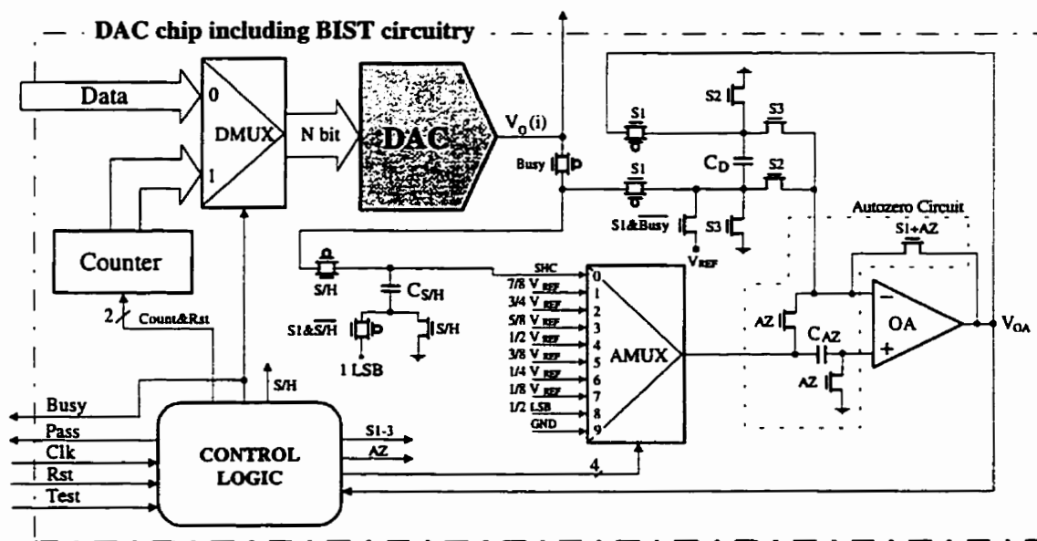
Fig. 2: BIST architecture for D/A converter testing.
