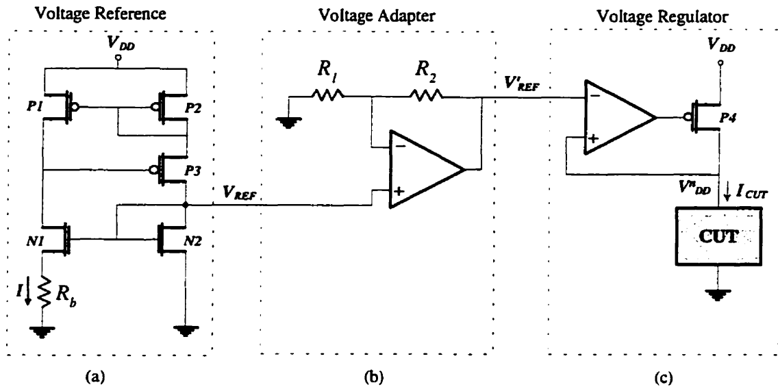
Fig. 1: Circuit schematic of the precision CMOS voltage reference and regulator.
