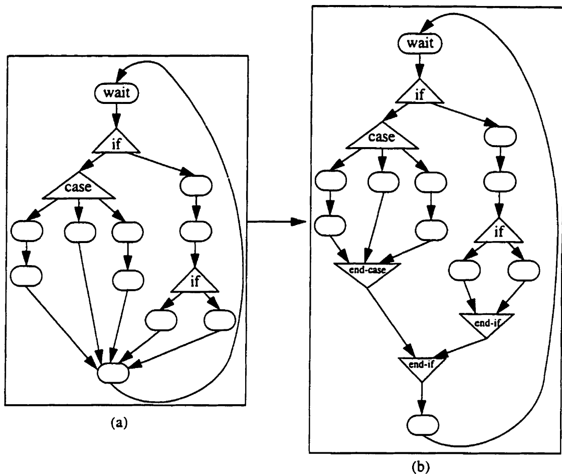
Figure A.2.7 (a) An example of a CDFG without end-statement nodes. (b) example of a modified CDFG including the corresponding end-statements
