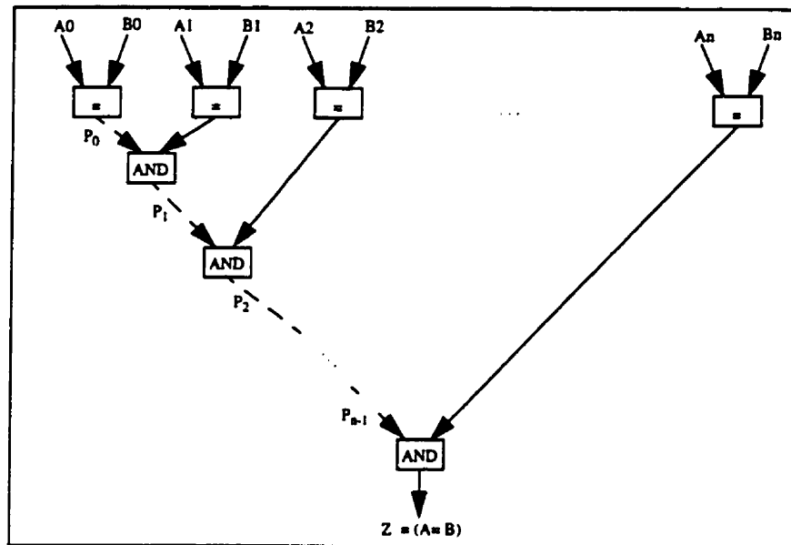
Figure 3.13 The internal signals considered for test-point insertion of an n-bit equality comparator.
