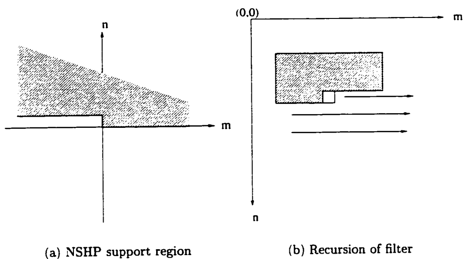
Figure 1.3: NSHP support region and Recursion of filter
