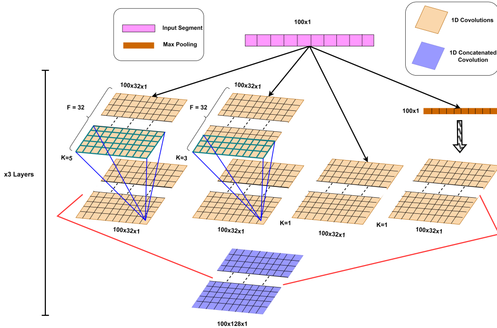
Figure 4. Architecture of the Inception1D block
