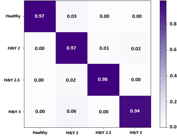
Figure 5. Confusion matrix of InceptoFormer
