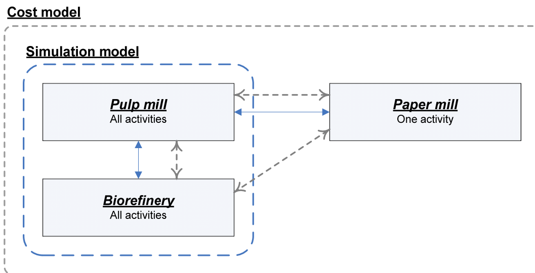
Figure 3. Structure of the modelling framework in the case study. Solid blue lines denote flow of material and energy, dashed grey lines flow of costs.
