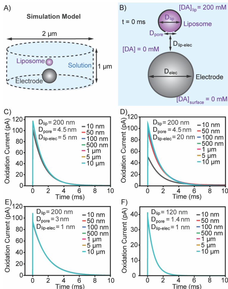
Figure S4. Prediction of amperometric current spikes generated by DA release from individual liposomes at the electrode surface. (A) Schematic of the simulation model: A buffer solution (blue cylinder) containing a single liposome (purple sphere) and an electrode (gray sphere) aligned along the vertical axis. (B) Initial state ( t = 0\ \text{ms} ): A liposome with diameter D_{\text{lip}} is filled with 200\ \text{mM} DA, surrounded by a DA-free buffer. The liposome membrane (black arc) is impermeable except for a membrane pore with diameter D_{\text{pore}} . The dopamine concentration [\text{DA}] at the electrode surface is initially set to 0\ \text{mM} . (C, D) Predicted amperometric current spikes following rupture of a 200\ \text{nm} liposome containing 200\ \text{mM} DA at varying cylindrical electrode diameters ( 10\ \text{nm} -
