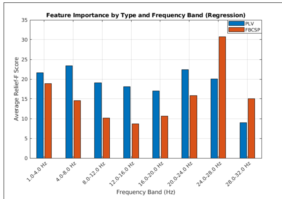
Figure 5. The bar plot displays the average ReliefF score for phase-locking value (PLV) and FBCSP features across eight frequency bands. Higher ReliefF scores indicate greater feature importance for the regression model.
