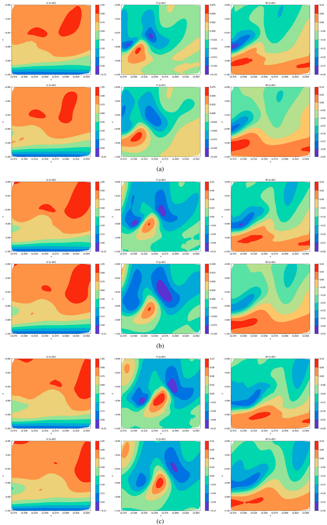
Fig. 13. 3D turbulent channel (Problem 4): Velocity contours at z_{\text{constant}} = 4.69 . (a) Top: reference solution at t = 0 ; bottom: TSA-PINN at t = 0 ; (b) Top: reference at t = 5 \times 0.0065 ; bottom: TSA-PINN at t = 5 \times 0.0065 ; (c) Top: reference at t = 10 \times 0.0065 ; bottom: TSA-PINN at t = 10 \times 0.0065 .
