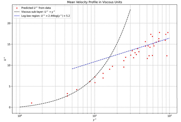
Fig. 14. 3D turbulent channel (Problem 4): Mean velocity profile in viscous units. Standard values of k = 0.41 and B = 5.2 are used in the log-law for reference.
