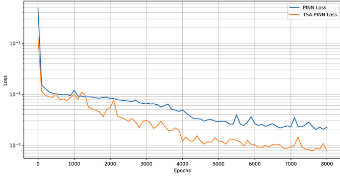
Fig. 2. Lid-driven cavity problem at Re = 100 : Comparison of loss decays.
