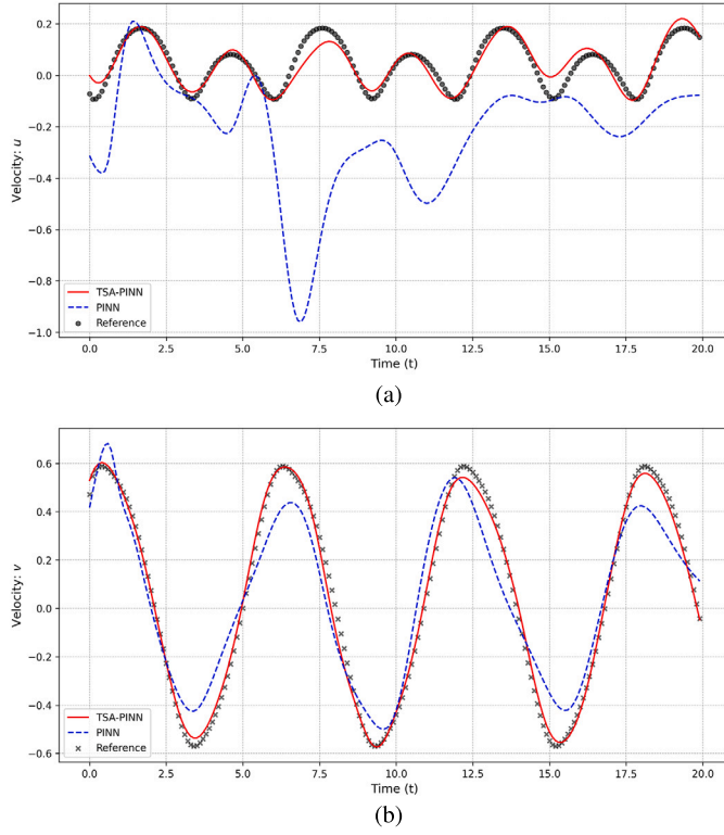
Fig. 11. Cylinder wake problem: Quantitative comparison of the solutions at x = 2.0 , y = 0.04 . (a) u vs. t ; (b) v vs. t .
