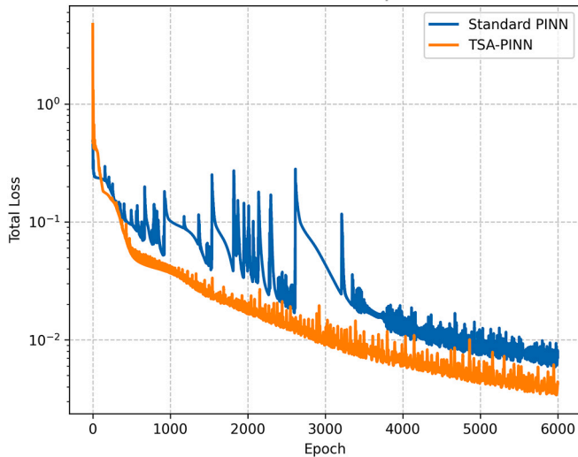
Fig. 7. Lid-driven cavity problem at Re = 3200 : Comparison of loss histories.
