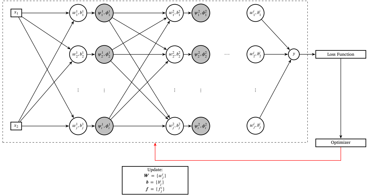
Fig. 1. Schematics of the TSA-PINN. The white circles represent the multiplication of weights and the addition of biases. The gray circles indicate the application of activation functions. (For interpretation of the colors in the figure(s), the reader is referred to the web version of this article.)
