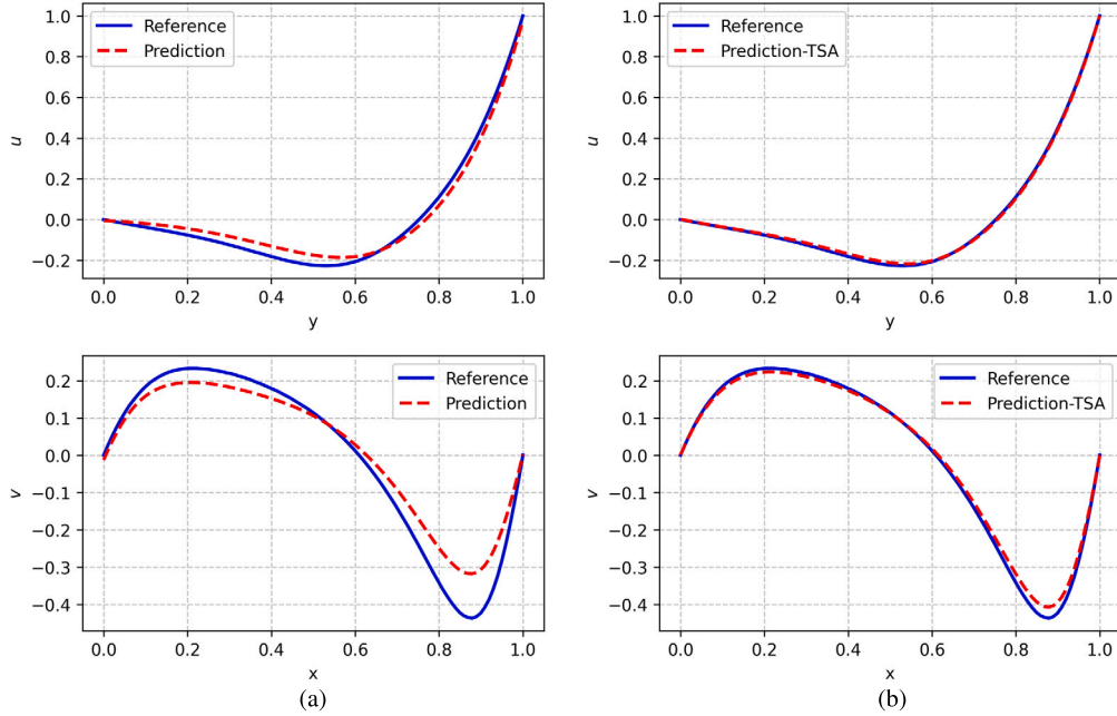
Fig. 4. Lid-driven cavity problem at Re = 100 : Quantitative comparison of the solutions at x_{\text{constant}} = 0.7 and y_{\text{constant}} = 0.7 . (a) Standard PINN; (b) TSA-PINN.
