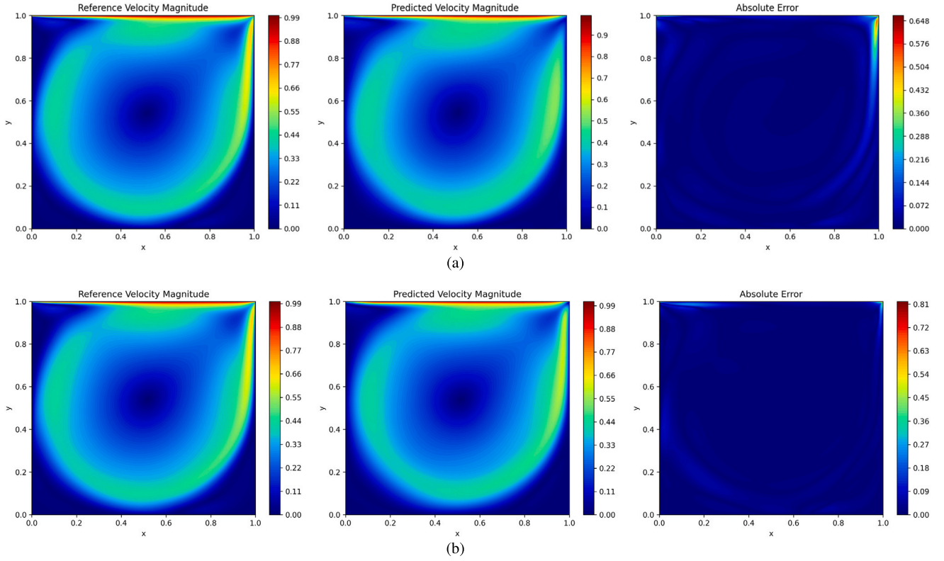
Fig. 5. Lid-driven cavity problem at Re = 3200 : Velocity contours and approximation error. (a) Standard PINN; (b) TSA-PINN.
