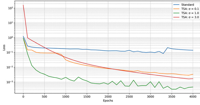
Fig. 8. Cylinder wake problem: Comparison of the loss history.
