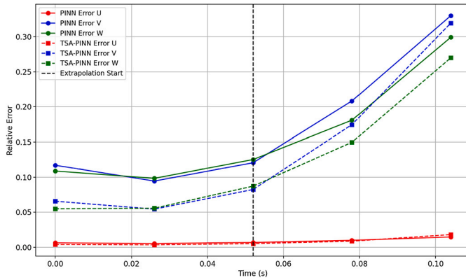
Fig. 16. 3D turbulent channel (Problem 5): Comparison of the error history.
