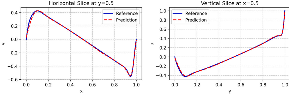
Fig. 6. Lid-driven cavity problem at Re = 3200 : Quantitative validation of the solution approximations at x_{\text{constant}} = 0.5 and y_{\text{constant}} = 0.5 .
