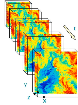
Fig. 12. Schematics of the 3D turbulent channel flow problem [52–54] from https://turbulence.pha.jhu.edu .
