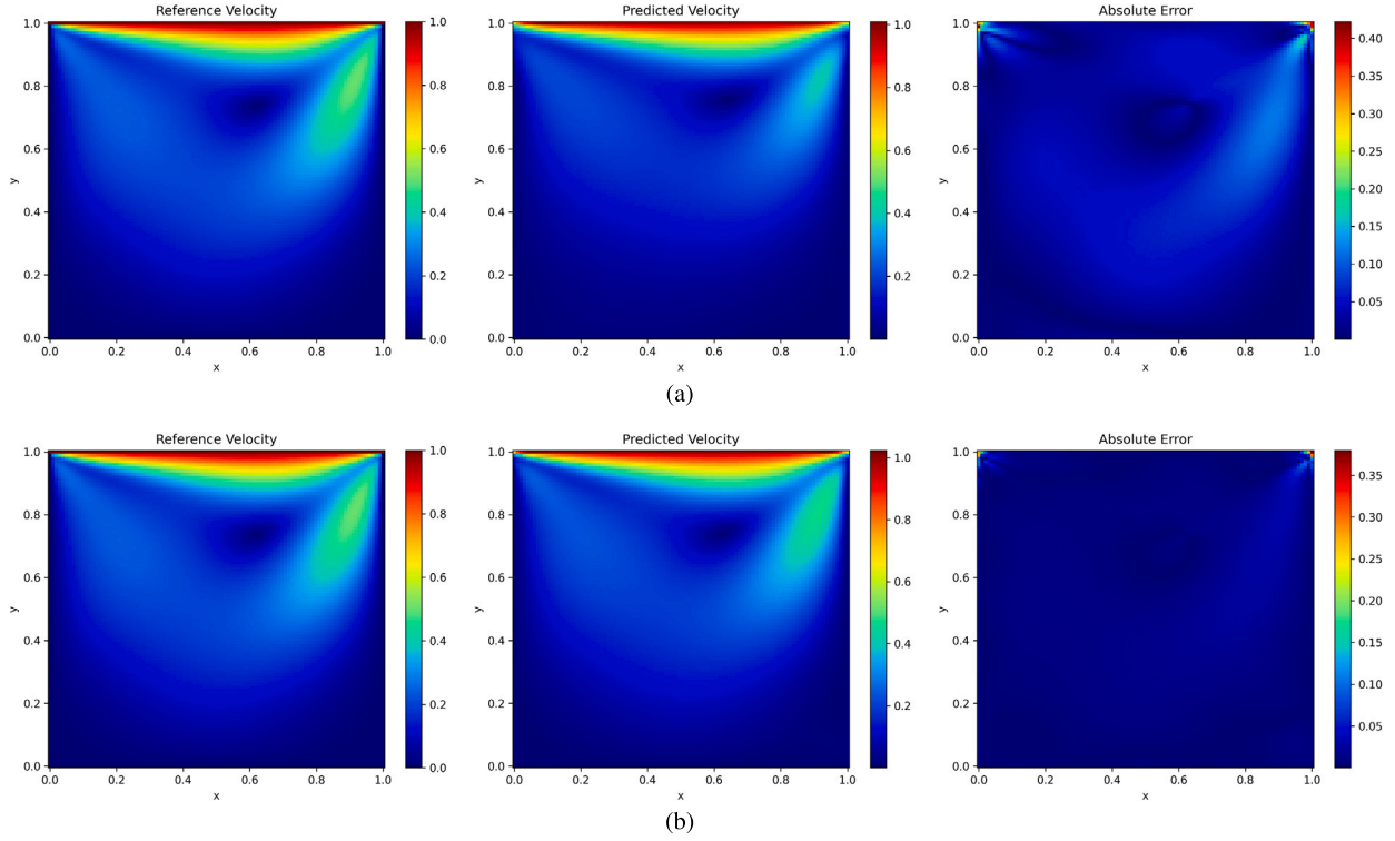
Fig. 3. Lid-driven cavity problem at Re = 100 : Velocity contours and approximation error. (a) Standard PINN; (b) TSA-PINN.
