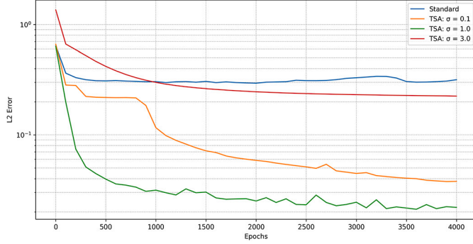
Fig. 9. Cylinder wake problem: Comparison of the error history.
