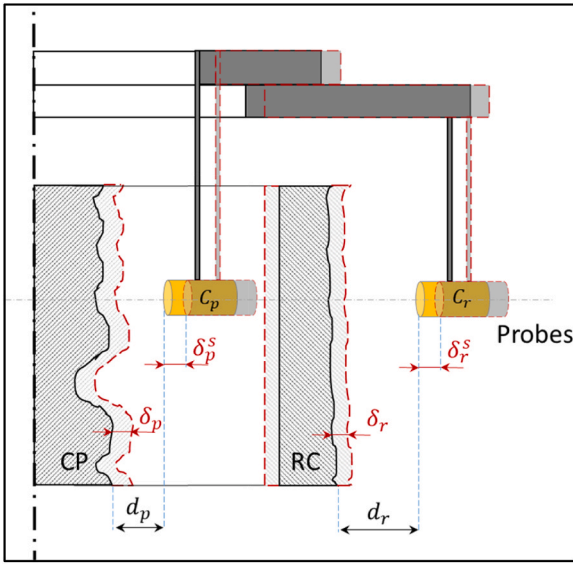
Fig. 13. Schematic of the symmetric configuration of the NanoCyl measuring elements (sensors and carriage structure). The expanded components are represented in red colour. RC=Reference Cylinder.
