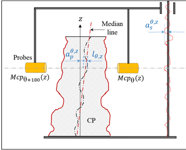
Fig. 10. Opposite probes for radial deviations detection.
