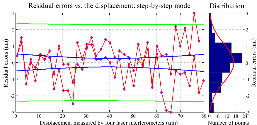
Fig. 7. Step by step calibration of one capacitive probe, third-order polynomial fitting model.
