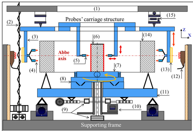
Fig. 4. Architecture of the primary NanoCyl applying the Precision Design Principles [15]: (1) XY translation table, (2) linear guidance, (3) metrology frame, (4) reference probes, (5) measuring probes, (6) cylindrical part, (7) automated tilt/centre table, (8) rotary indexing table, (9) encoders, (10) brake, (11) rotary table, (12) laser interferometers, (13) reflective mirror, (14) reference cylinder, (15) piezoelectric actuators.
