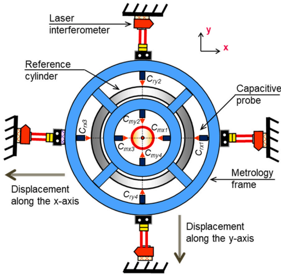
Fig. 6. Calibration of Capacitive Probes using laser interferometers [15].
