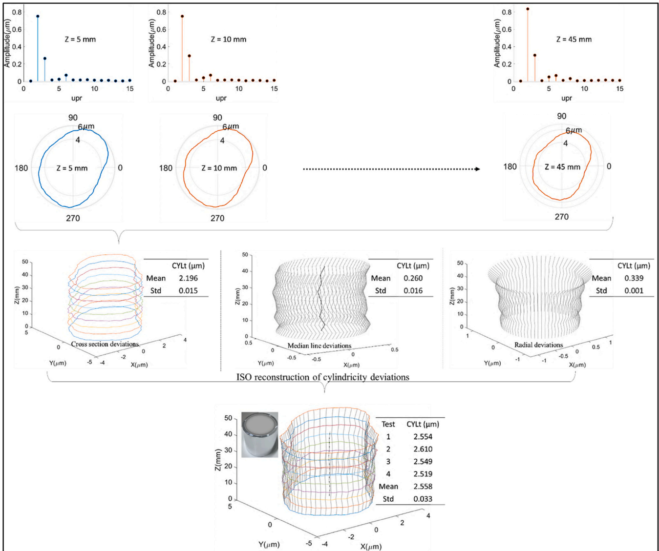
Fig. 12. Cylindricity calibration of the selected high-quality CP including the three simple elements with respect to ISO 12180.
