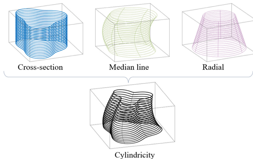
Fig. 2. Elements of cylindricity deviations as defined in ISO 12180–1 [6].
