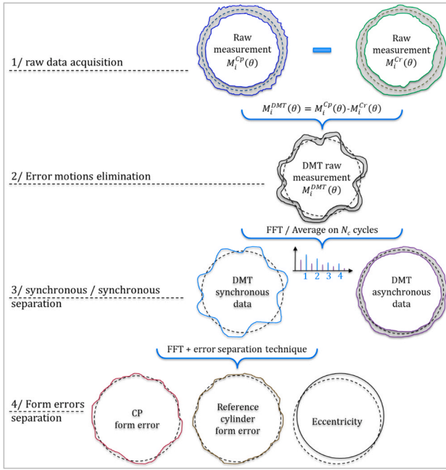
Fig. 8. Schematic diagram of the processing strategy.
