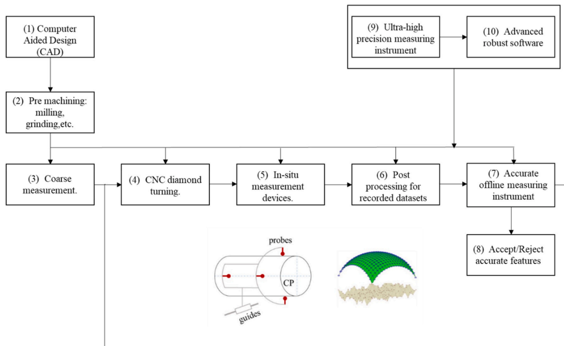
Fig. 1. Iterative process chain for ultra-accurate manufacturing.
