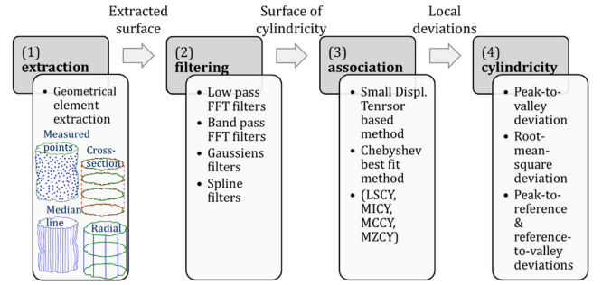
Fig. 11. Implemented strategy for evaluating the cylindricity, including the extraction and combination of the three elements (cross-section deviations, median line and radial deviations).
