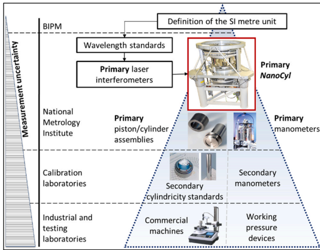
Fig. 3. Established traceability for cylindricity measurements for piston-cylinder assemblies and material CP transfer standards.
