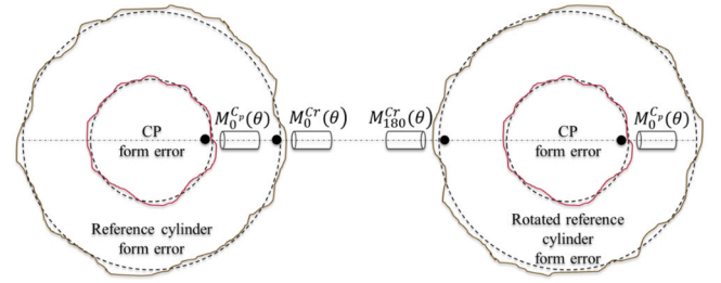
Fig. 9. Revisiting reversal error separation technique. M_0^{CP} and M_{180}^{CP} in the above text.
