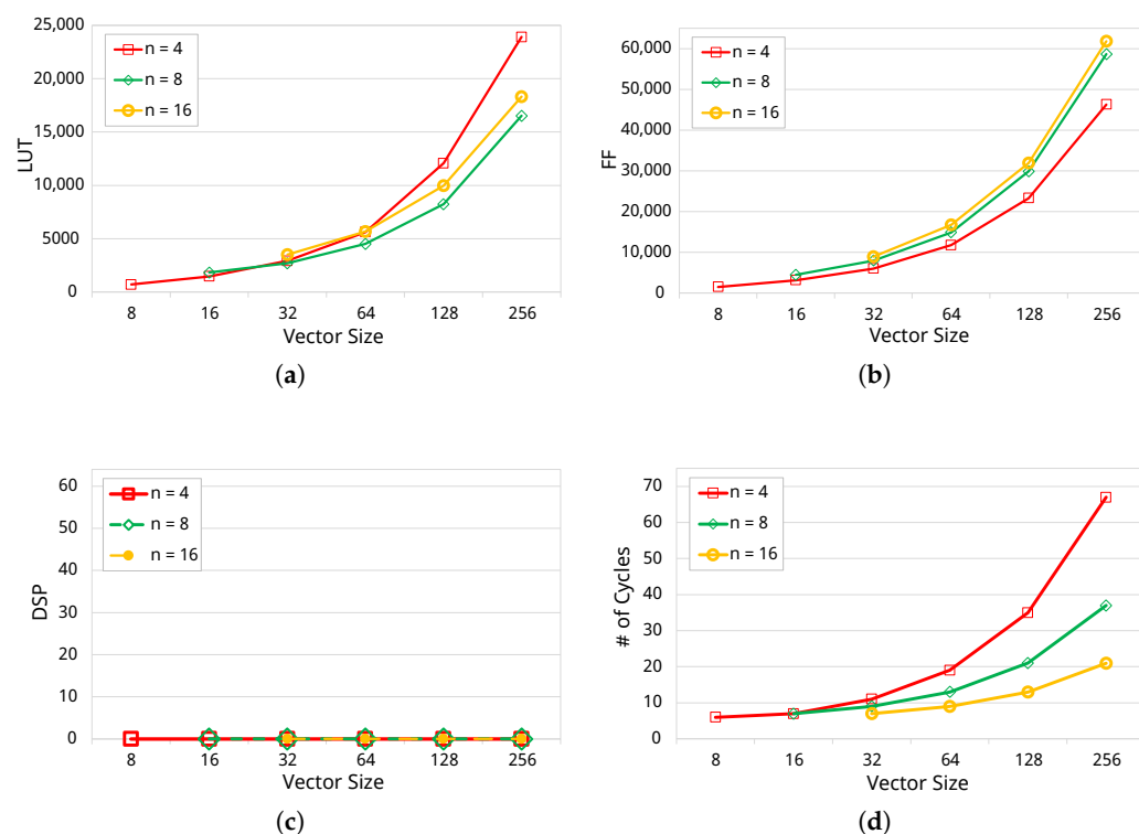
Figure 6. Comparing the resource utilization of vsum operation for different n (4, 8, 16); (a) LUT Utilization; (b) FF Utilization; (c) DSP Utilization; (d) Number of clock cycles.
