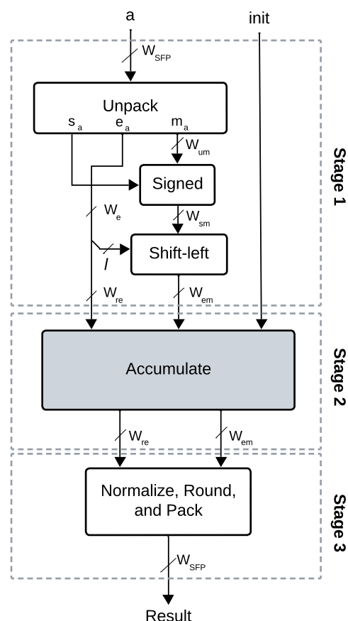
Figure 2. Main stages of a SAT-based accumulator [5].
