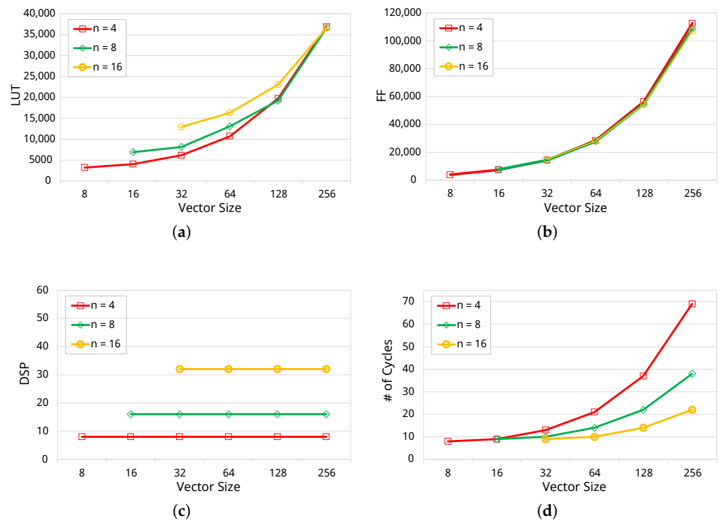
Figure 7. Comparing the resource utilization of dp operation for different n (4, 8, 16); (a) LUT utilization; (b) FF utilization; (c) DSP utilization; (d) number of clock cycles.
