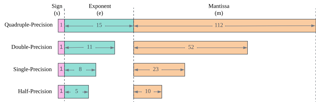
Figure 1. Several precision levels of IEEE-754 standard.
