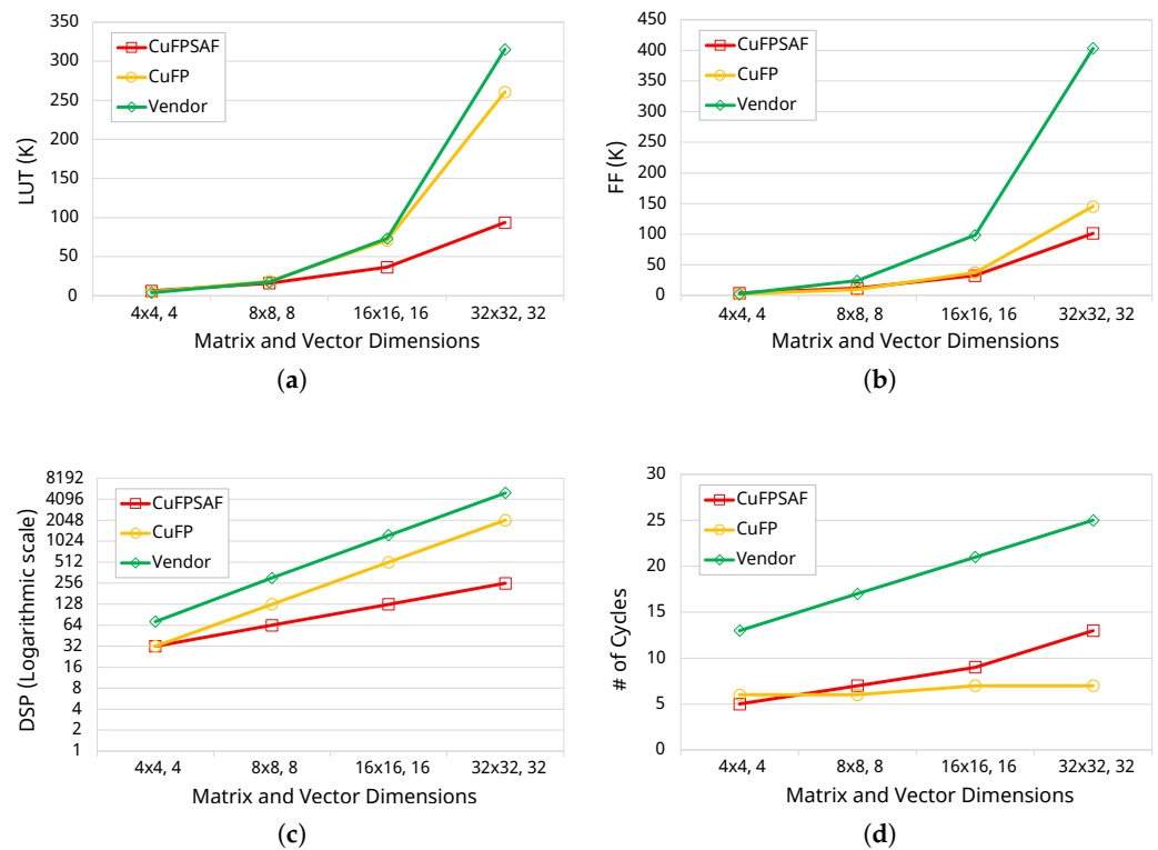
Figure 8. Comparing the resource utilization of mvm operation for different matrix and vector dimensions; (a) LUT Utilization; (b) FF Utilization; (c) DSP Utilization (Logarithmic scale); (d) Number of clock cycles. The x-axis represents the matrix and vector dimensions, where, for example, “ 4 \times 4, 4 ” denotes a 4 \times 4 matrix multiplied by a 4 \times 1 vector.
