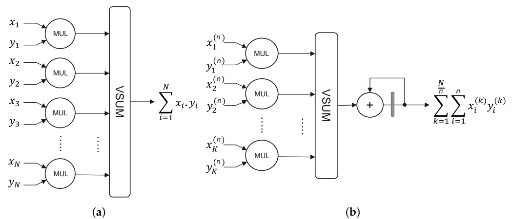
Figure 4. Dot product design: (a) Latency-Constrained approach; (b) Resource-Constrained approach. The grey line stands for register level.
