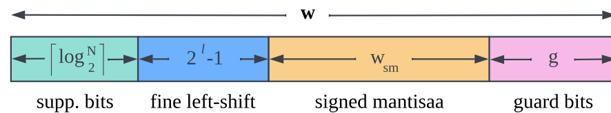
Figure 3. Extended mantissa composition in SAF [5].
