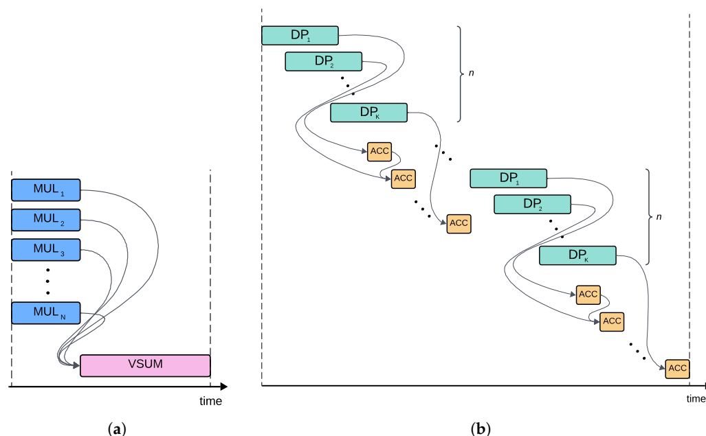
Figure 5. Schedule viewer: (a) Latency-Constrained approach; (b) Resource-Constrained approach. Arrows indicate the data dependencies between operations.
