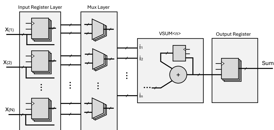
Figure 9. Input operand scheduling for vsum operation with the RC approach.
