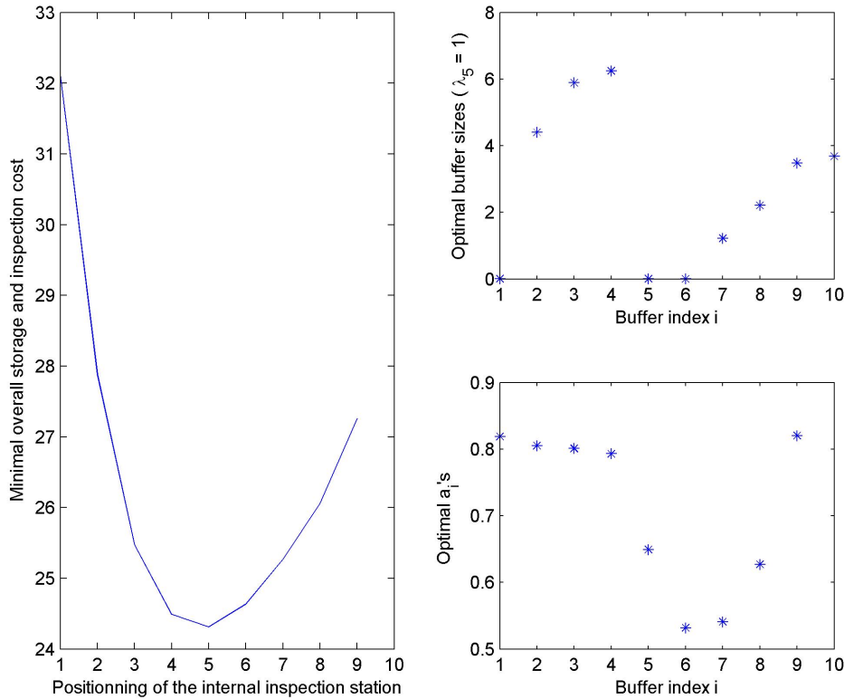
Figure 5.3 The optimal solution.
