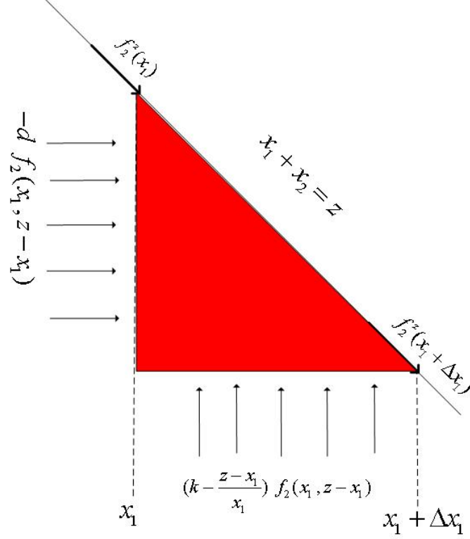
Figure 4.7 Boundary x_1 + x_2 = z in mode 2.
