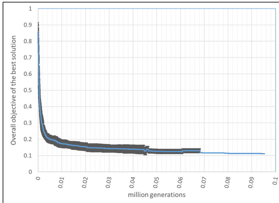
Figure 5.7 Convergence graph of the genetic algorithm
