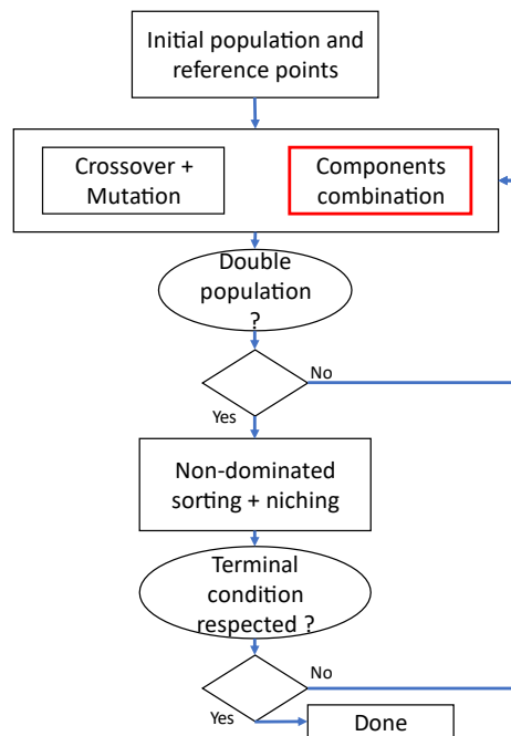
Figure 7.2 Overview of the modified NSGA-III algorithm. The red square represents the added operator.
