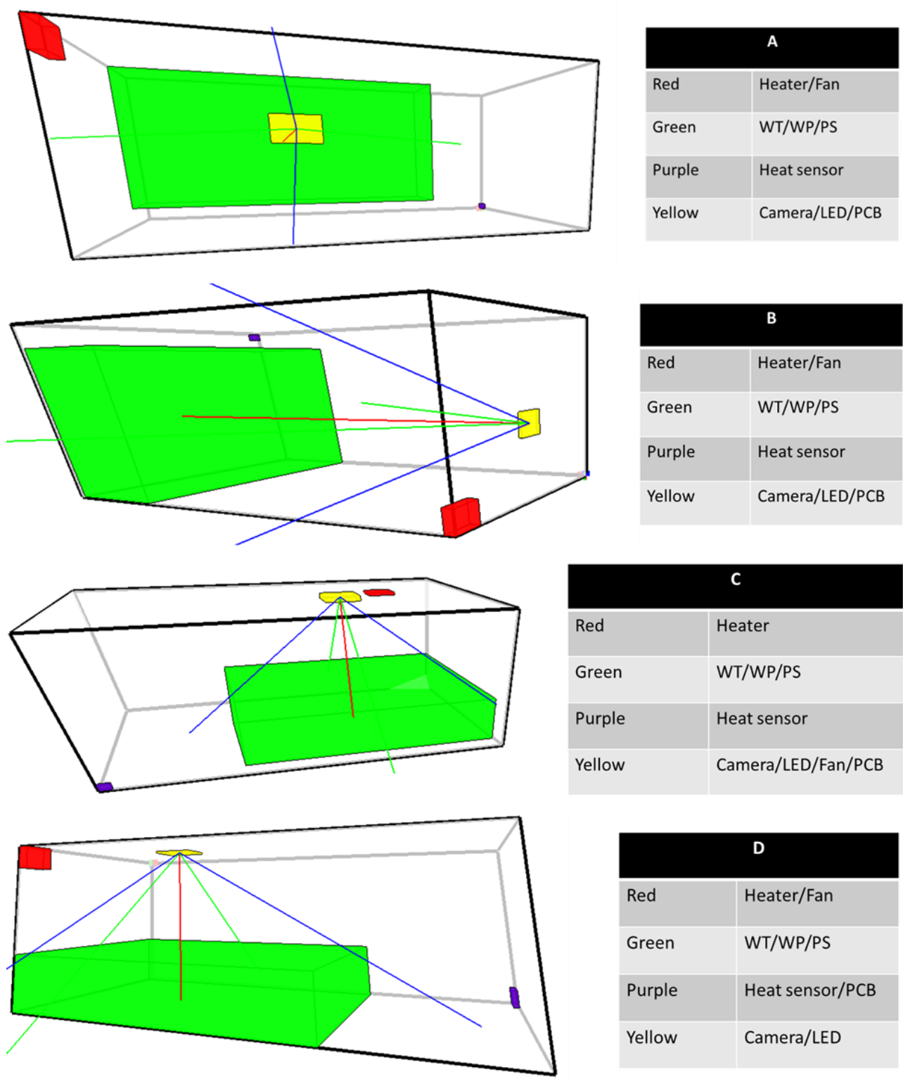
Figure 7.9 Examples of highly modular layouts
