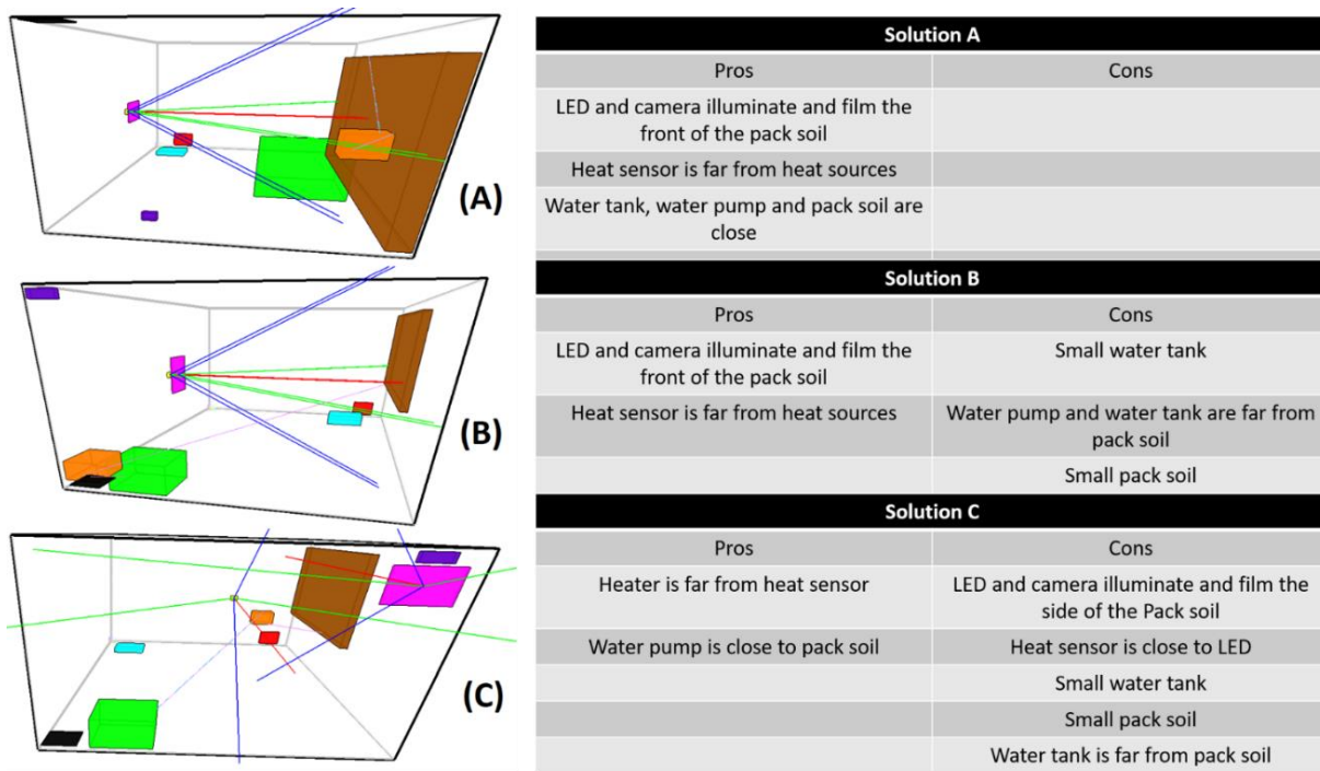
Figure 6.6 Solutions without objective aggregation: (a) good (b) fair (c) mediocre
