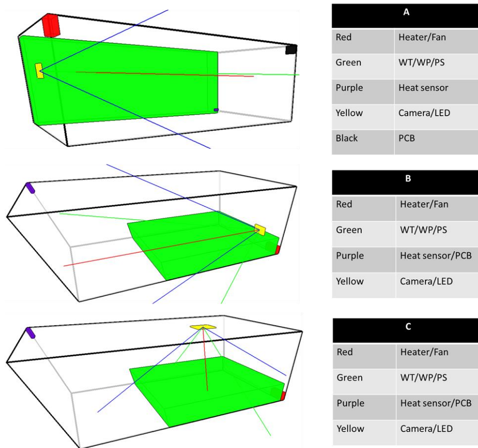
Figure 7.12 Examples of inadequate layouts
