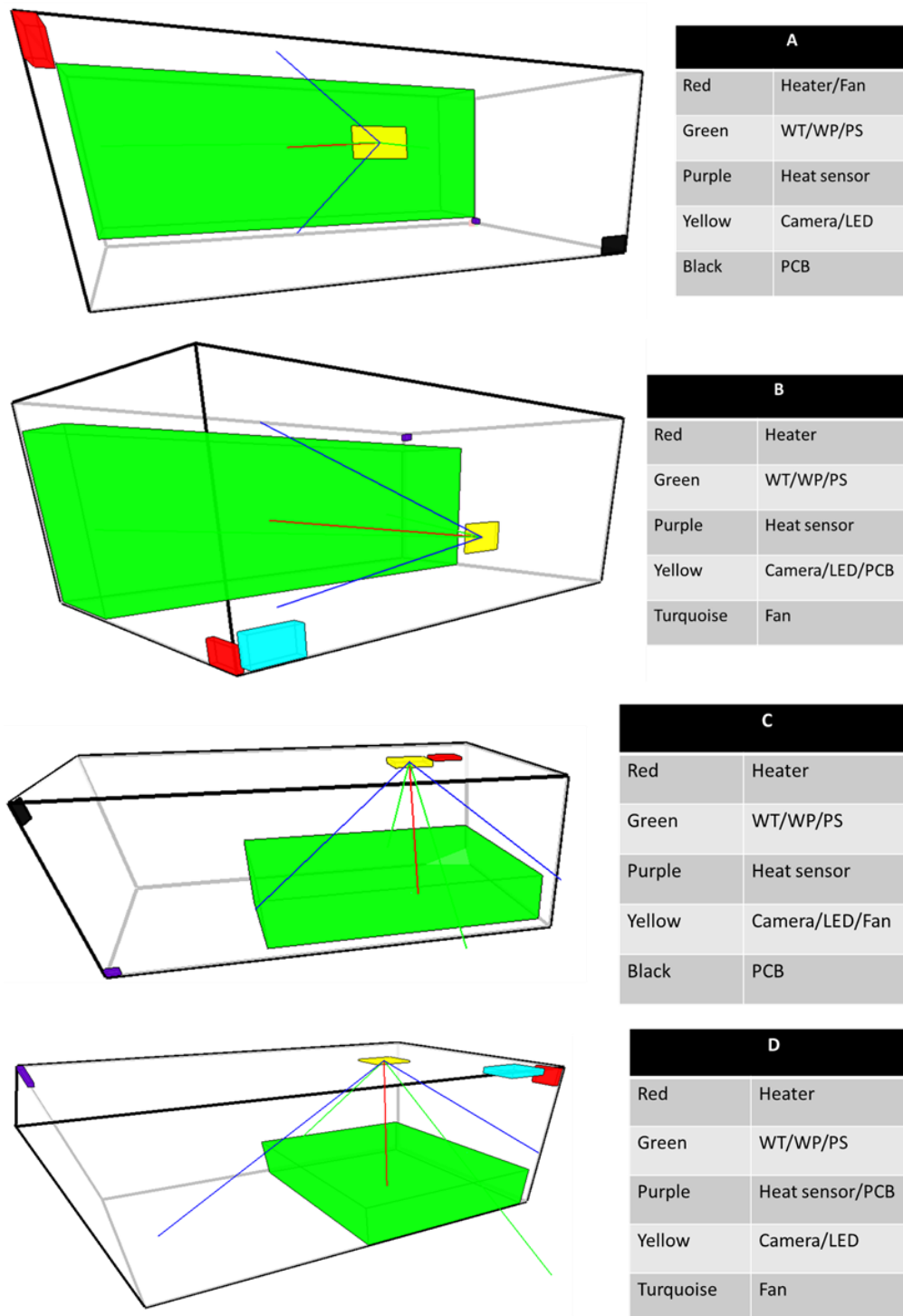
Figure 7.10 Examples of moderate modular layouts
