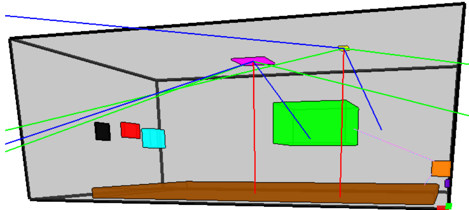
Figure 5.8 Layout optimization of the greenhouse (Side view)
