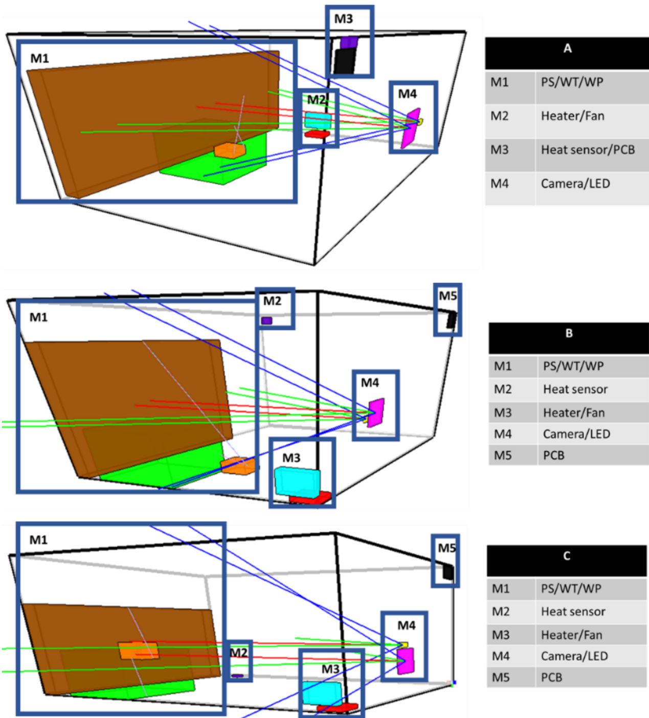
Figure 7.8 Examples of layouts are generated without modularization. Highlighting the possible modules.
