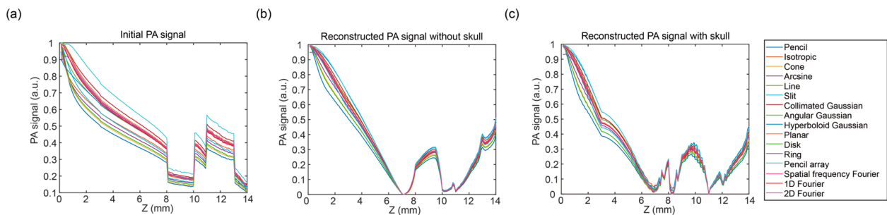
Figure 6. PA signals in the Z direction ( x = 7 mm) under the illumination of sixteen optical source types. (a) Initial PA signal, (b) reconstructed PA signal without the skull, and (c) reconstructed PA signal with the skull.
