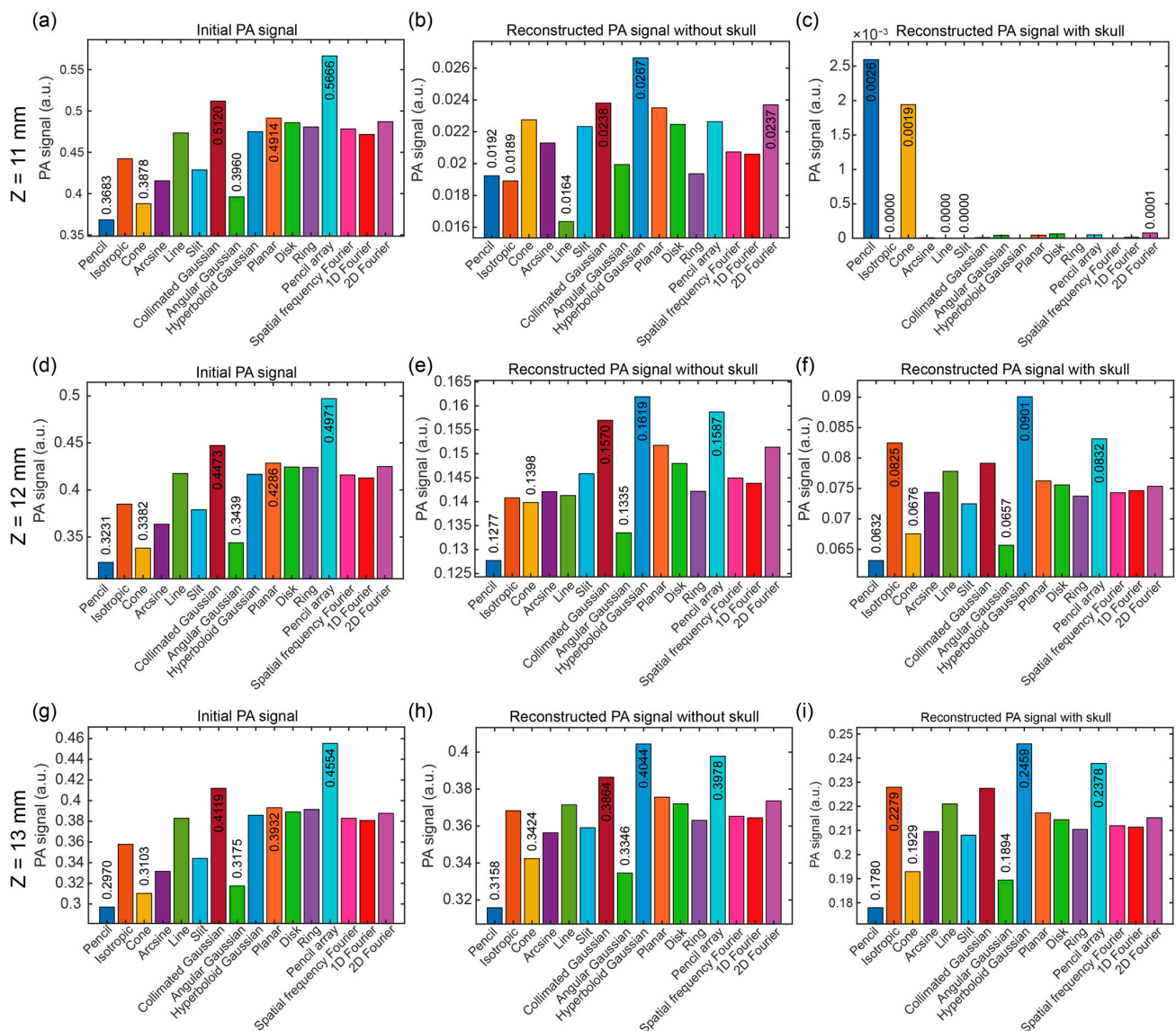
Figure 8. Maximum and minimum PA signals and corresponding optical source types at the specific position ( x = 7 mm, z = 11 , 12, and 13 mm) under the illumination of sixteen optical source types. In the X direction at z = 11 mm, (a–c): (a) initial PA signal, (b) reconstructed PA signal without the skull, and (c) reconstructed PA signal with the skull; in the X direction at z = 12 mm, (d–f): (d) initial PA signal, (e) reconstructed PA signal without the skull, and (f) reconstructed PA signal with the skull; in the X direction at z = 13 mm, (g–i): (g) initial PA signal, (h) reconstructed PA signal without the skull, and (i) reconstructed PA signal with the skull. The data of the first three maximum and the first three minimum PA signals were noted around the bars in the subfigures (a–i).
