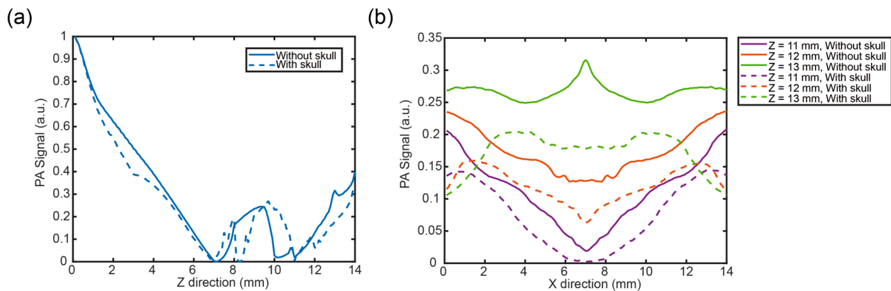
Figure 5. PA signals of reconstructed images without the skull or with the skull under the illumination of a pencil beam. (a) Z direction at x = 7 mm; (b) X direction at z = 11 mm, 12 mm, and 13 mm.
