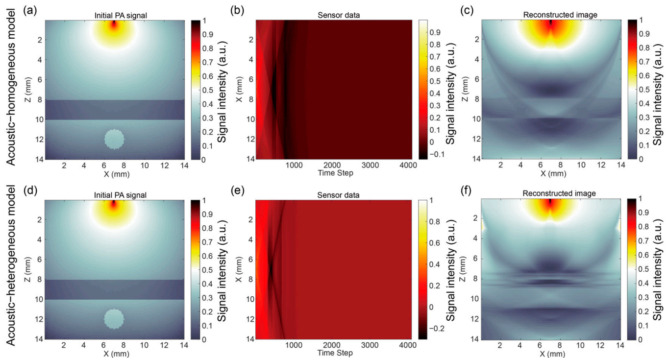
Figure 4. Simulation and reconstruction results of multi-layer brain tissues embedded with blood vessels under the illumination of a pencil beam. Homogeneity of acoustic properties without considering the skull in (a–c): (a) initial PA signal from optical simulation, (b) sensor data from acoustic simulation, and (c) reconstructed image; heterogeneity of acoustic properties considering of skull (d–f): (d) initial PA signal from optical simulation, (e) sensor data from acoustic simulation, and (f) reconstructed image.
