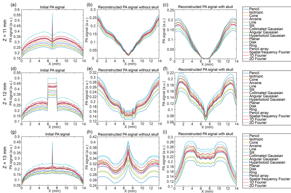
Figure 7. PA signals in the X direction at different Z positions under the illumination of sixteen optical source types. In the X direction at z = 11 mm (a–c): (a) initial PA signal, (b) reconstructed PA signal without the skull, and (c) reconstructed PA signal with the skull; in the X direction at z = 12 mm (d–f): (d) initial PA signal, (e) reconstructed PA signal without the skull, and (f) reconstructed PA signal with the skull; in the X direction at z = 13 mm (g–i): (g) initial PA signal, (h) reconstructed PA signal without the skull, and (i) reconstructed PA signal with the skull.
