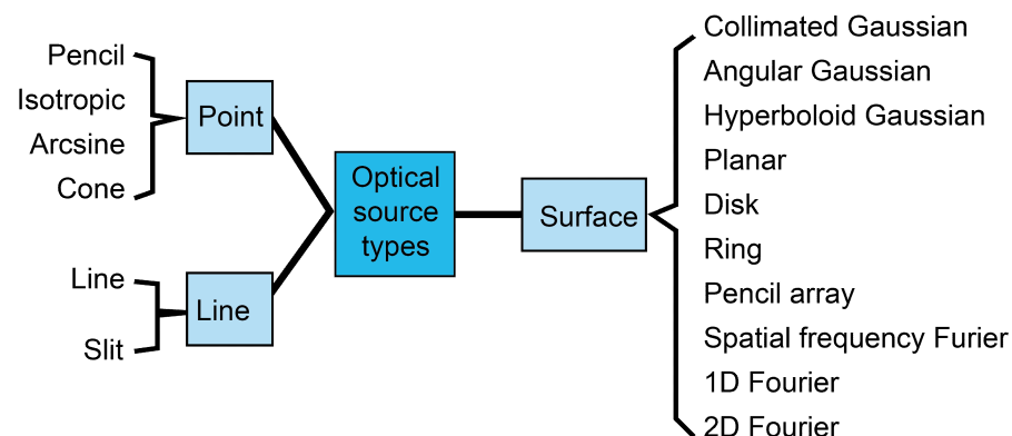
Figure 2. Optical source types into three categories of point, line and surface.
